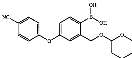
[[4-[4-cyanophenoxy]-2-[(tetrahydro-2H-pyran-2-yl)oxy]methyl]phenyl]boronic acid
