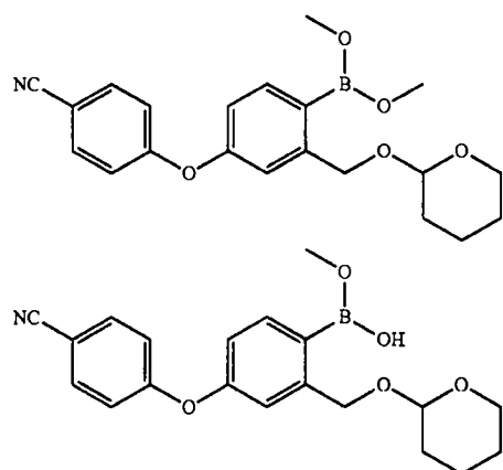
[[4-[4-cyanophenoxy]-2-[(tetrahydro-2H-pyran-2-yl)oxy]methyl]phenyl]boronic acid dimethyl ester
