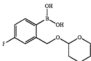
[[4-Fluoro-2-[(tetrahydro-2H-pyran-2-yl)oxy]methyl]phenyl]boronic acid
