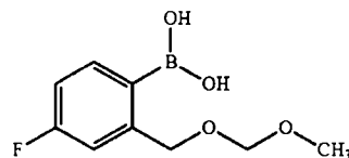
[(4-Fluoro-2-methoxymethoxyethyl)phenyl]boronic acid
