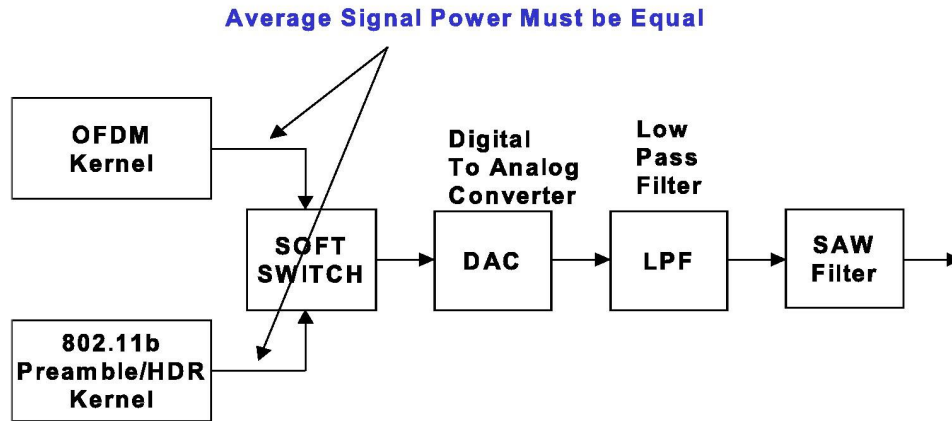
Figure 1530—Comparing signal power
