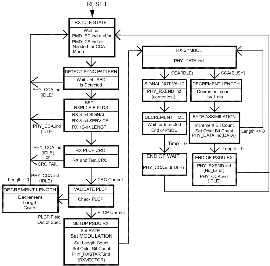
Figure 136—PLCP receive state machine
