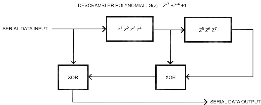
Figure 132—Data descrambler
