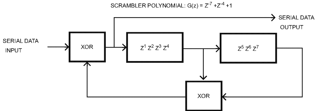
Figure 131—Data scrambler
