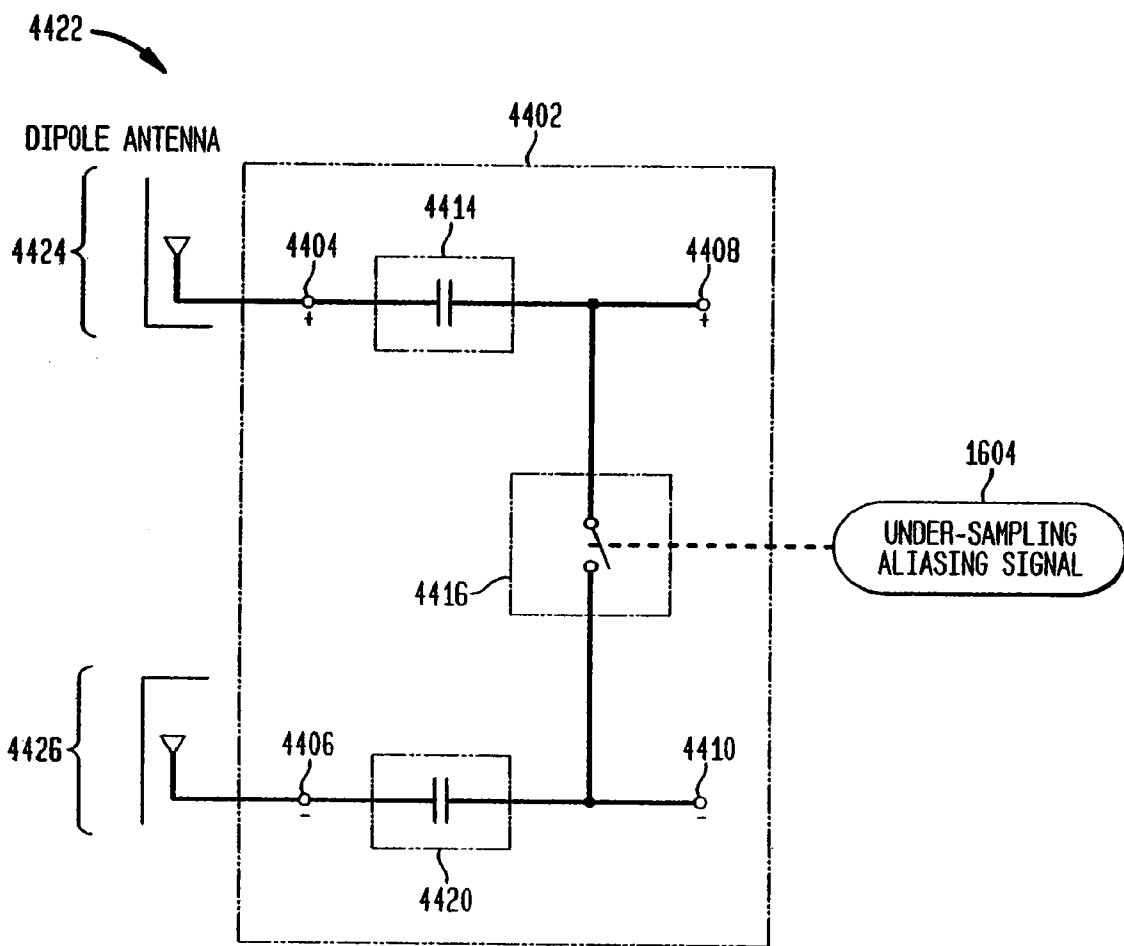
FIG. 44B DIFFERENTIAL INPUT TO DIFFERENTIAL OUTPUT
