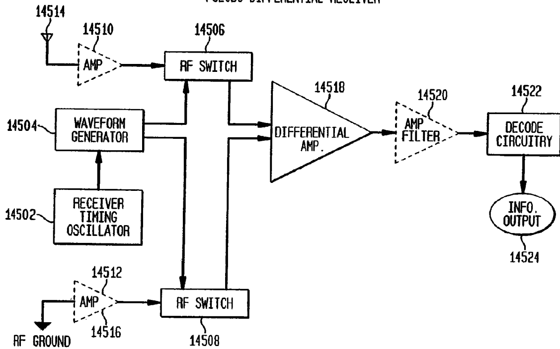
PSEUDO DIFFERENTIAL RECEIVER
