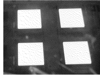
Thin-film encapsulated OLEDs lighting up with minimal luminance change after 1654 hours in damp heat
