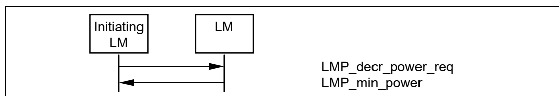
Sequence 44: The TX power cannot be decreased.
