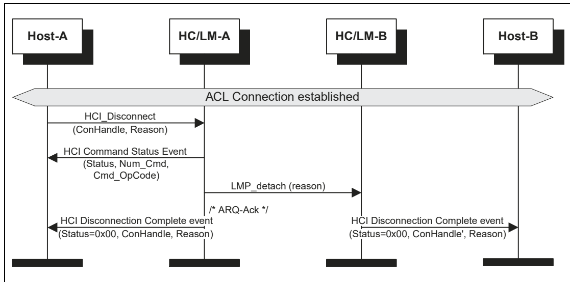
Figure 3.6: ACL Disconnection
