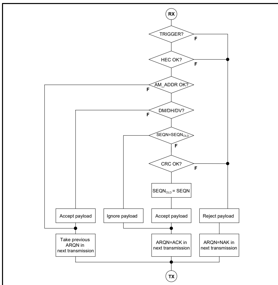
Figure 5.3: Receive protocol for determining the ARQN bit.
