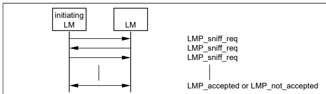
Sequence 31: Negotiation for sniff mode.
