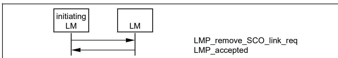
Sequence 53: SCO link removed.
