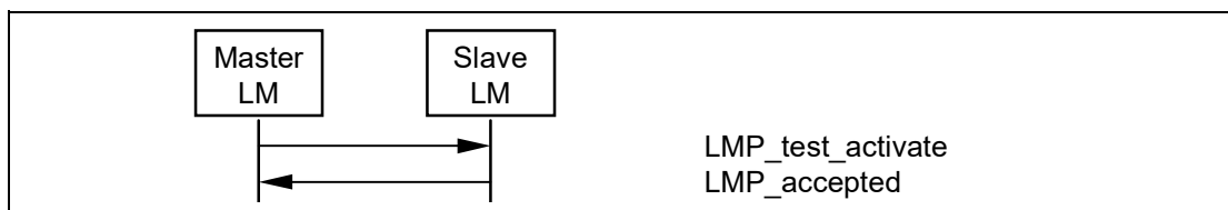
Sequence 60: Activation of test mode successful.
