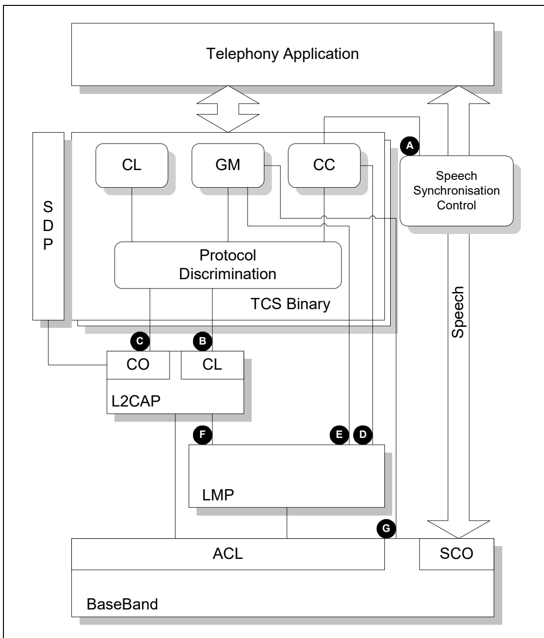
Figure 1.4: TCS Architecture
