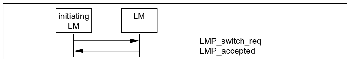
Sequence 23: Master-slave switch accepted.
