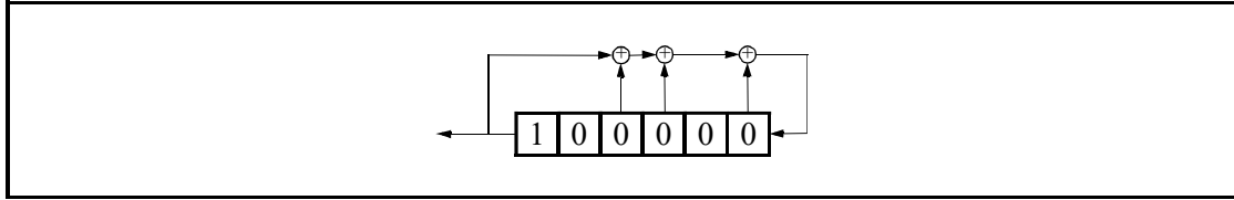
Figure 13.3: LFSR and the starting state to generate p^i(D)
