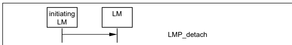
Sequence 26: Connection closed by sending LMP_detach.
