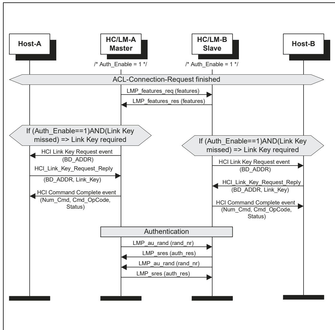
Figure 3.4: ACL Connection setup with authentication
