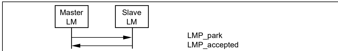
Sequence 33: Slave forced into park mode.
