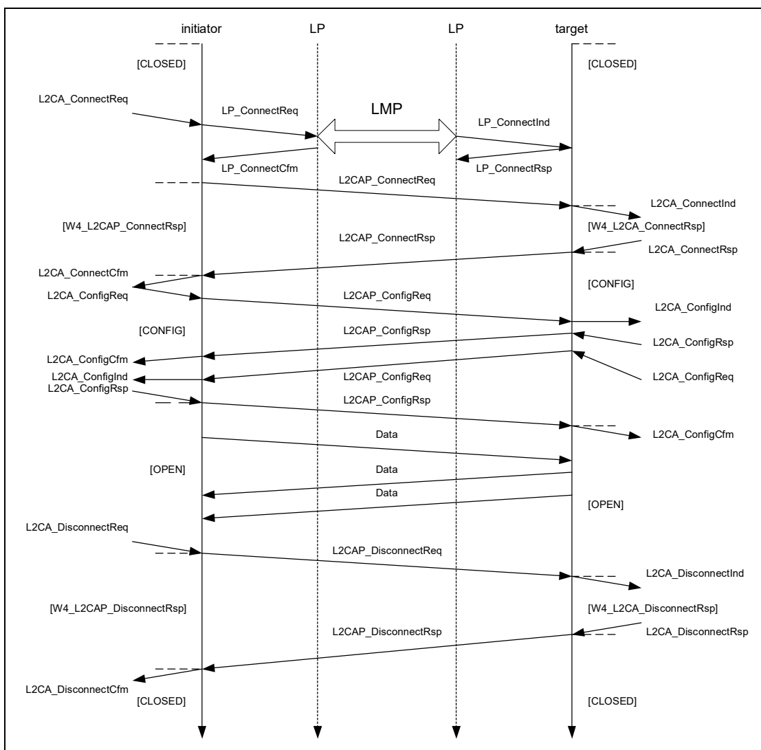
Figure 3.4: Message Sequence Chart of Basic Operation
