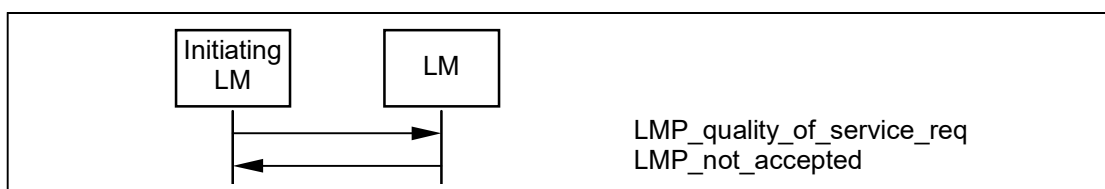
Sequence 49: Device rejects new quality of service.
