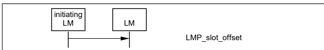
Sequence 18: Slot offset information is sent.
