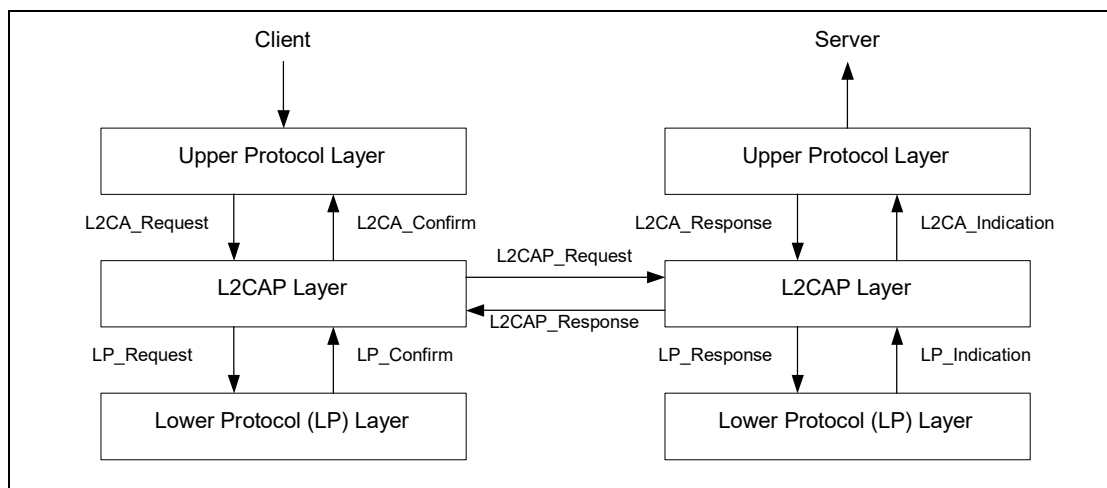
Figure 3.1: L2CAP Layer Interactions
