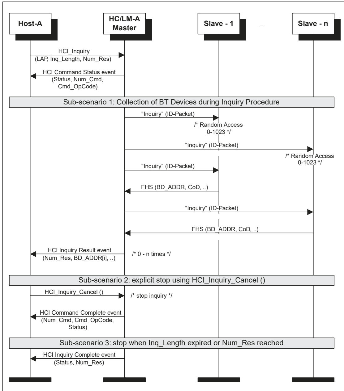
Figure 2.2: One-Time Inquiry
