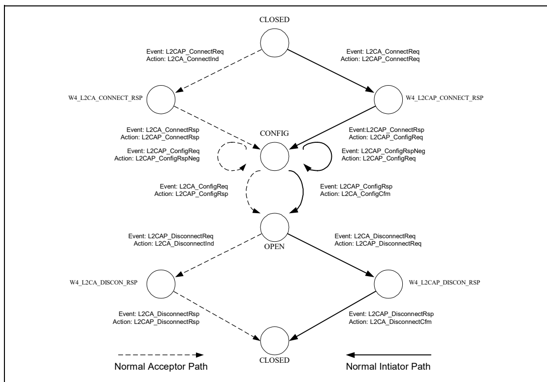
Figure 3.3: State Machine Example
