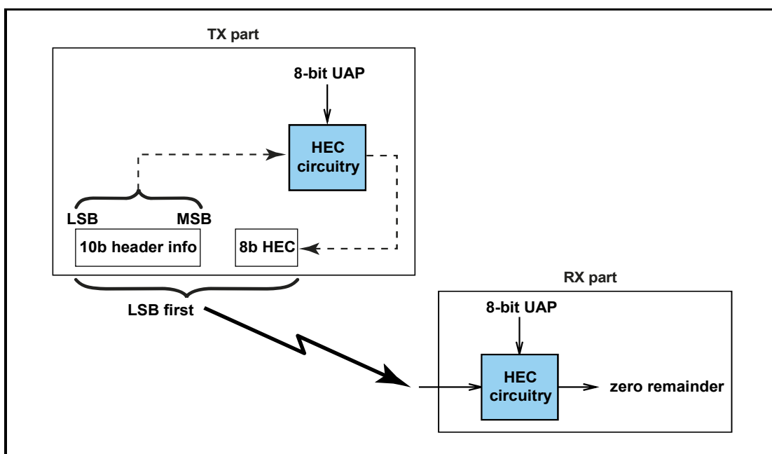
Figure 5.8: HEC generation and checking.
