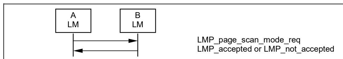
Sequence 58: Negotiation for page scan mode
