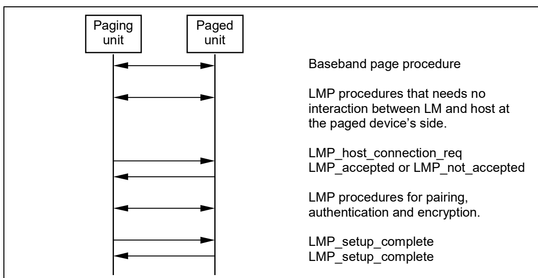
Figure 4.1: Connection establishment.
