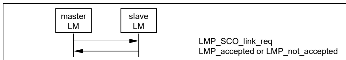
Sequence 50: Master requests an SCO link.
