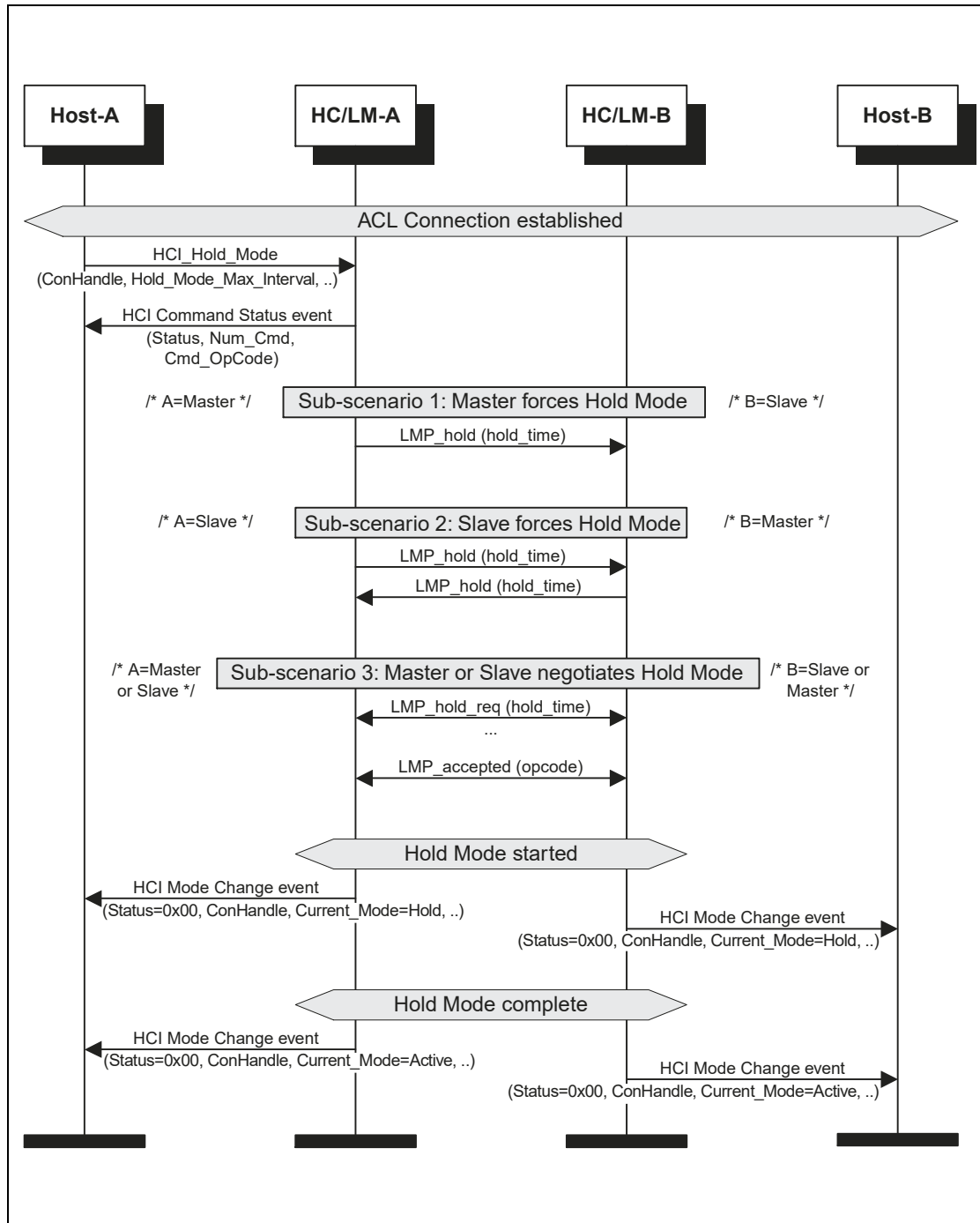
Figure 6.2: Hold Mode
