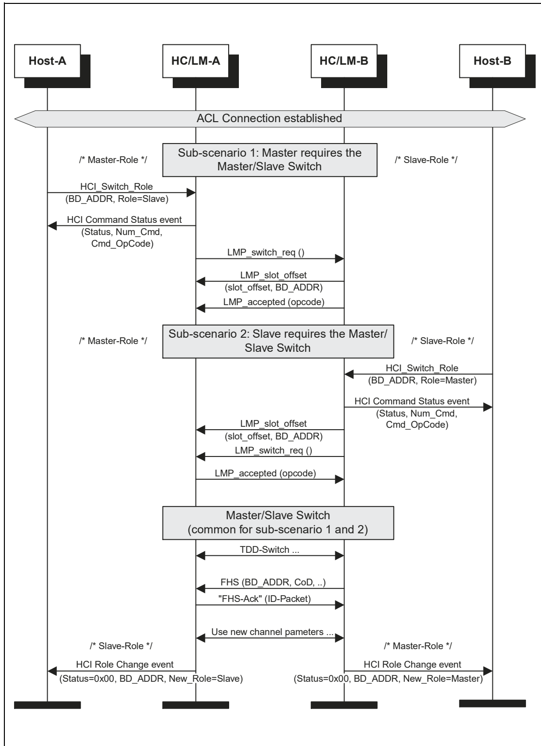
Figure 4.9: Switch Role
