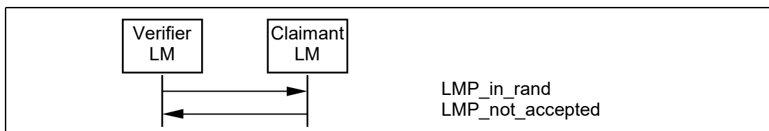
Sequence 6: Claimant rejects pairing.
