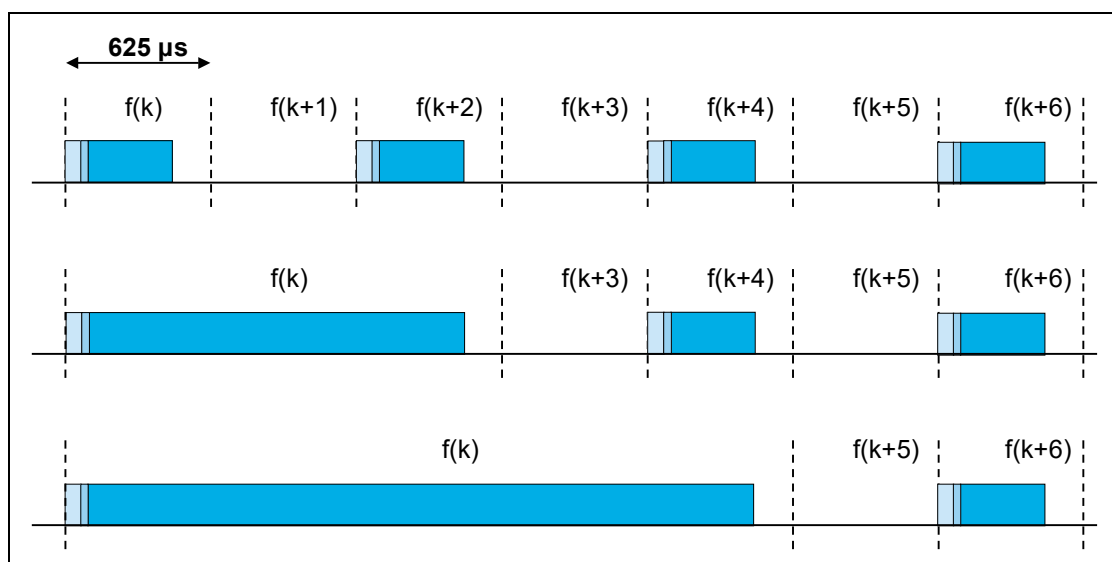
Figure 2.2: Multi-slot packets
