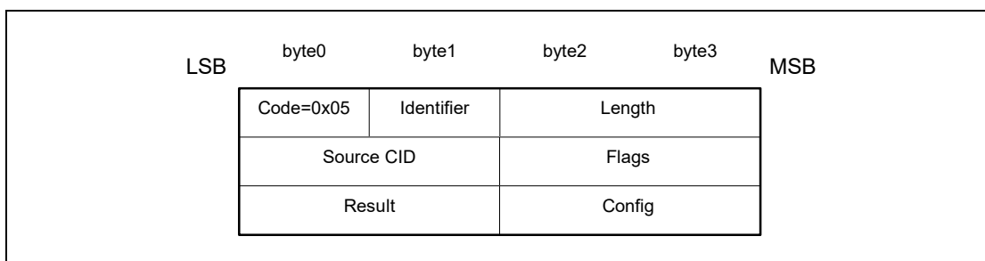
Figure 5.8: Configuration Response Packet
