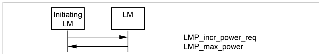
Sequence 43: The TX power cannot be increased.
