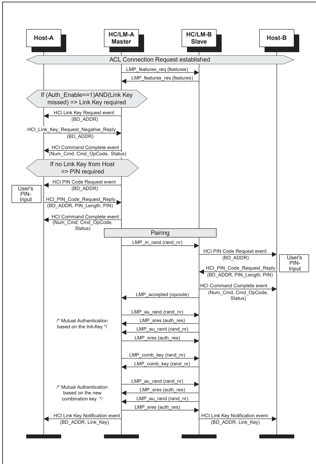
Figure 3.3: ACL Connection setup with pairing
