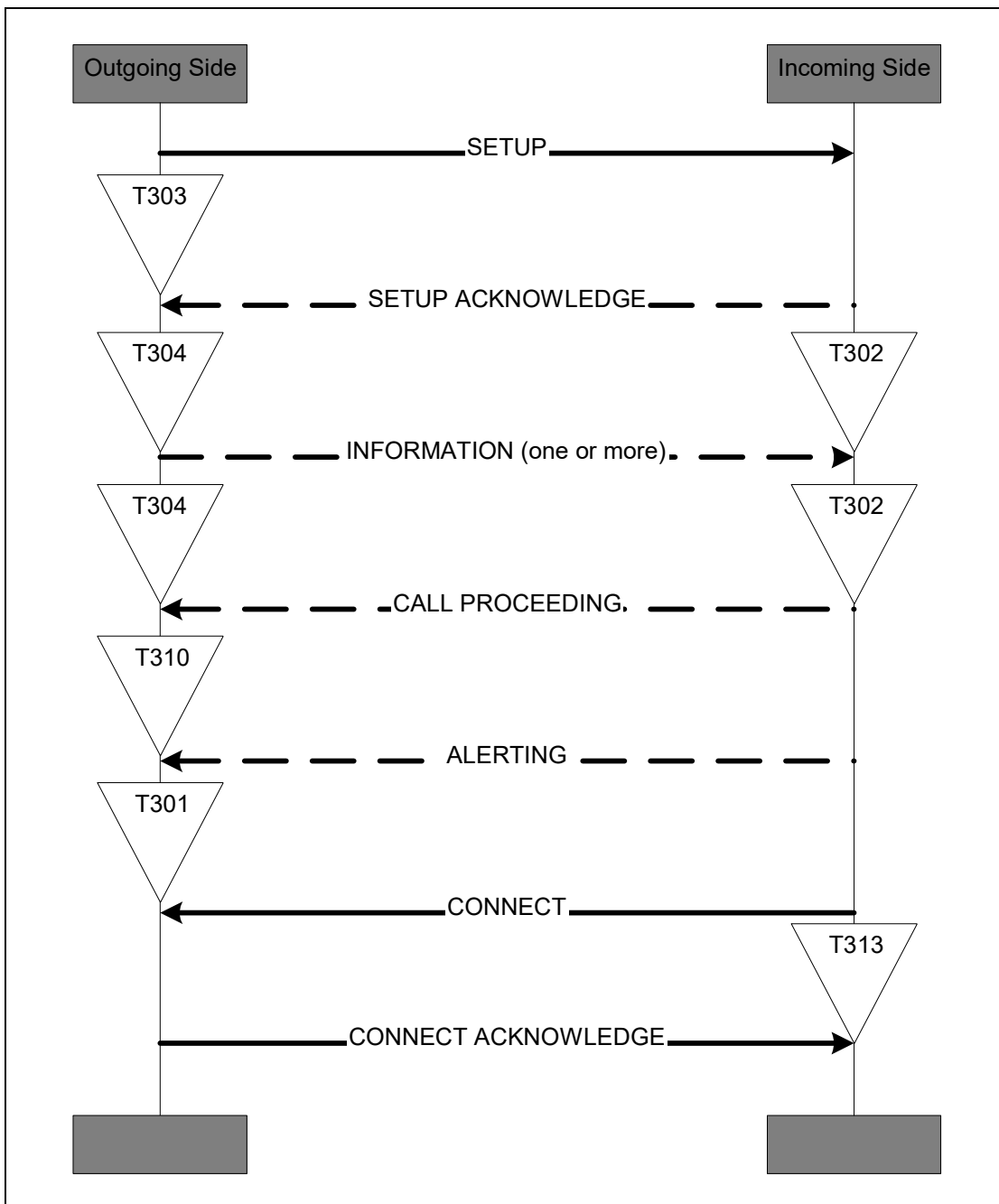
Figure 2.1: Call establishment message flow
