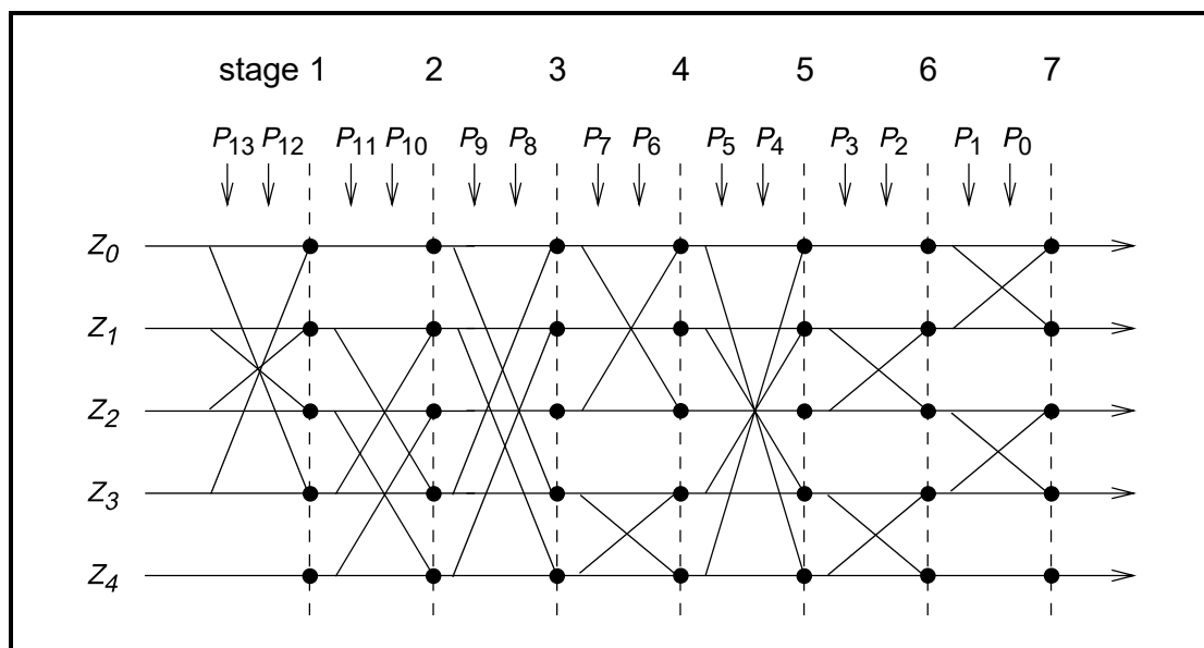
Figure 11.6: Permutation operation for the 79 hop system.
