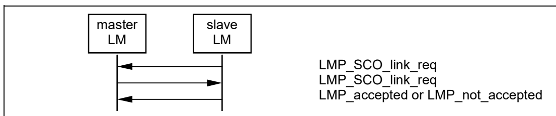
Sequence 52: Master accepts slave's request for an SCO link.
