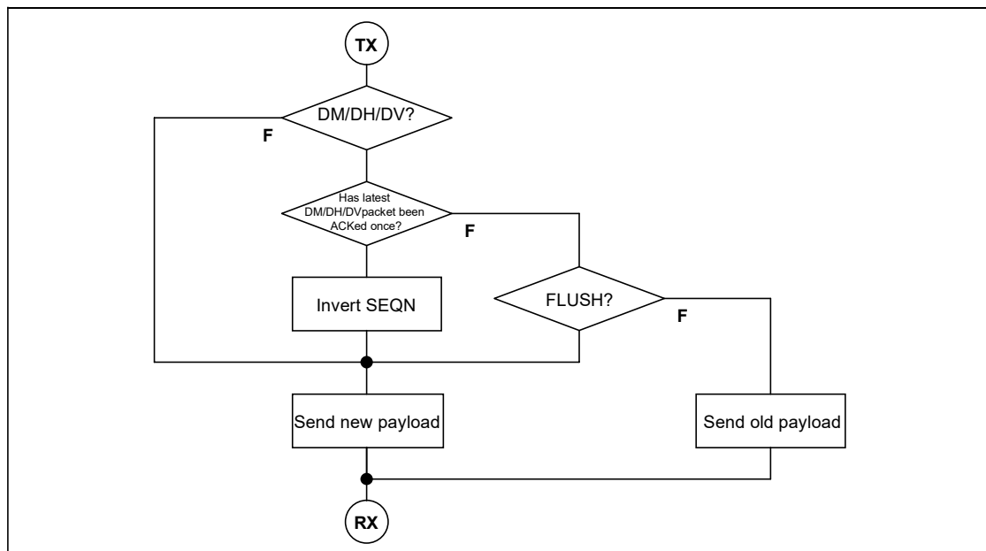
Figure 5.4: Retransmit filtering for packets with CRC.
