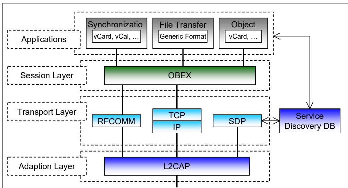
Figure 1.1: Part of Bluetooth Protocol Hierarchy
