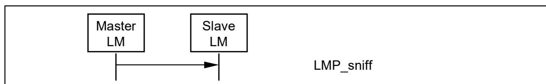
Sequence 30: Master forces slave into sniff mode.
