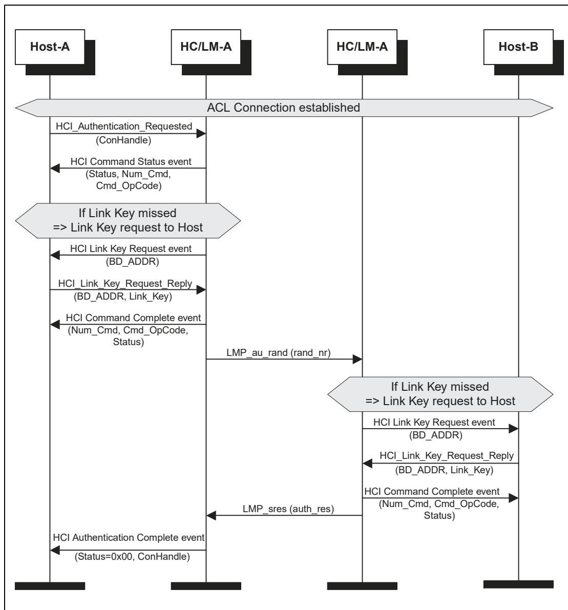
Figure 4.1: Authentication Requested
