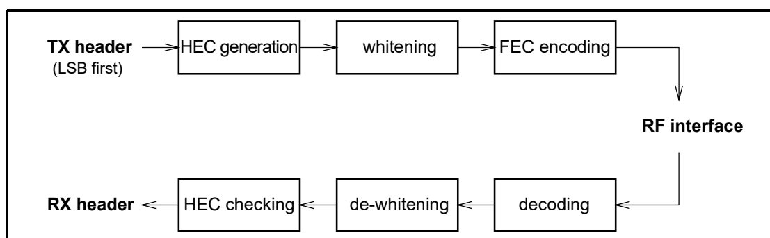
Figure 8.3: Header bit processes.
