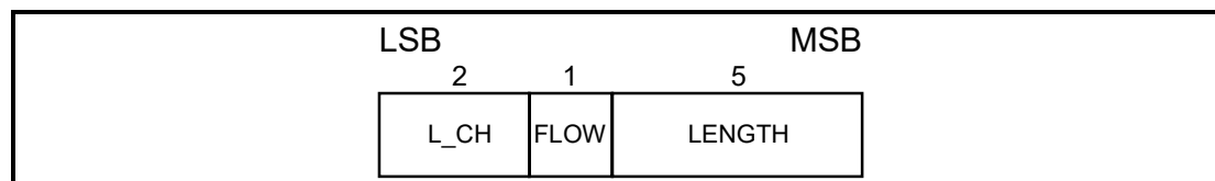
Figure 4.8: Payload header format for single-slot packets.
