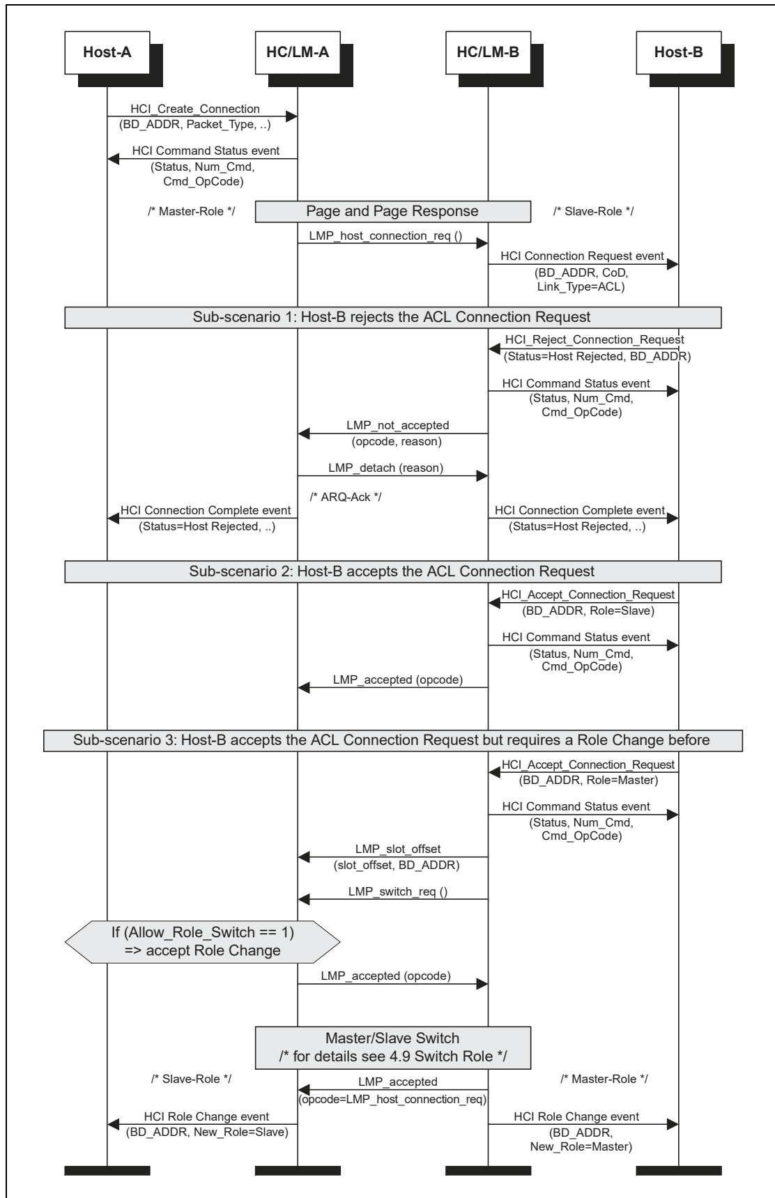
Figure 3.2: ACL Connection Request phase
