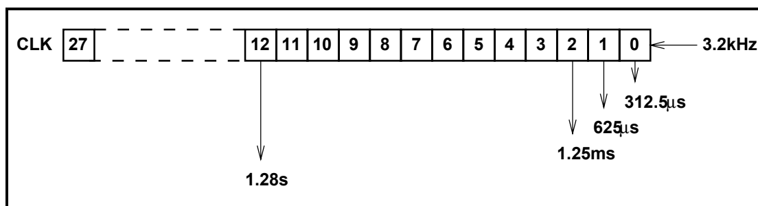
Figure 10.1: Bluetooth clock.
