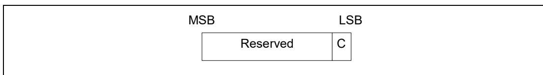
Figure 5.9: Configuration Response Flags field format
