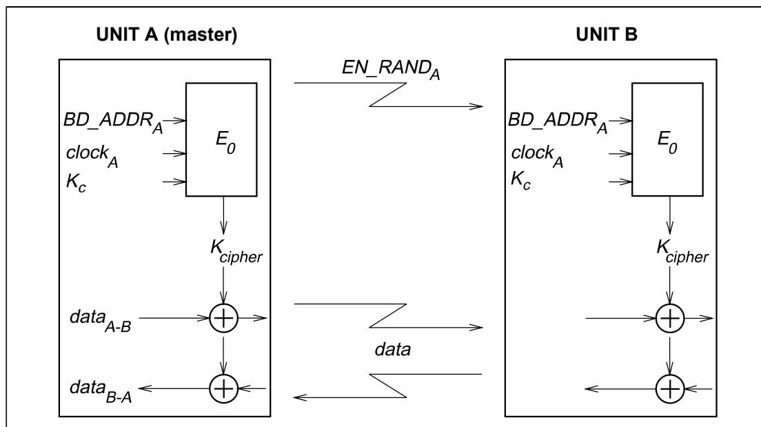
Figure 14.5: Functional description of the encryption procedure
