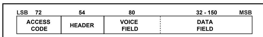
Figure 4.7: DV packet format
