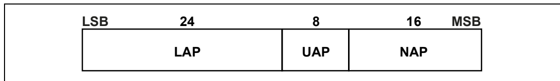
Figure 13.1: Format of BD_ADDR
