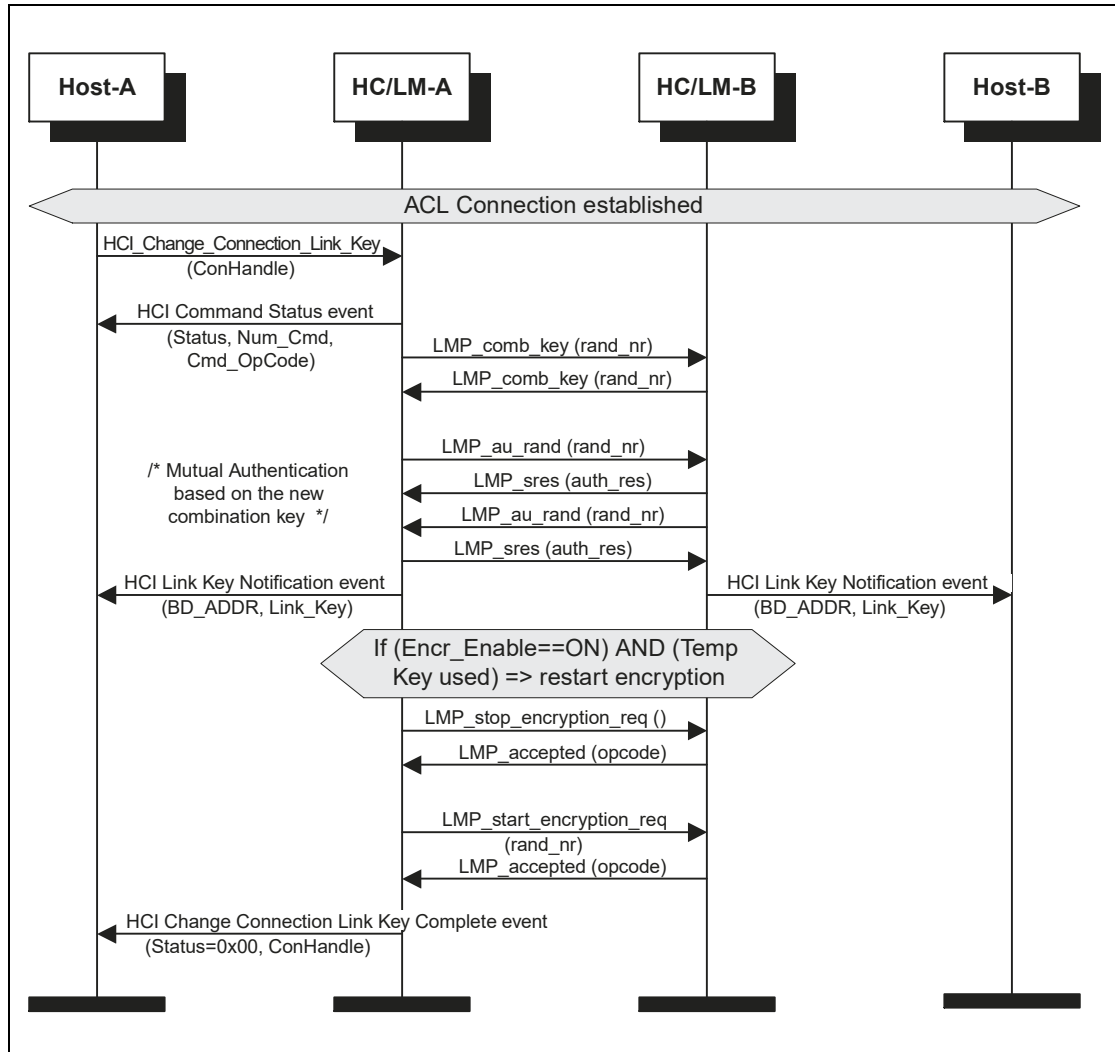
Figure 4.3: Change Connection Link Key
