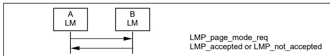
Sequence 57: Negotiation for page mode.
