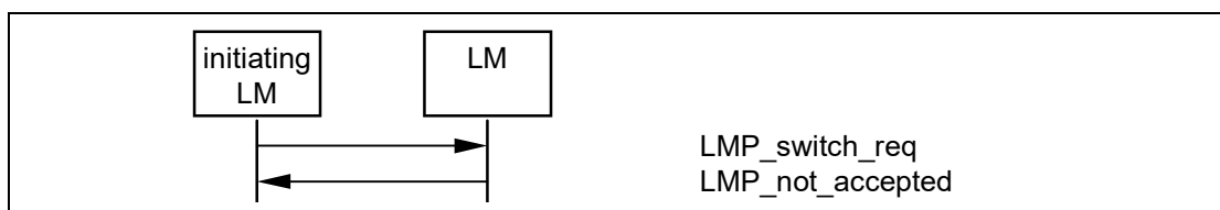
Sequence 24: Master-slave switch not accepted.
