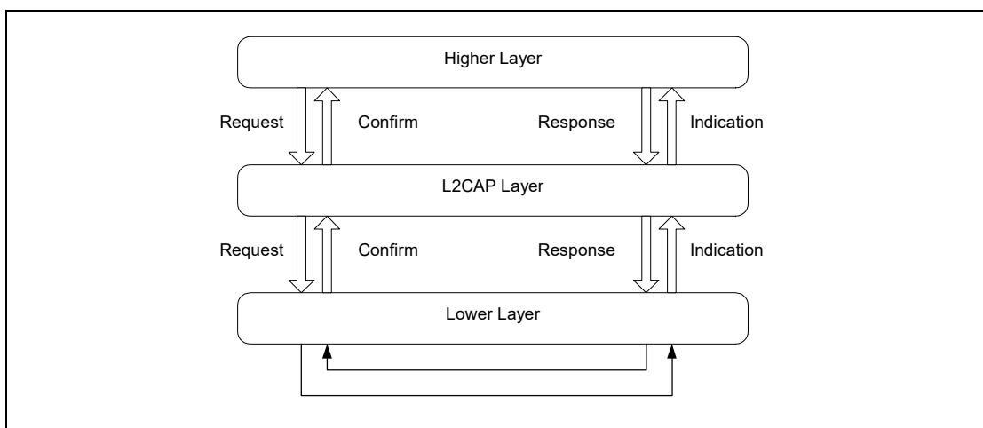
Figure 2.2: L2CAP Architecture
