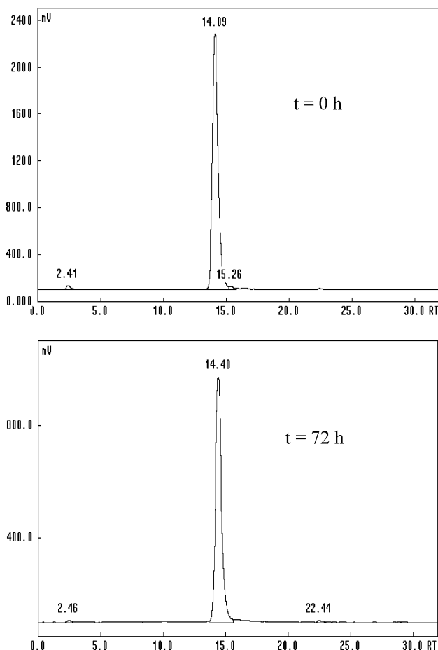
Figure 3. Radio-HPLC chromatograms of ^{90}\text{Y} -TA138 at -78 °C.
