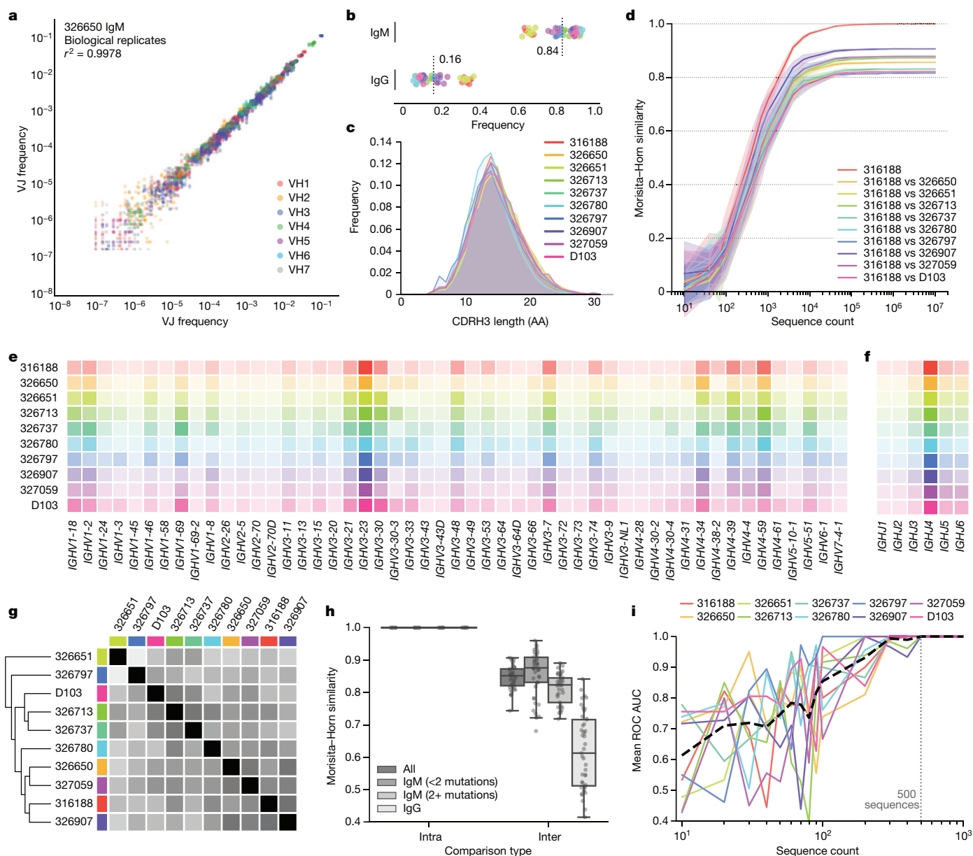
Fig. 1 | Uniqueness of the repertoires of individual subjects. a , Frequency comparison of V and J combinations in biological replicates from subject 326650. V and J combinations are coloured according to the V gene used. b , Sequence frequency by antibody isotype. Subjects are coloured as in c . Each point represents a single biological replicate. Mean of all samples is indicated for each isotype. c , CDRH3 length distribution for each subject. CDRH3 lengths were determined using the Immunogenetics (IMGT) numbering scheme. AA, amino acids. d , Morisita–Horn similarity of pairwise comparisons between subject 316188 and each of the other subjects. Lines indicate mean similarity of 20 bootstrap samplings, and shaded areas indicate 95% confidence intervals. Data from subject 316188 are representative; plots for all other subjects can be found in Extended Data Fig. 4. e , f , V gene ( e ) and J gene ( f ) use by subject. Increased colour intensity indicates higher frequency. Subjects are coloured as in c . g , Clustered distance matrix of subjects,
