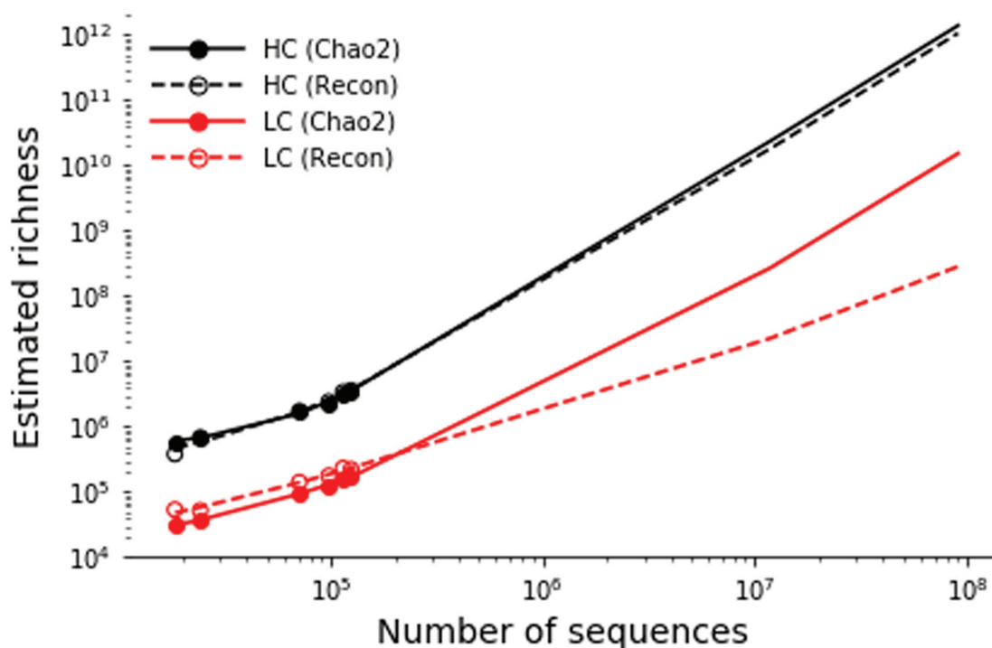
Extended Data Fig. 7 | Relative light-chain diversity estimation. Using previously reported datasets of paired heavy and light antibody chains, clonotype diversity was estimated for heavy and light chains using both Chao 2 and Recon estimators. Estimates are shown in filled or unfilled
