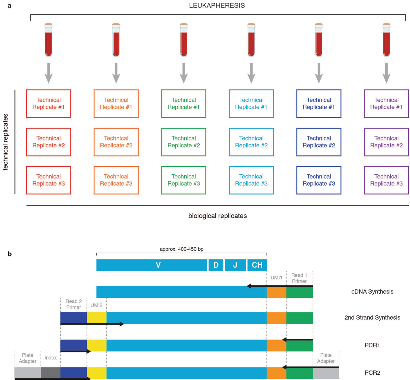
Extended Data Fig. 1 | Nearly full-length antibody gene amplification from biological and technical replicate samples. a , Schematic of biological and technical replicate samples. Biological replicates (columns) are derived from distinct cell aliquots, so identical clonotypes or sequences found in multiple biological replicates must arise from different cells. Technical replicates (rows) were amplified using discrete RNA aliquots from a single-cell aliquot. b , Strategy for nearly full-length antibody heavy
