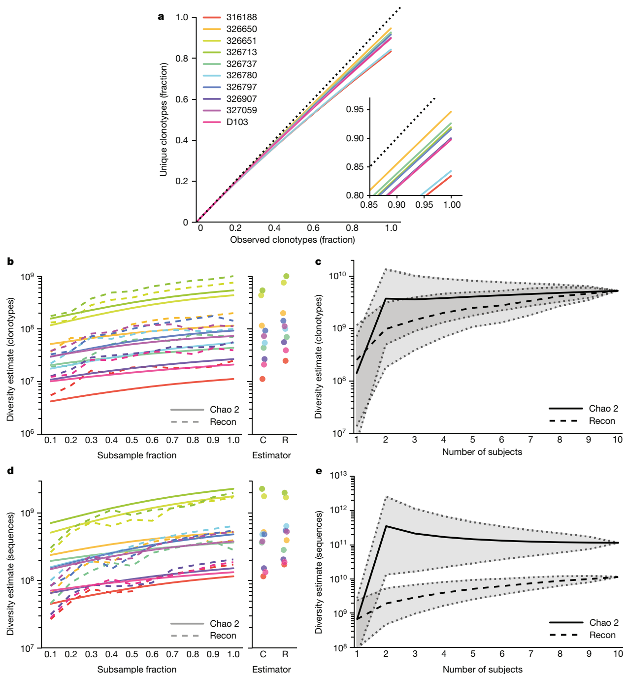
Fig. 2 | Clonotype and sequence diversity amongst the 10 subjects.
