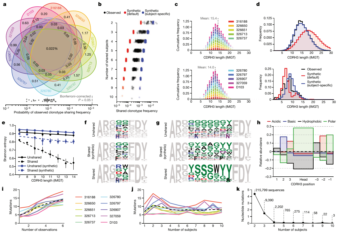
Fig. 3 | Shared clonotypes and sequences amongst the 10 subjects. a , Venn diagram of shared clonotype frequency. b , Shared clonotype frequency between subject groups. Points represent different group combinations. Observed sequences (black), synthetic sequences generated with IGoR's default model (red) and sequences generated with subject-specific models (blue) are shown. c , Distribution of CDRH3 lengths for clonotypes found in one biological replicate (top) or all six biological replicates (bottom). CDRH3 length is defined using IMGT numbering. The colour key legend is split to maintain legibility; data for all subjects are present in both plots. d , Distribution of CDRH3 length for unshared clonotypes (top) or clonotypes shared by the majority of subjects (bottom). Observed sequences (black), default model (red) and subject-specific model (blue) synthetic sequences are shown. e , Per position Shannon entropy of the CDRH3 head regions of unshared (solid) or majority-shared (dashed) clonotypes. Points indicate the mean, whiskers indicate the 95% confidence interval, and lines represent the linear best fit.
