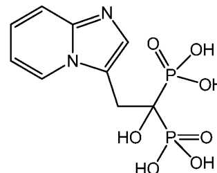
minodronic acid
