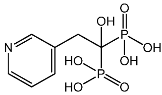
risedronic acid
