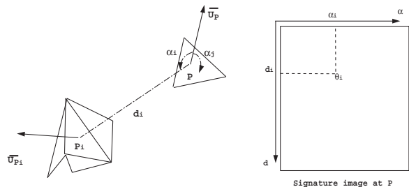
Fig. 2. For each point P we generate a signature image where the image axis are the distance d between P and each other point on the surface and the angle \alpha between the normal at P , \vec{U}_P and the vector from P to each other point. The image encodes the simplex angle \theta .
