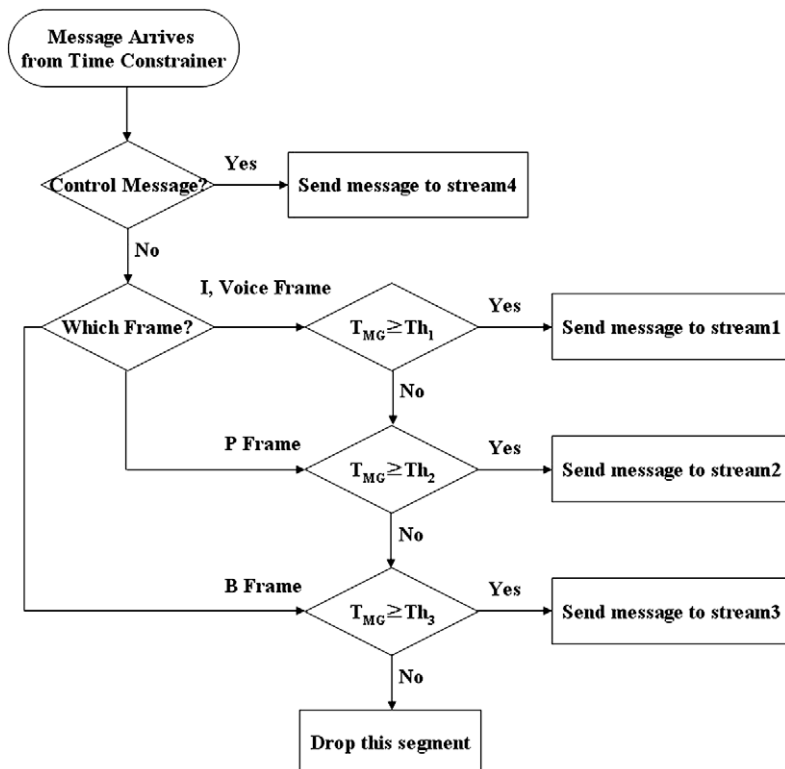
Fig. 5. TCSL data transmission algorithm.
