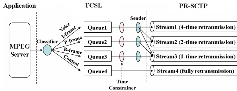
Fig. 2. Differentiated transmission according to data type.
