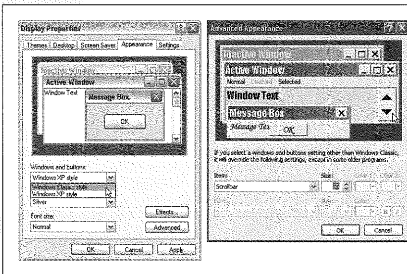
Figure 8-11: Left: For the full arsenal of design-scheme controls, choose "Windows Classic style," as shown here, before clicking the Advanced button.
