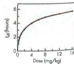
Figure 19-6. Plot of t_{\text{eff}} versus dose.
