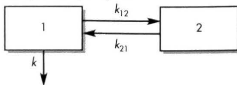
MODEL 3. Two-compartment open model, IV injection.
