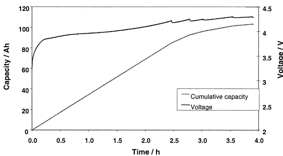
Fig. 5. Capacity and voltage vs time.
