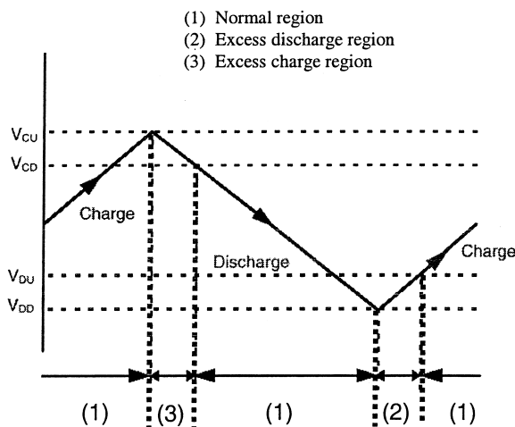
Fig. 9. Mode of operation of protection board.
