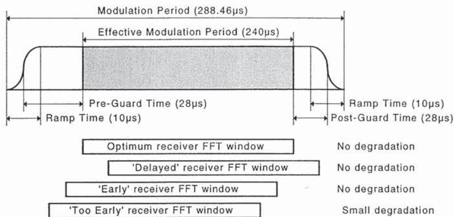
Figure 9.9 OFMDA burst and synchronization requirements.
