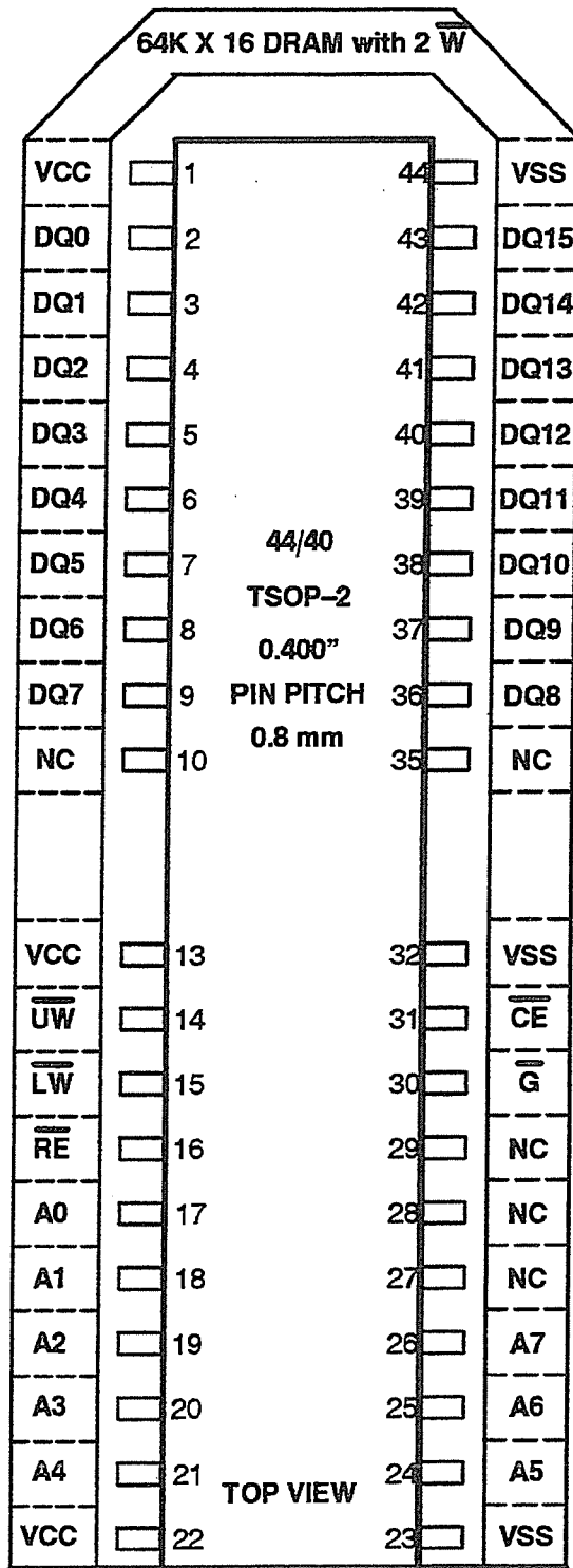
FIGURE 3.9.4-6 64K BY 16 DRAM WITH 2 W IN TSOP-2
