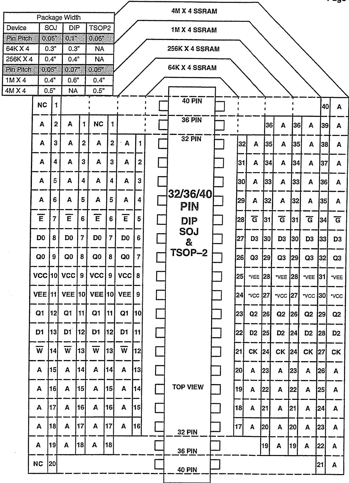
FIGURE 3.7.4-8 64K TO 4M BY 4 ECL SSRAM FAMILY IN DIP, SOJ, AND TSOP-2
