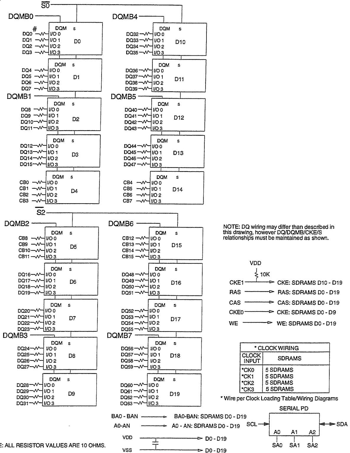
Figure 4.5.4-U X8 SDRAM DIMM, 1 Bank with X4 SDRAMs
