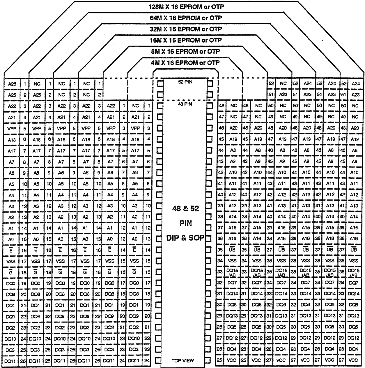
FIGURE 3.4.2-5 4M TO 128M BY 16 EPROM & OTP IN DIP AND SOP
