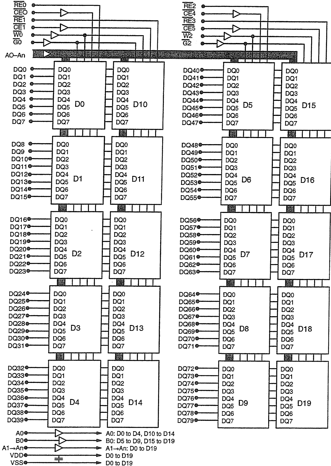
Figure 4.5.1-Y 168 PIN, X80 (ECC mode) DRAM DIMM, 2 banks with X8 DRAMs Release 4-7
