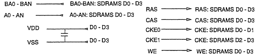
Figure 4.5.6-L 144 Pin X64 SDRAM SO-DIMM, 2 Bank with X32 SDRAMs
