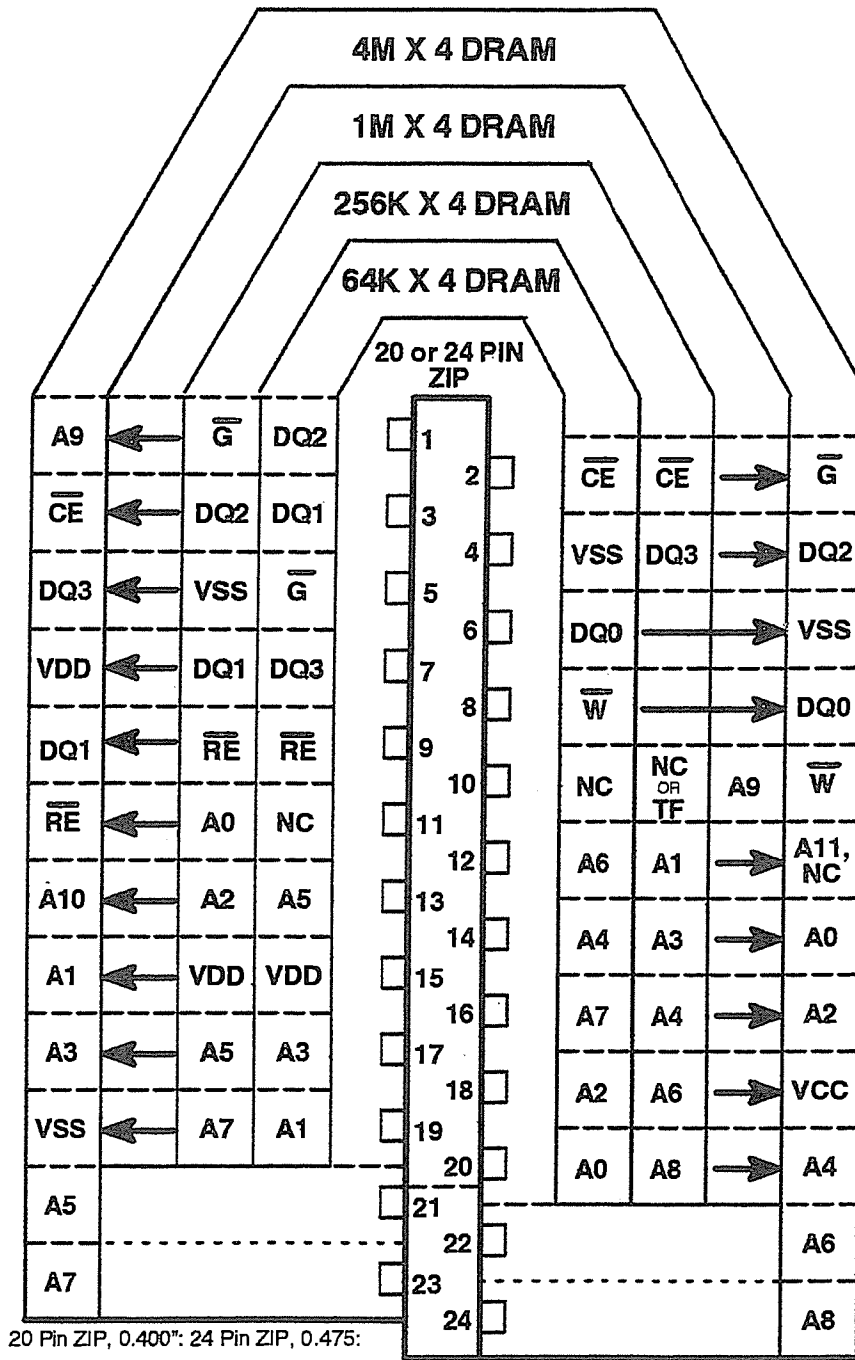
TOP VIEW
