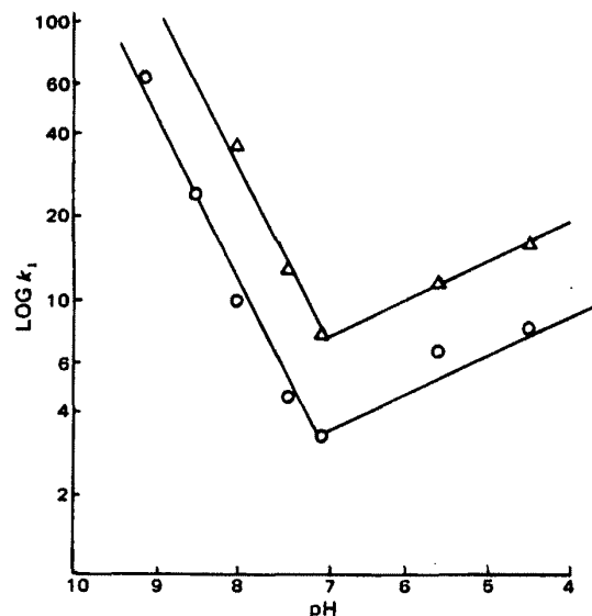
Figure 8 —The pH stability profile of 5-azacytidine ( 8.2 \times 10^{-4} M ) in aqueous buffers (potassium phosphate buffer, 0.067 M) at 25° (○) and 37° (Δ).
