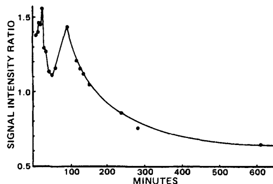
Figure 6—Kinetic profiles of 90% enriched 6- 13 C-5-azacytidine (0.158 M) hydrolysis in pH 8.0, 0.067 M potassium phosphate buffer containing 30% deuterium oxide and 13 C-sodium acetate (0.20 M) at 27° using 13 C-NMR measurements. Vertical axis is signal intensity ratios between 5-azacytidine and sodium acetate.
