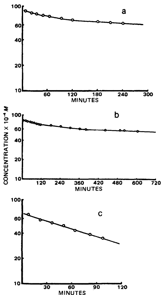
Figure 7 —Kinetic profiles of 5-azacytidine ( 8.2 \times 10^{-4} M ) hydrolysis in potassium phosphate buffers using HPLC measurements. Key: (a), pH 5.6 and 2.5°; (b), pH 7.0 and 25°; and (c), pH 9.1 and 25°.
