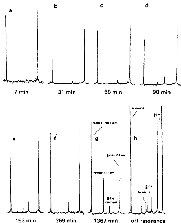
Figure 5— 13 C-NMR spectrum of 90% enriched 6- 13 C-5-azacytidine (0.148 M) in pH 8.0, 0.067 M potassium phosphate buffer containing 30% deuterium oxide and 13 C-sodium acetate (0.20 M) at 27°. Figures 5a–5h are spectra at selected times. For complete number of time points, see Fig. 6.
