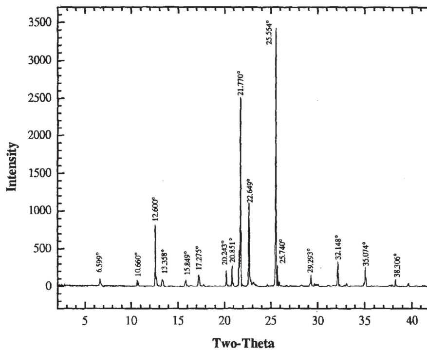
Figure 8 X-ray Powder Diffraction Pattern of Azacitidine, Form VIII, Labeled with the more Prominent 2\theta Angles (Cu K\alpha Radiation)
