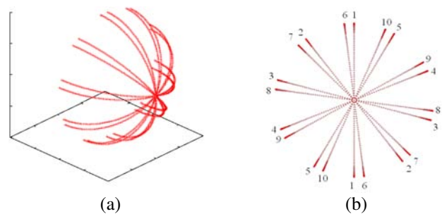
Fig. 8. Change of measurement points with the sensor rotating fast: (a) Bird view, (b) View from x-axis
