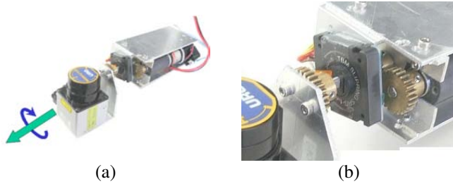
Fig. 6. Rotating device : (a) overall view, (b) slip ring
