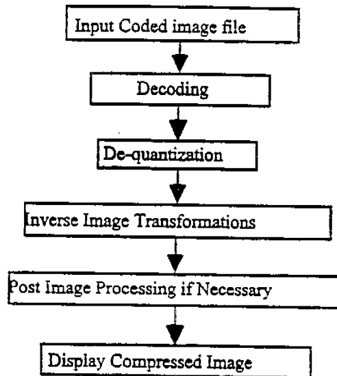
Figure 2: Image decompression
