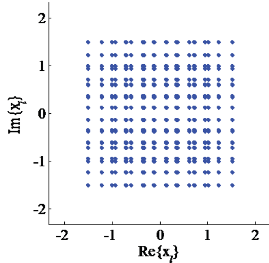
Figure 6.13 Example 1024-NUC for code rate 6/15.
