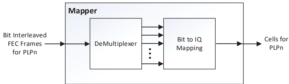
Figure 6.10 Mapper structure.
