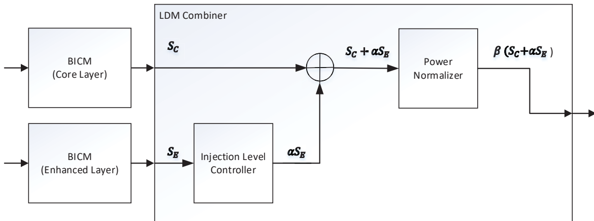
Figure 6.15 Constellation superposition for two-layer LDM.
