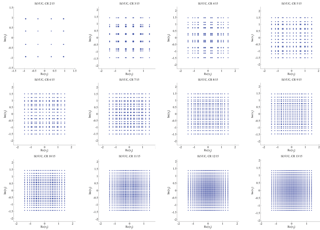
Figure C.2.5 Constellations of 1024QAM.
