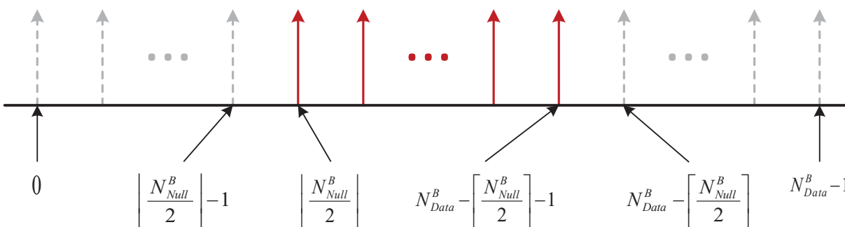
Figure 7.14 Data carrier indices for null and active data carriers.
