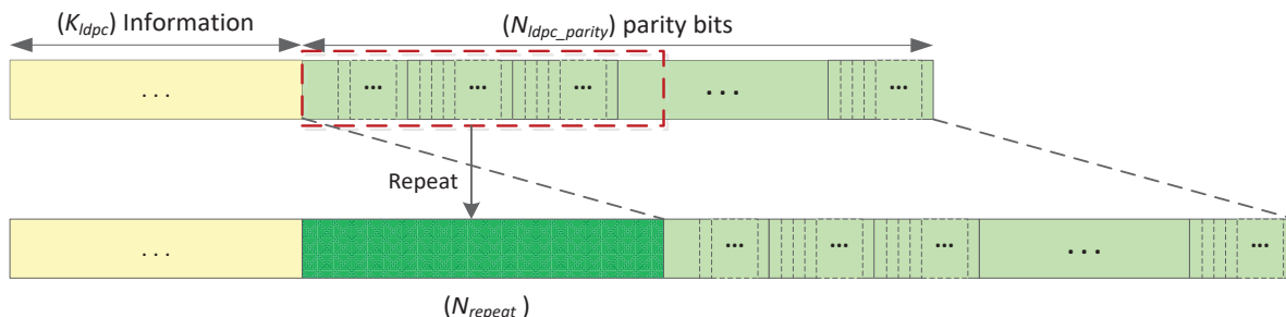
Figure 6.22 Parity Repetition ( N_{repeat} \leq N_{ldpc\_parity} ).
