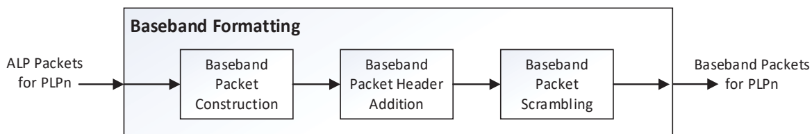
Figure 5.2 Block diagram of baseband formatting.
