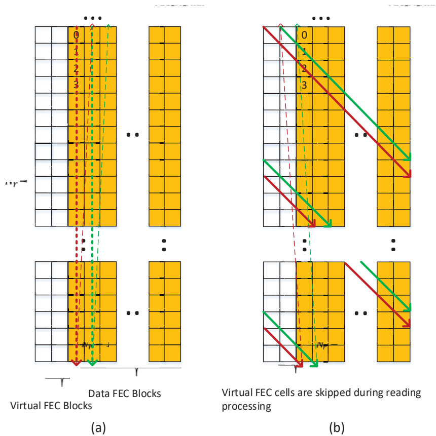
Figure 7.7 Block diagram of Twisted Block Interleaver: (a) linear writing operation, (b) diagonal-wise reading operation.
