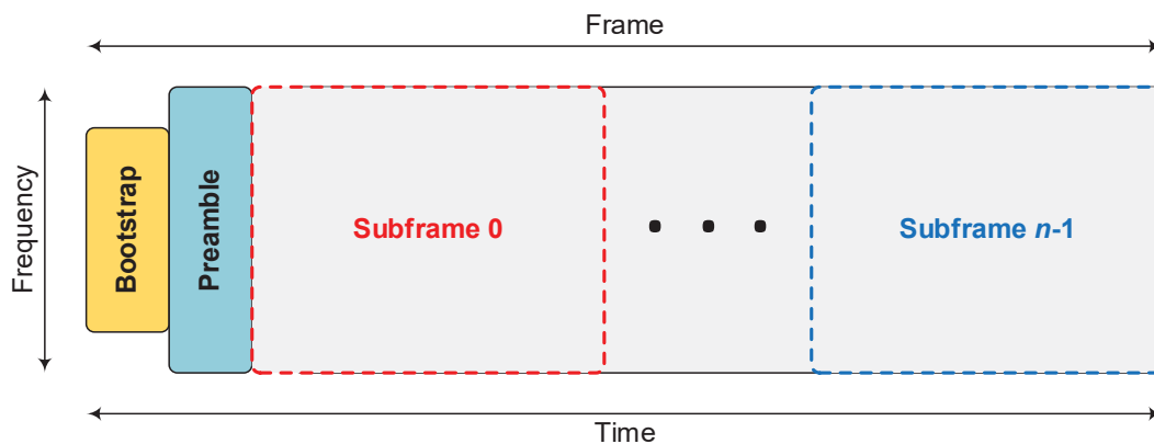
Figure 7.10 Frame structure.
