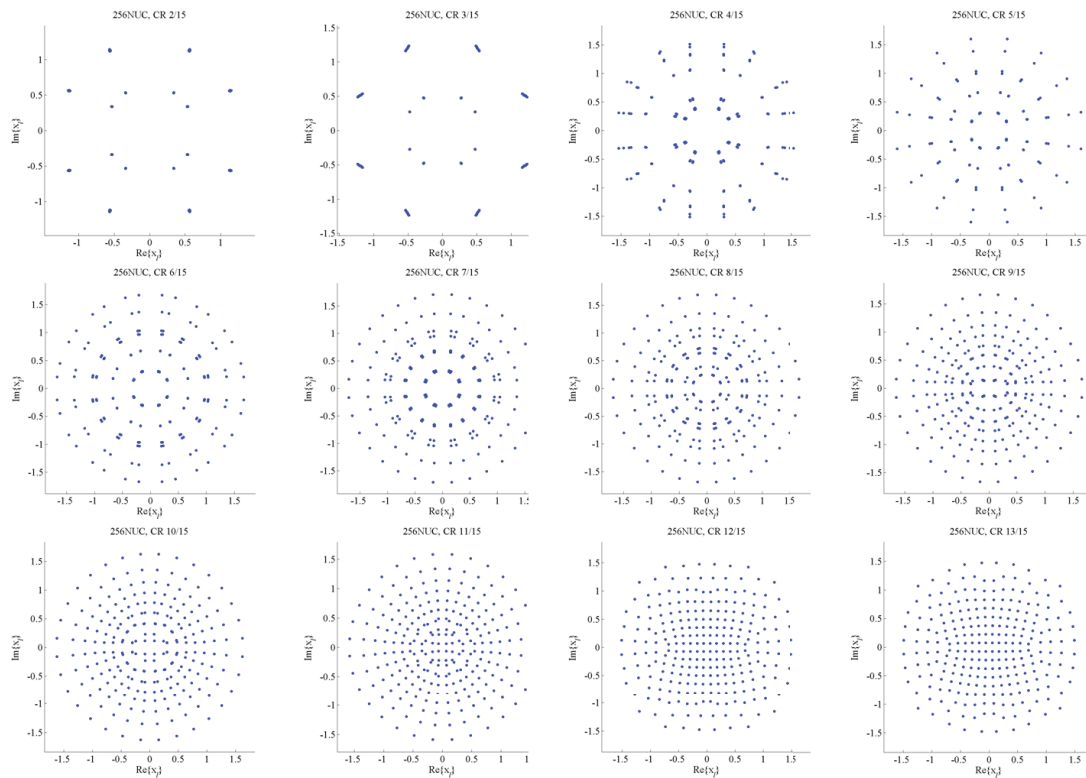
Figure C.2.4 Constellations of 256QAM.
