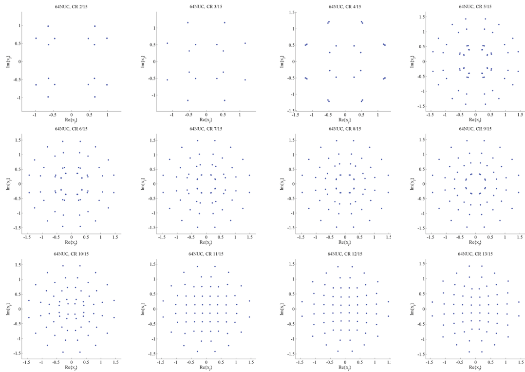
Figure C.2.3 Constellations of 64QAM.
