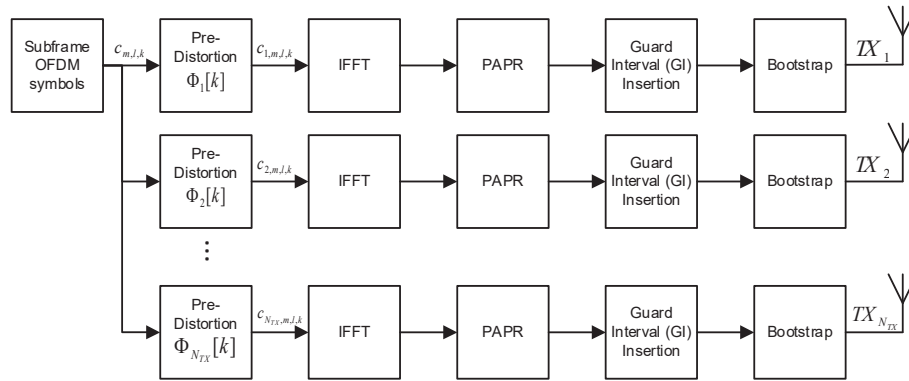
Figure 8.3 Block diagram showing example MISO transmission.
