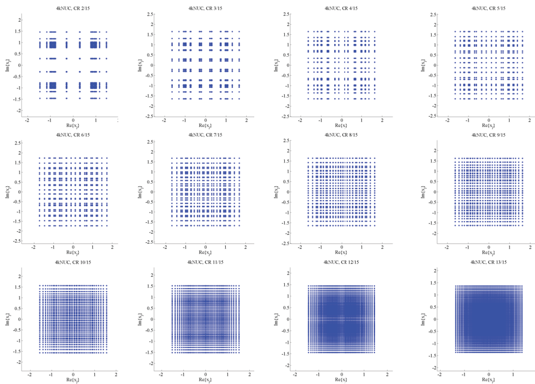
Figure C.2.6 Constellations of 4096QAM.
