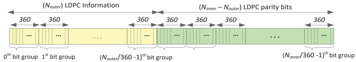
Figure 6.6 Parity interleaved LDPC codeword bit groups.
