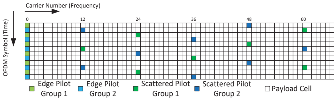
Figure L.9.22 MIMO pilot scheme MP12_4 for null pilot encoding.
