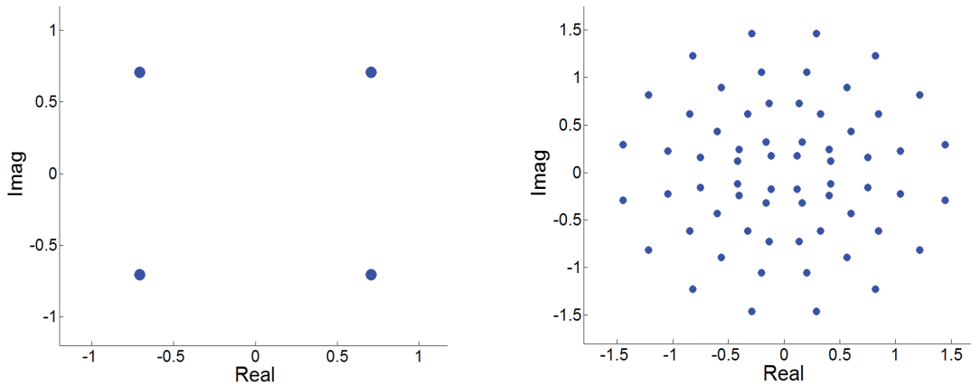
Figure 6.16 Examples of (a, left) Core Layer and (b, right) Enhanced Layer constellations.
