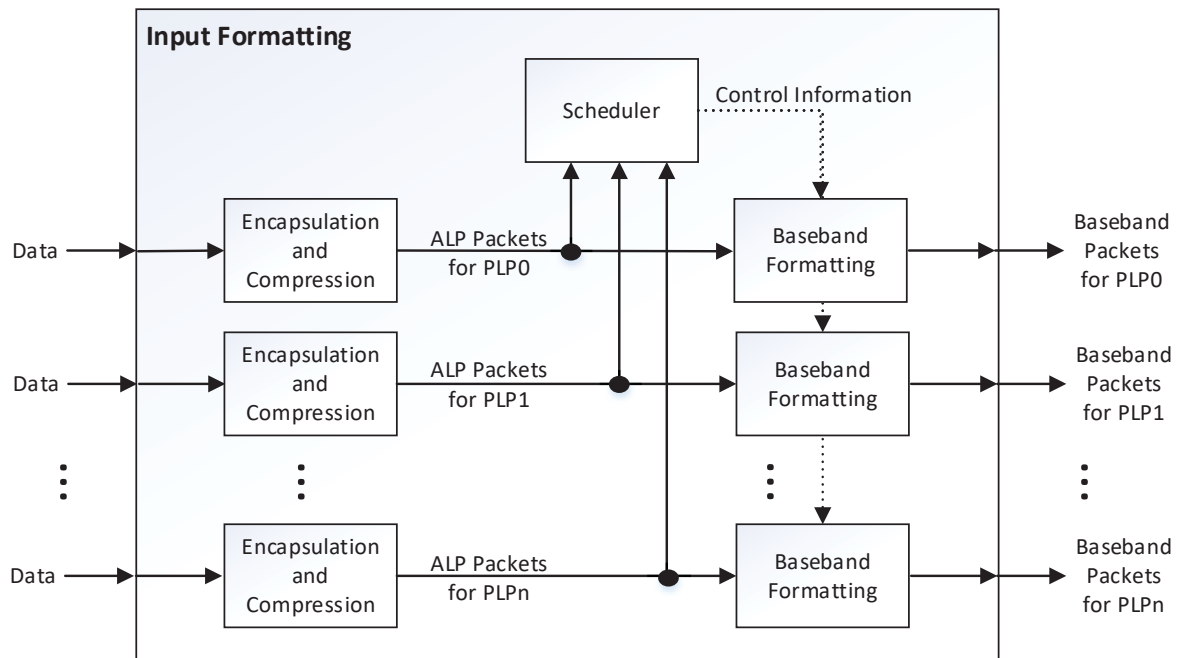
Figure 5.1 Block diagram of input formatting.
