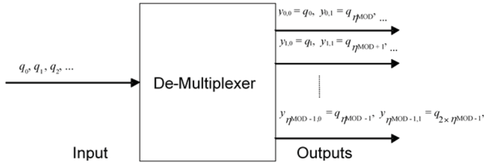
Figure 6.11 De-multiplexing of bits into sub-streams.
