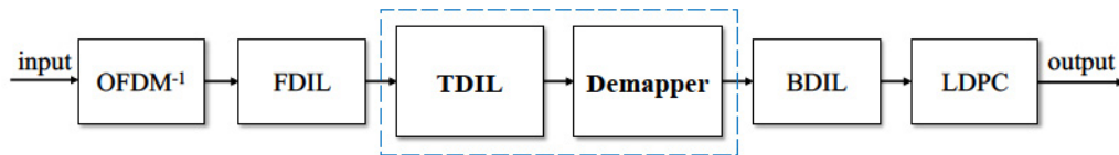
Figure 4.1: General receiver architecture. Time de-interleaving and demapping blocks are explored in this chapter.
