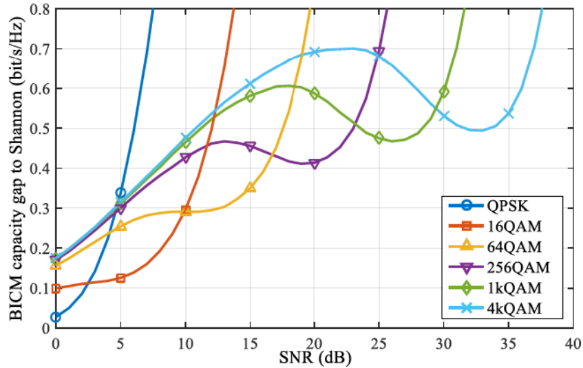
Figure 2.9: BICM capacity shortfall of uniform QAM constellations from the Shannon theoretical limit, AWGN channel.
