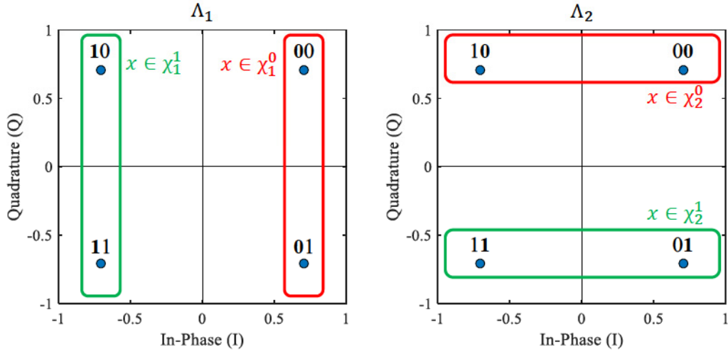
Figure 2.10: Complementary sets of transmitted symbols to compute \Lambda_1 and \Lambda_2 , using a QPSK constellation.
