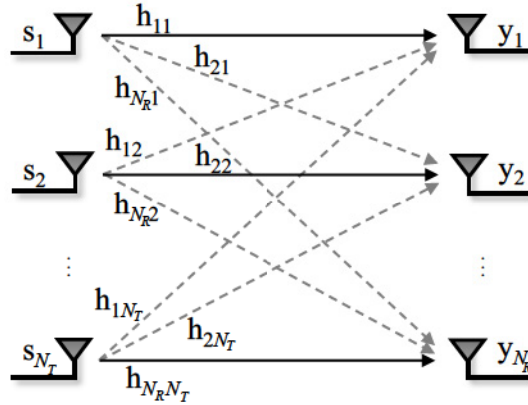
Figure 2.3: N_T \times N_R MIMO channel diagram.
