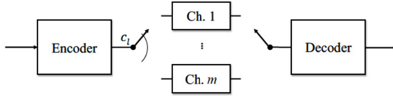
Figure 2.5: Parallel channel model for a BICM transmission.
