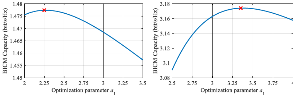
Figure 3.1: BICM capacity values obtained for different parameters a_1 , for 1D-16NUC in AWGN at 3 and 10 dB of SNR. The value a_1 = 3 represents the uniform QAM value.
