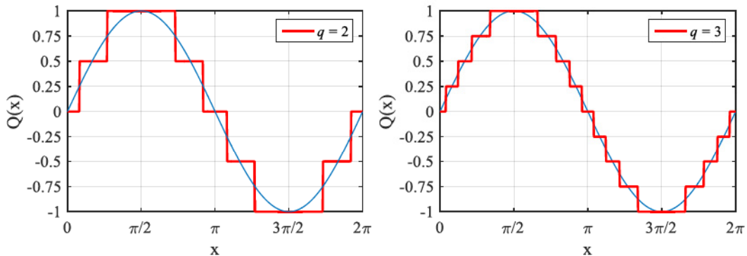
Figure 2.13: Example of uniform-quantized signals, using 2, or 3 bits, i.e. 4 and 8 possible levels.
