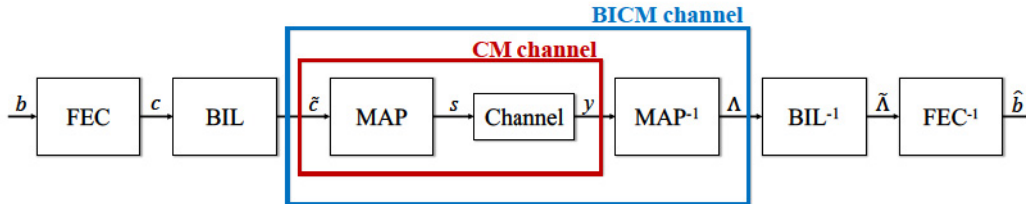
Figure 2.4: Transmit to receive BICM system block diagram.
