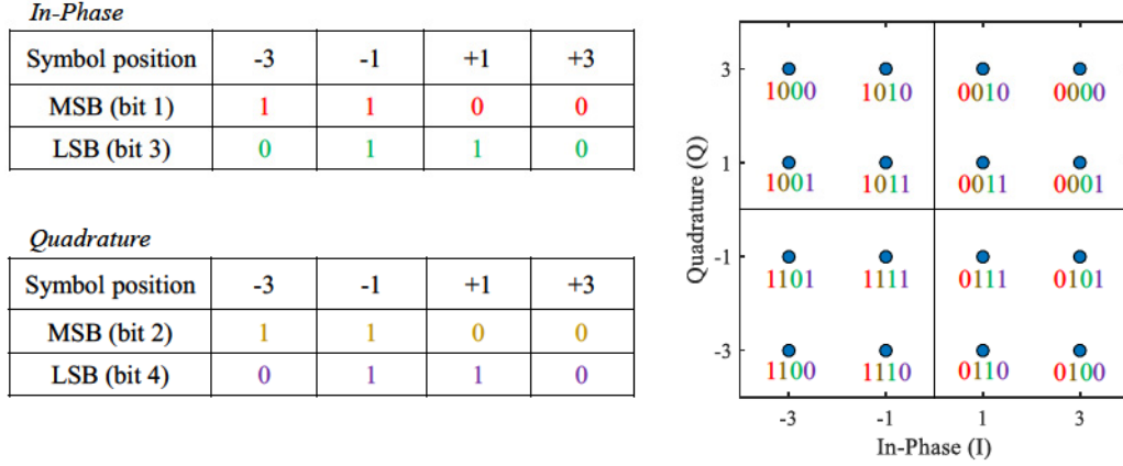
Figure 2.6: Gray mapping for 16QAM constellations.
