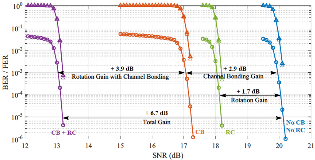
Figure 3.30: SNR performance with channel bonding and/or rotation. Two RF channels, for a QPSK CR 13/15 and i.i.d. Rayleigh channel, PI of 9 dB.
