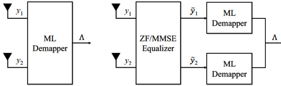
Figure 2.14: Two demapping configurations considered. Optimum ML (left) vs. ZF/MMSE (right).
