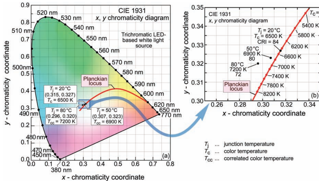
Fig. 4. Change in chromaticity coordinate, correlated color temperature, and CRI of trichromatic LED light source for junction temperatures of T_j = 20^\circ, 50^\circ, and 80^\circ\text{C} represented in the (x, y) chromaticity diagram.
