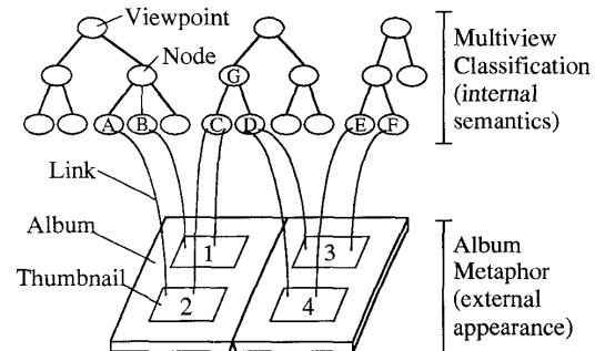
Fig. 1 Conceptual Model of Digital Album
