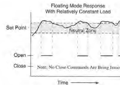
Figure 8.10 Floating Controller Response to Constant Load
