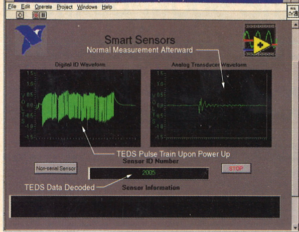
Figure 5. TEDS decoding with LabVIEW (courtesy of National Instruments).
