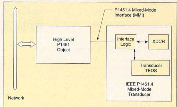
Figure 2. IEEE P1451.4 interface.
