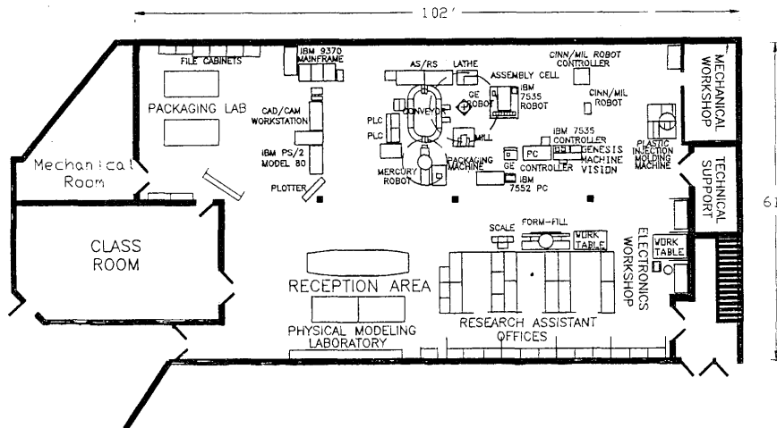
Figure 1. Layout of UMR Engineering Management CIM Laboratory
