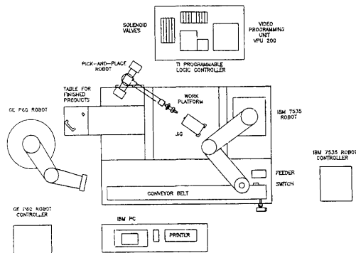
Figure 2. Layout of Flexible Assembly Cell
