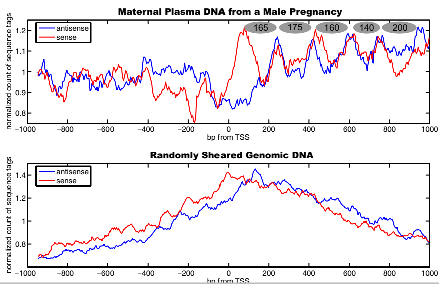
Fig. 4. Distribution of sequence tags around transcription start sites (TSS) of ReSeq genes on all autosomes and chromosome X from plasma DNA sample of a normal male pregnancy (Upper) and randomly sheared genomic DNA control (Lower). The number of tags within each 5-bp window was counted within \pm 1,000 -bp region around each TSS, taking into account the strand to which each sequence tag mapped. The counts from all transcription start sites for each 5-bp window were summed and normalized to the median count among the 400 windows. A moving average was used to smooth the data. A peak in the sense strand represents the beginning of a nucleosome, whereas a peak in the antisense strand represents the end of a nucleosome. In the plasma DNA sample shown here, five well positioned nucleosomes are observed downstream of transcription start sites and are represented as gray ovals. The number within each oval represents the distance in base pairs between adjacent peaks in the sense and antisense strands, corresponding to the size of the inferred nucleosome. No obvious pattern is observed for the genomic DNA control.
