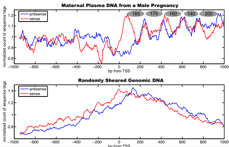
Fig. 4. Distribution of sequence tags around transcription start sites (TSS) of ReSeq genes on all autosomes and chromosome X from plasma DNA sample of a normal male pregnancy ( Upper ) and randomly sheared genomic DNA control ( Lower ). The number of tags within each 5-bp window was counted within \pm 1,000 -bp region around each TSS, taking into account the strand to which each sequence tag mapped. The counts from all transcription start sites for each 5-bp window were summed and normalized to the median count among the 400 windows. A moving average was used to smooth the data. A peak in the sense strand represents the beginning of a nucleosome, whereas a peak in the antisense strand represents the end of a nucleosome. In the plasma DNA sample shown here, five well positioned nucleosomes are observed downstream of transcription start sites and are represented as gray ovals. The number within each oval represents the distance in base pairs between adjacent peaks in the sense and antisense strands, corresponding to the size of the inferred nucleosome. No obvious pattern is observed for the genomic DNA control.
