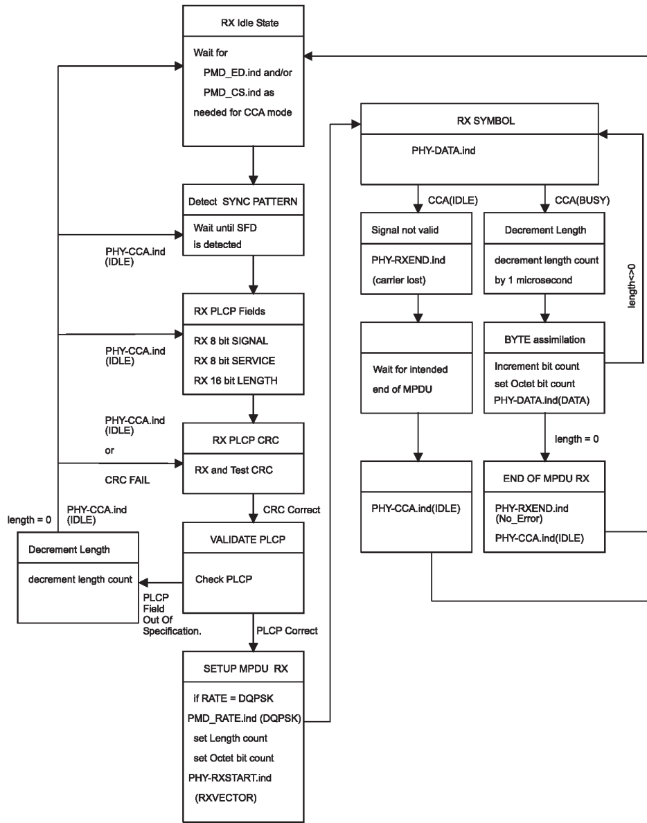
Figure 15-9—PLCP receive state machine
