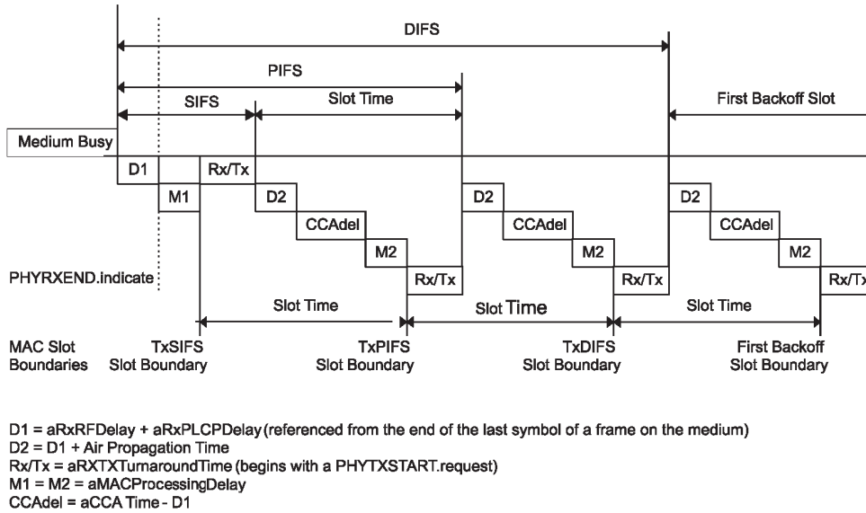
Figure 9-12—DCF timing relationships
