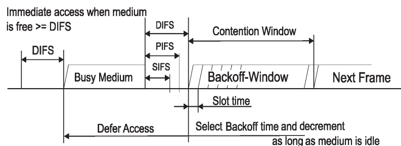
Figure 9-5—Basic access method
