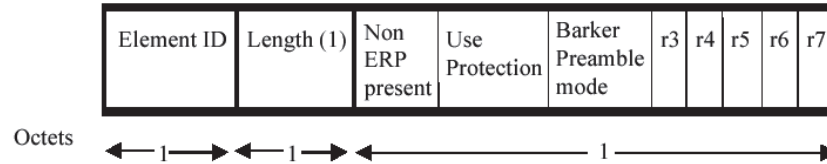
Figure 7-50—ERP Information element
