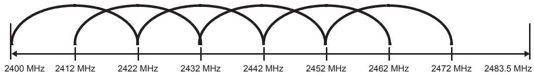
Figure 18-16—China and North American channel selection—overlapping
