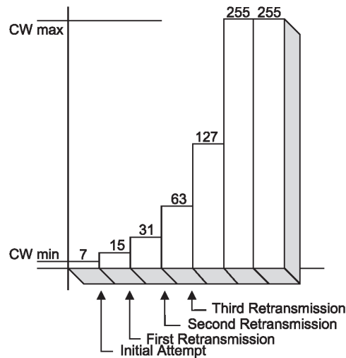
Figure 9-4—Example of exponential increase of CW
