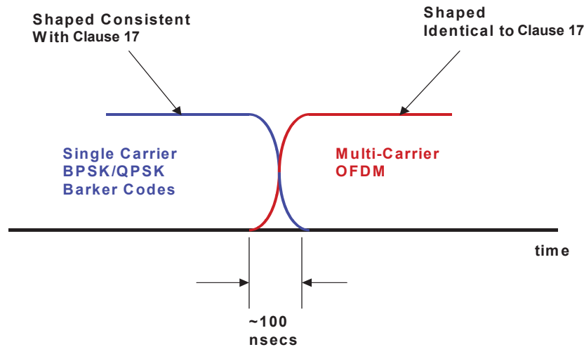
Figure 19-18—Single carrier termination requirement
