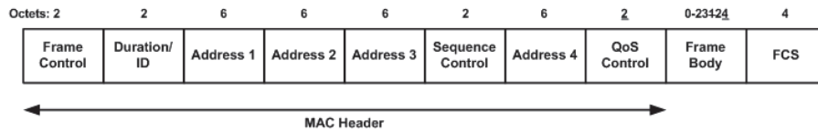
Figure 7-1—MAC frame format
