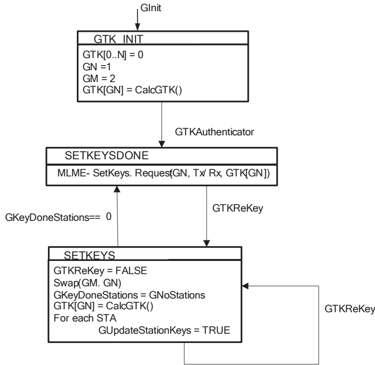
Figure 8-40—Authenticator state machines, part 4
