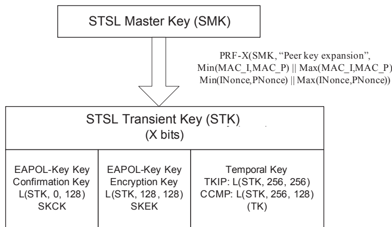
Figure 8-22—PeerKey hierarchy
