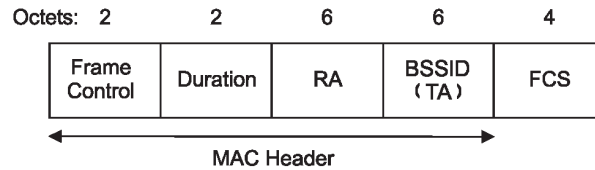
Figure 7-11—CF-End+CF-Ack frame
