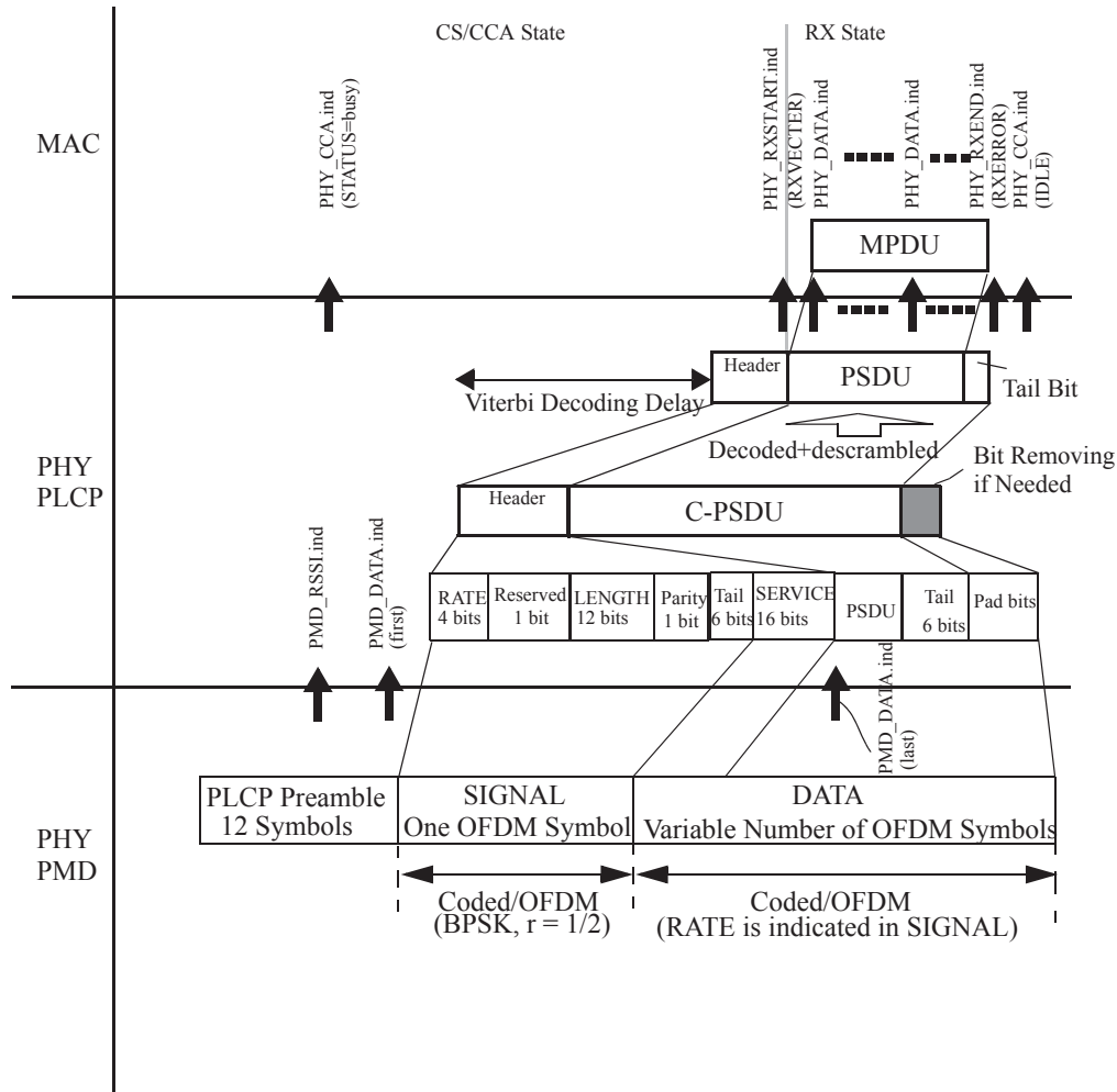
Figure 17-16—Receive PLCP
