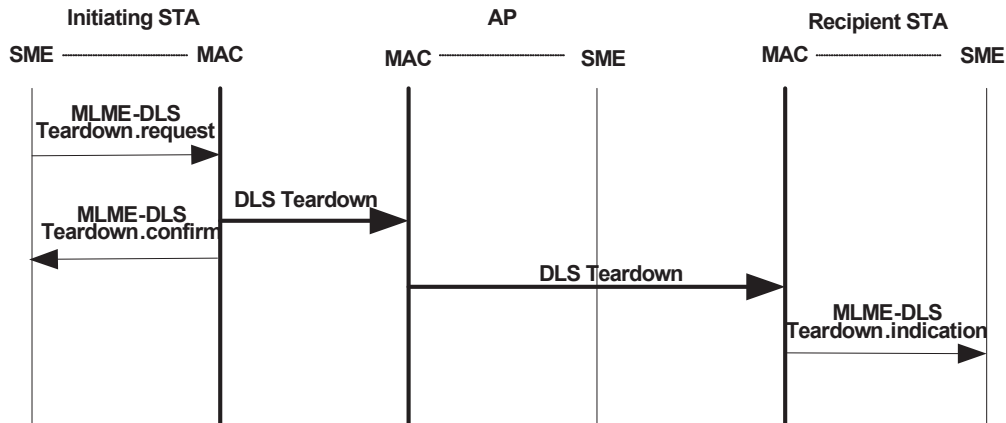
Figure 11-17—STA-initiated DLS teardown message flow
