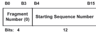
Figure 7-14—Block Ack Starting Sequence Control field
