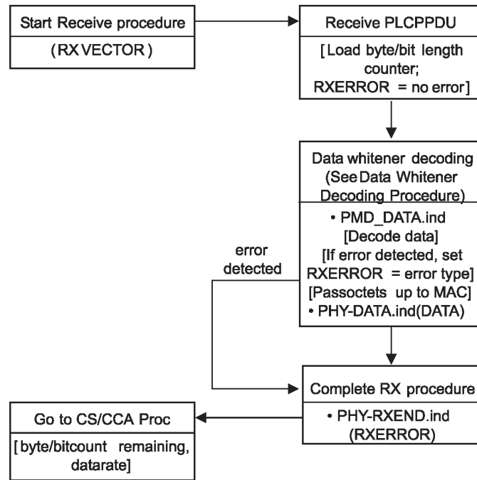
Figure 14-11—Receive state machine
