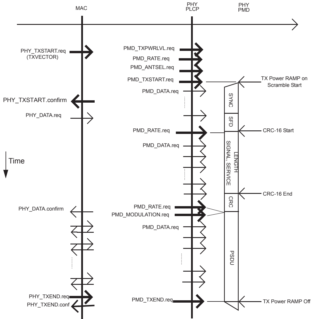
Figure 18-7—Transmit PLCP
