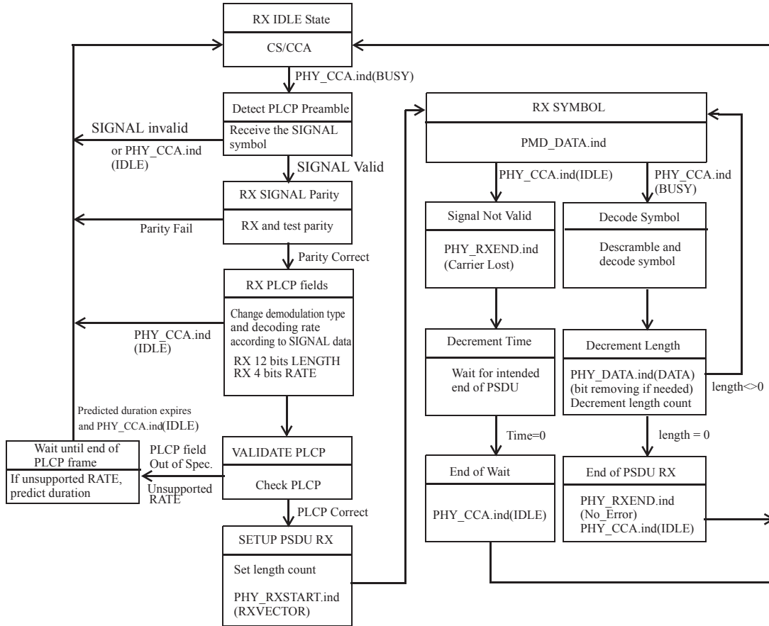
Figure 17-17—PLCP receive state machine
