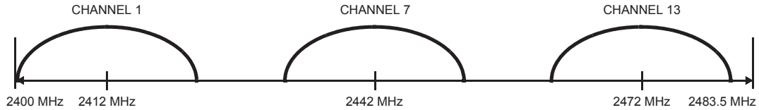
Figure 18-17—European channel selection—nonoverlapping
