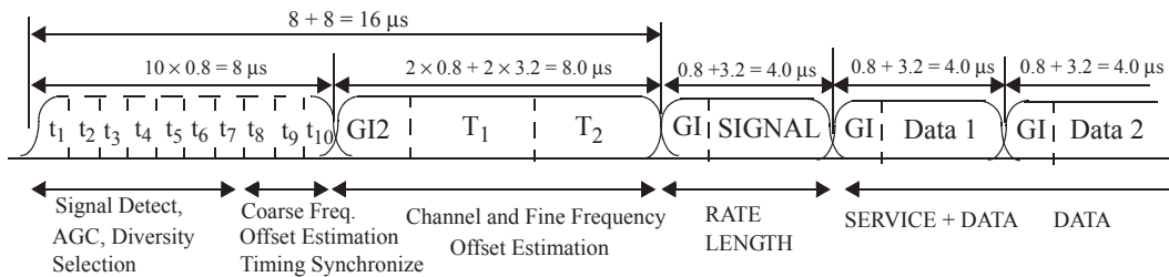
Figure 17-4—OFDM training structure
