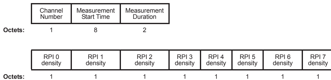
Figure 7-68—Measurement Report field format for an RPI histogram report
