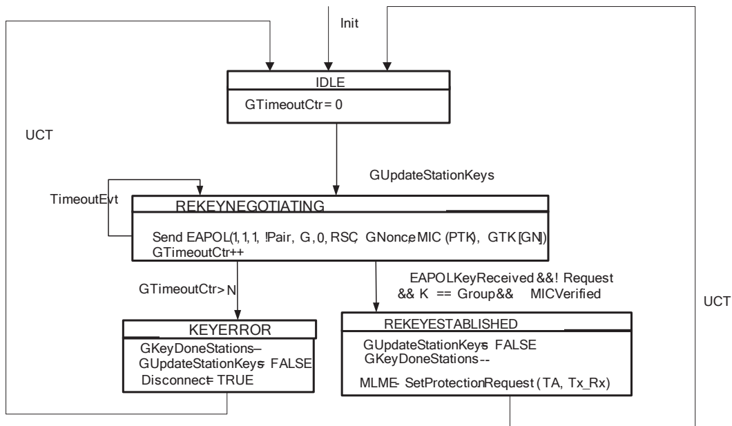
Figure 8-39—Authenticator state machines, part 3
