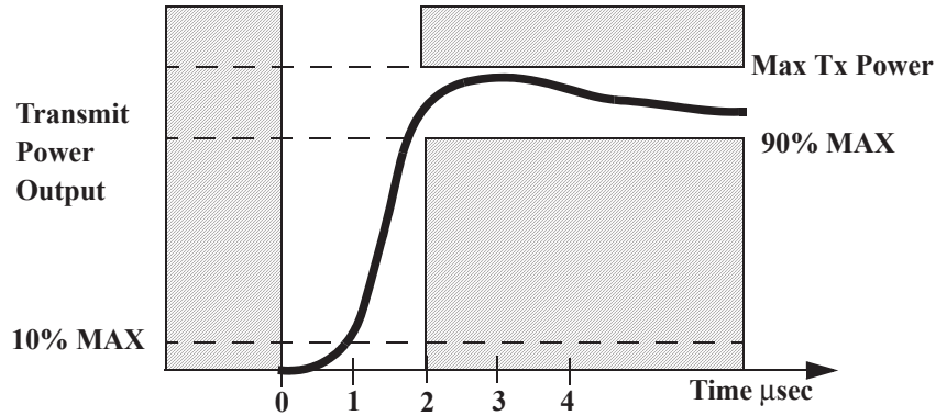
Figure 18-20—Transmit power-on ramp
