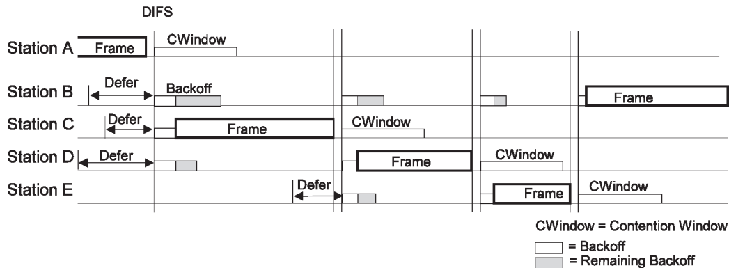
Figure 9-6—Backoff procedure
