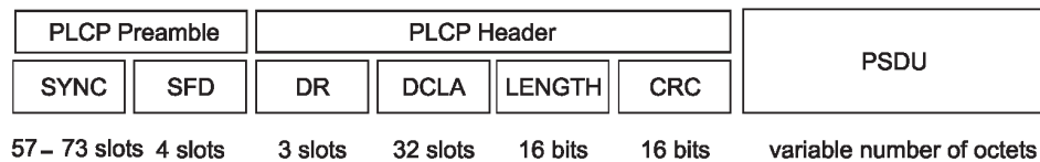
Figure 16-1—PPDU frame format
