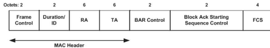
Figure 7-12—BlockAckReq frame
