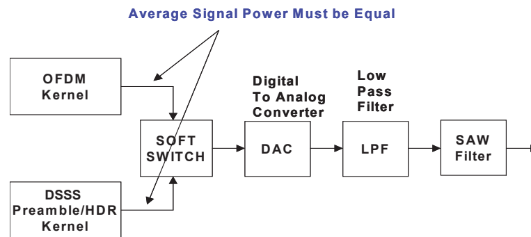
Figure 19-15—Comparing signal power
