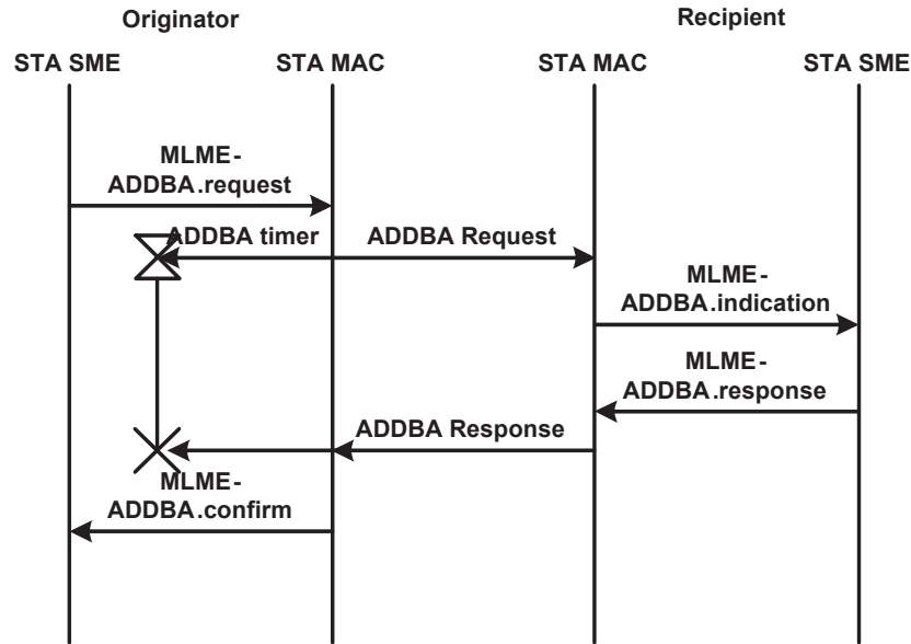
Figure 11-12—Block Ack setup
