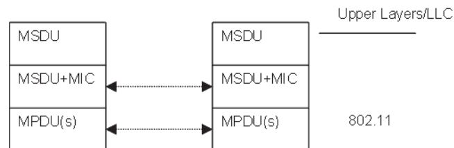
Figure 8-7—TKIP MIC relation to IEEE 802.11 processing (informative)
