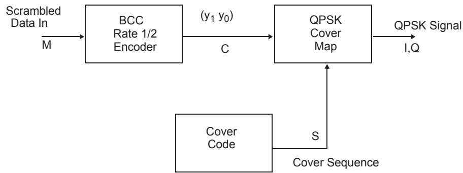
Figure 18-12—PBCC modulator scheme
