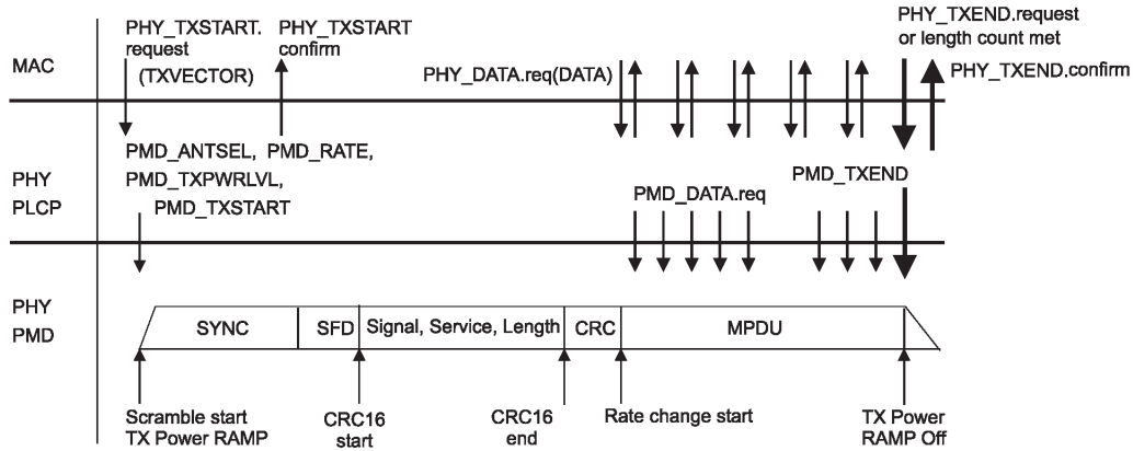
Figure 15-6—Transmit PLCP
