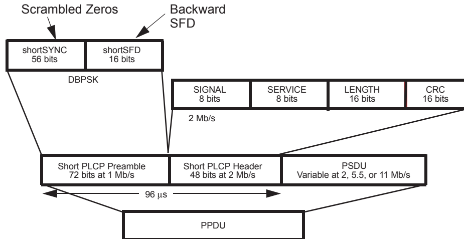
Figure 18-2—Short PPDU format
