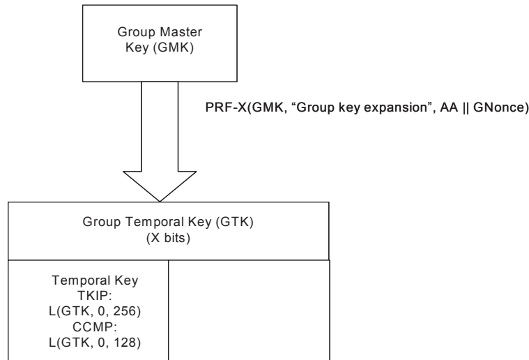
Figure 8-21—Group key hierarchy (informative)
