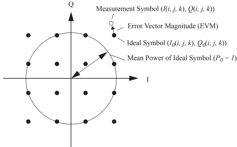
Figure 17-13—Constellation error
