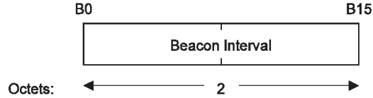
Figure 7-21—Beacon Interval field
