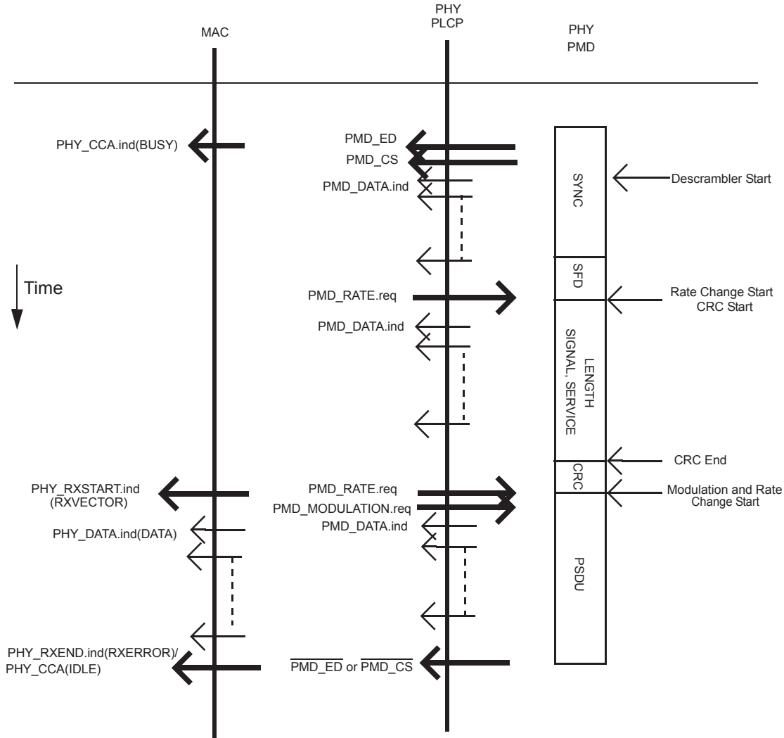
Figure 18-9—Receive PLCP
