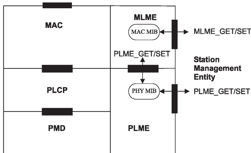
Figure 10-1—GET and SET operations
