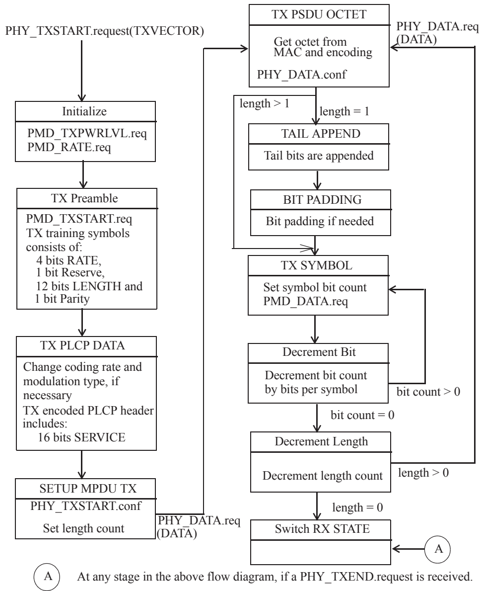
Figure 17-15—PLCP transmit state machine
