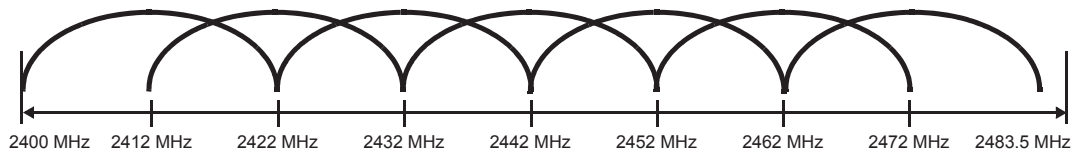
Figure 18-18—European channel selection—overlapping
