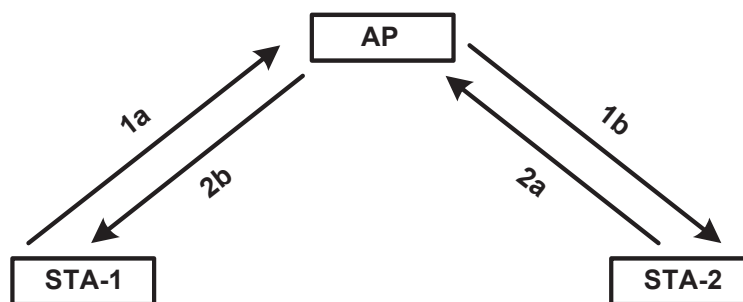
Figure 11-15—The four steps involved in direct-link handshake
