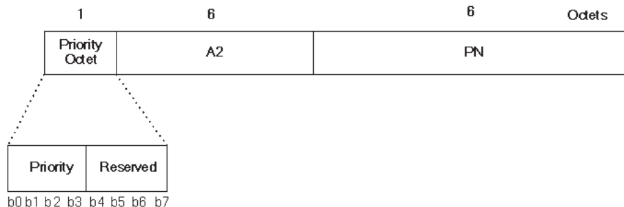
Figure 8-18—Nonce construction
