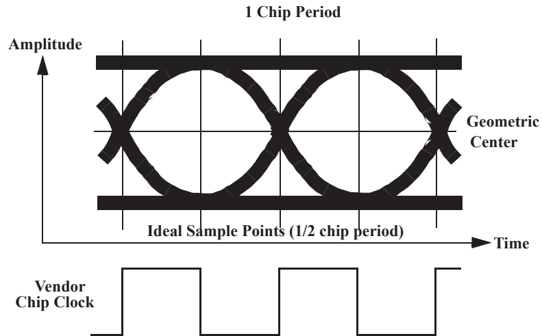
Figure 18-23—Chip clock alignment with baseband eye pattern
