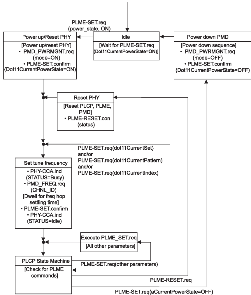
Figure 14-14—PLME state machine
