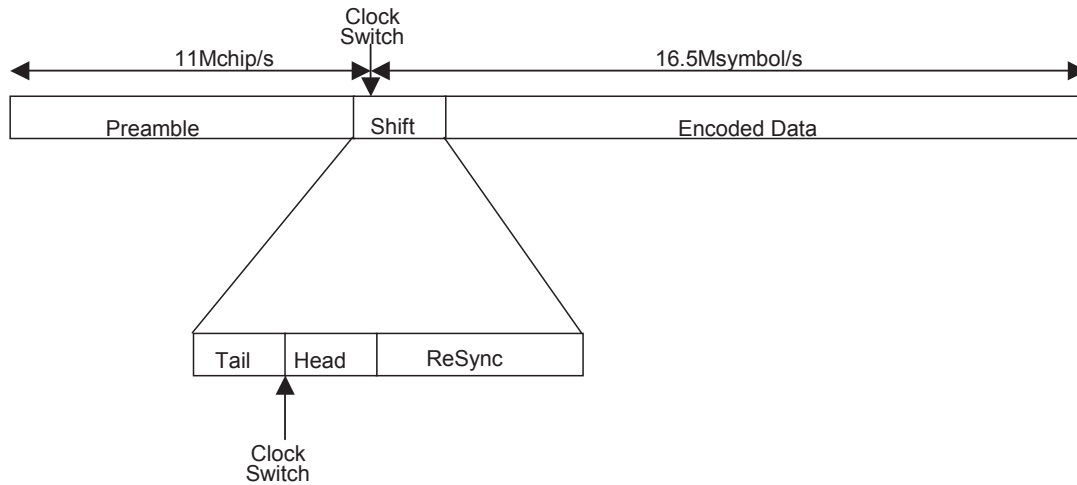
Figure 19-5—33 Mb/s clock switching
