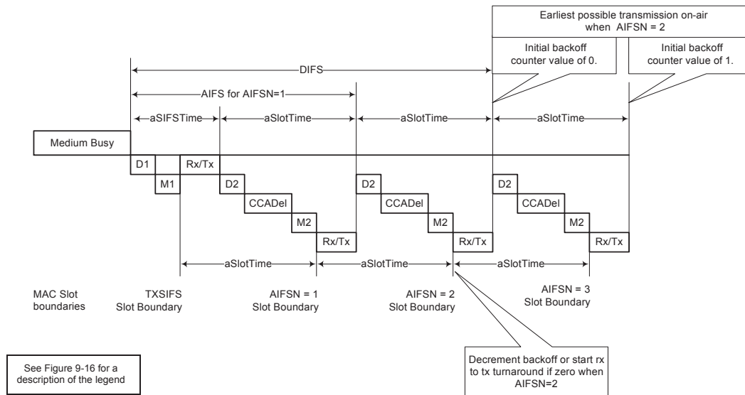
Figure 9-18—EDCA mechanism timing relationships
