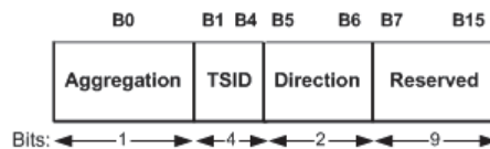
Figure 7-94—Schedule Info field
