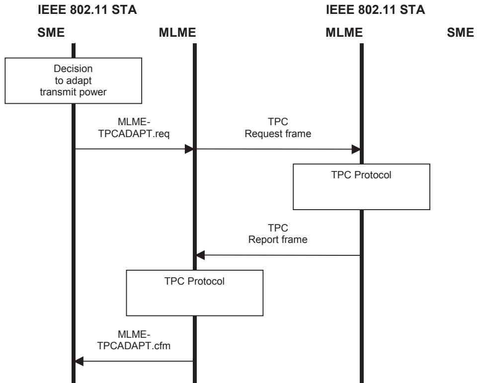
Figure 10-5—TPC adaptation
