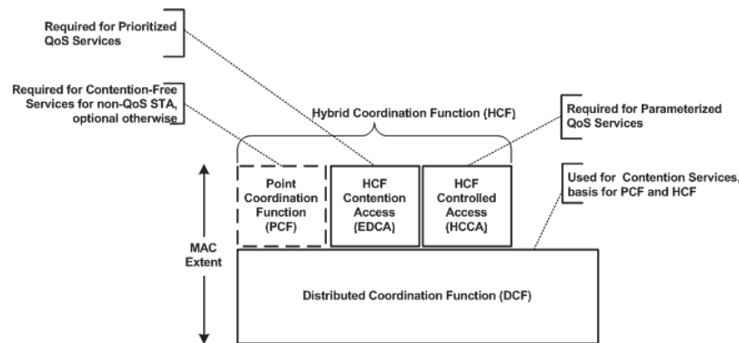
Figure 9-1—MAC architecture
