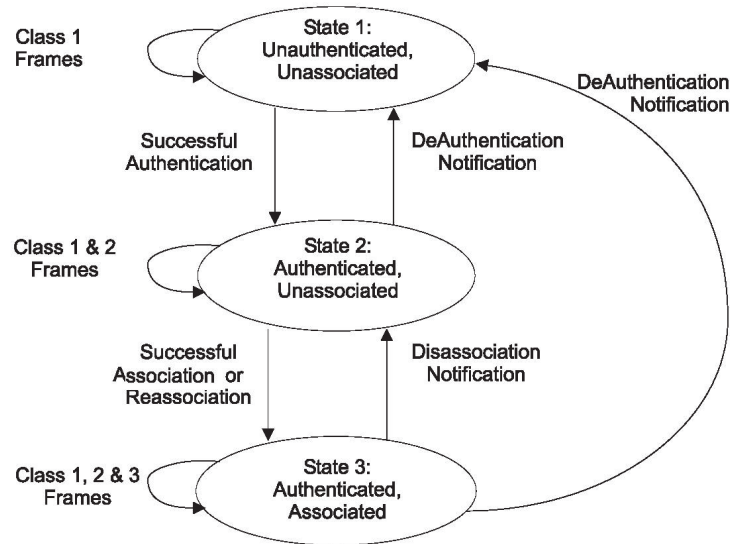
Figure 11-6—Relationship between state variables and services
