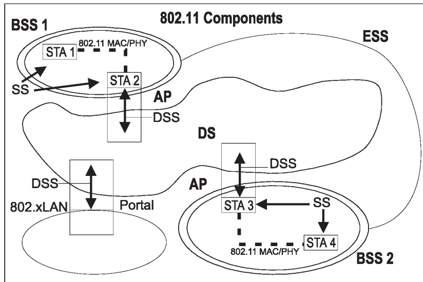
Figure 5-8—IEEE 802.11 architecture (again)
