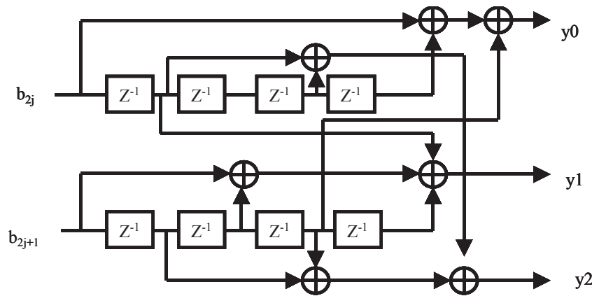
Figure 19-3—22/33 Mb/s ERP-PBCC convolutional encoder
