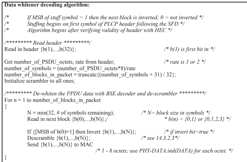
Figure 14-12—Data whitener decoding procedure
