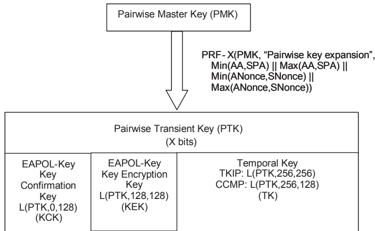
Figure 8-20—Pairwise key hierarchy
