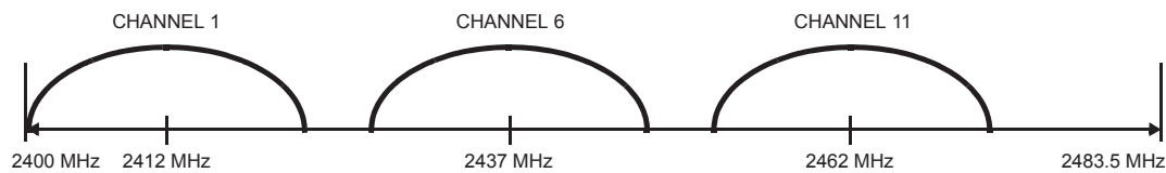
Figure 18-15—China and North American channel selection—nonoverlapping
