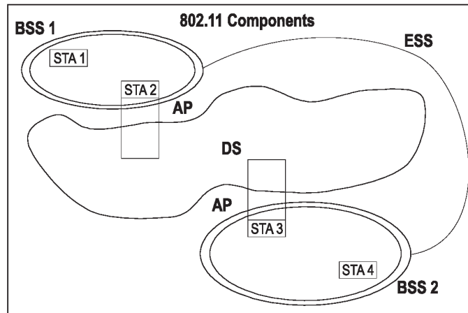
Figure 5-3—ESS
