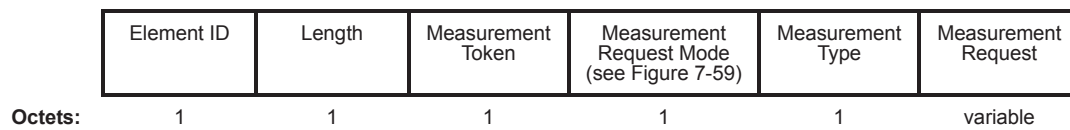
Figure 7-58—Measurement Request element format
