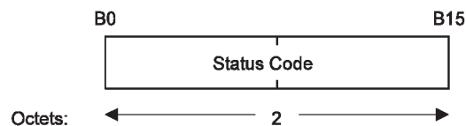
Figure 7-27—Status Code field
