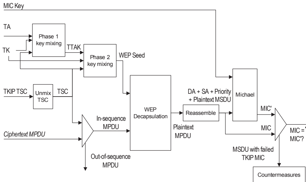
Figure 8-5—TKIP decapsulation block diagram
