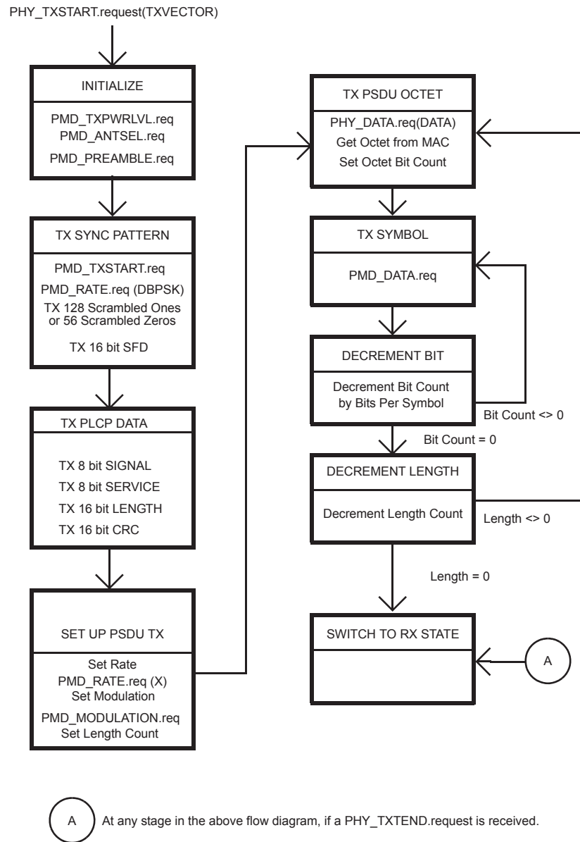
Figure 18-8—PLCP transmit state machine
