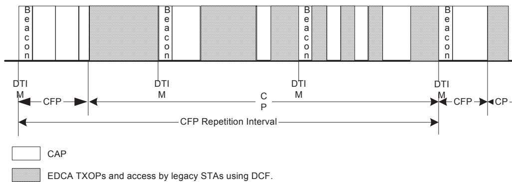
Figure 9-19—CAP/CFP/CP periods
