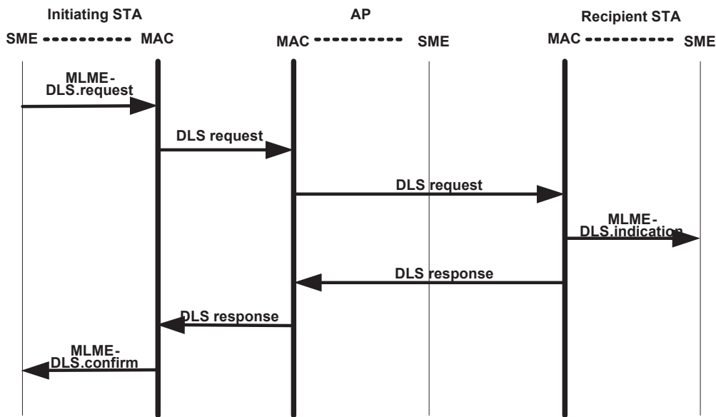
Figure 11-16—DLS message flow
