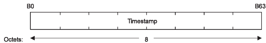
Figure 7-28—Timestamp field
