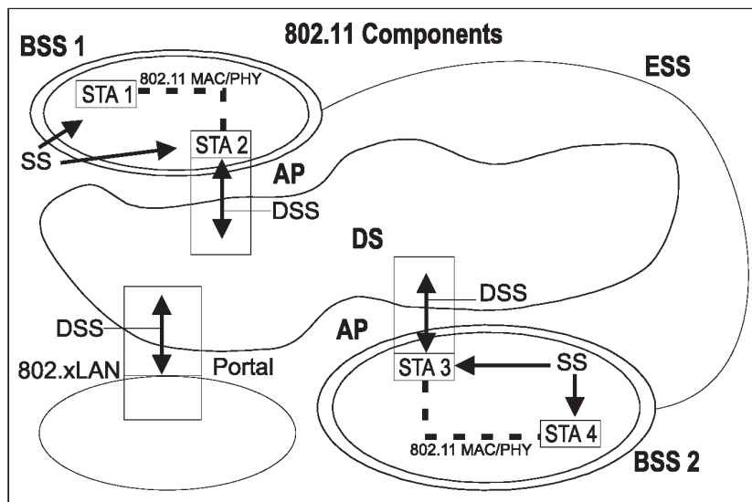
Figure 5-7—Complete IEEE 802.11 architecture
