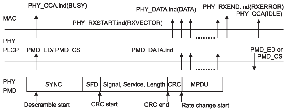
Figure 15-8—Receive PLCP
