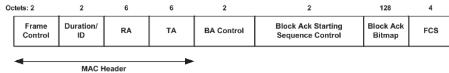
Figure 7-15—BlockAck frame
