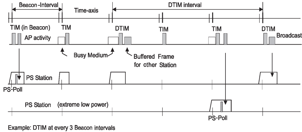
Figure 11-4—Infrastructure power management operation (no PCF operating)
