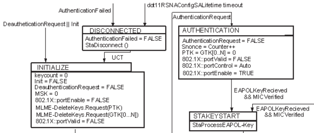
Figure 8-35—RSNA Supplicant key management state machine
