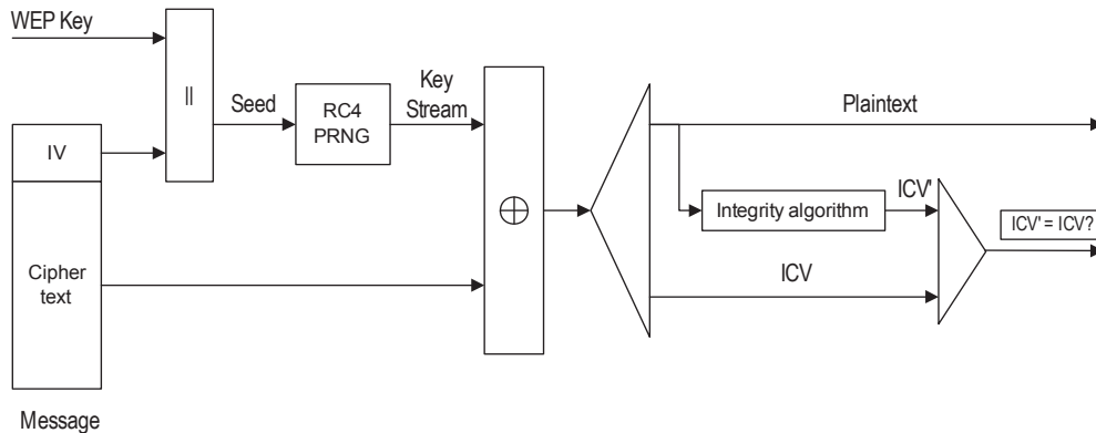
Figure 8-3—WEP decapsulation block diagram
