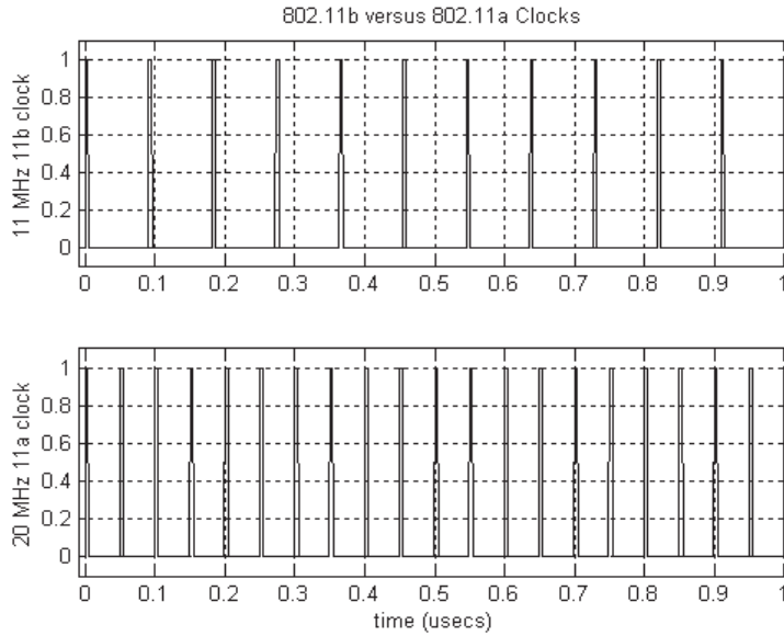
Figure 19-16—Aligning the 11 MHz and 20 MHz clocks
