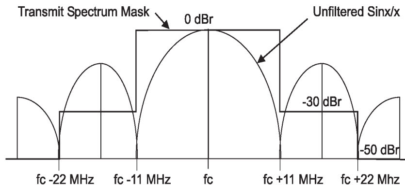
Figure 18-19—Transmit spectrum mask
