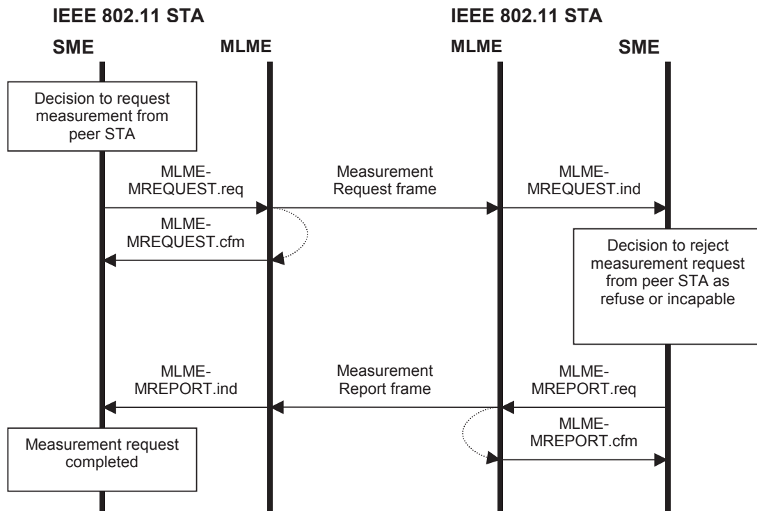
Figure 10-4—Measurement request—rejected
