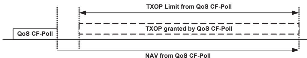
Figure 9-20—Polled TXOP
