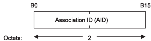
Figure 7-26—AID field
