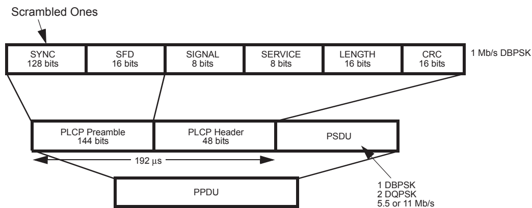
Figure 18-1—Long PPDU format
