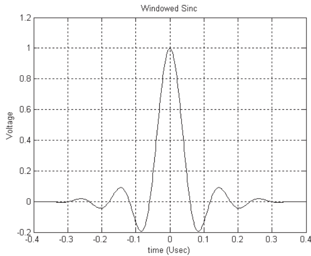
Figure 19-13—Specified pulse
