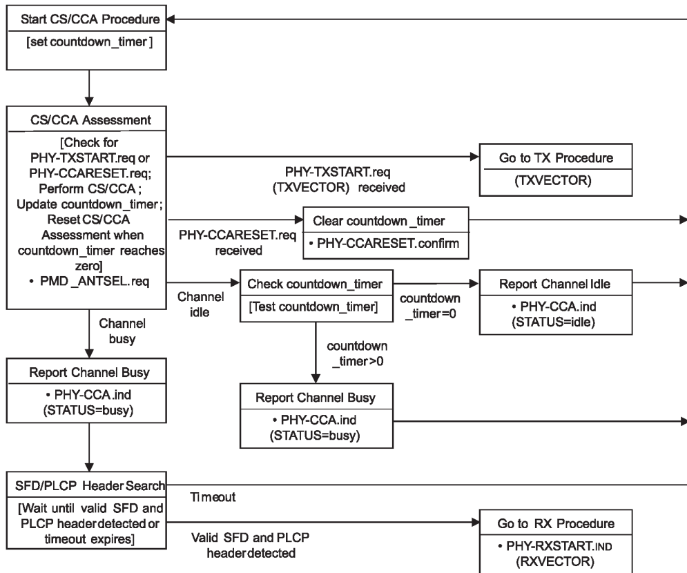
Figure 14-9—CS/CCA state machine
