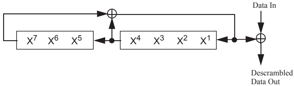
Figure 17-7—Data scrambler
