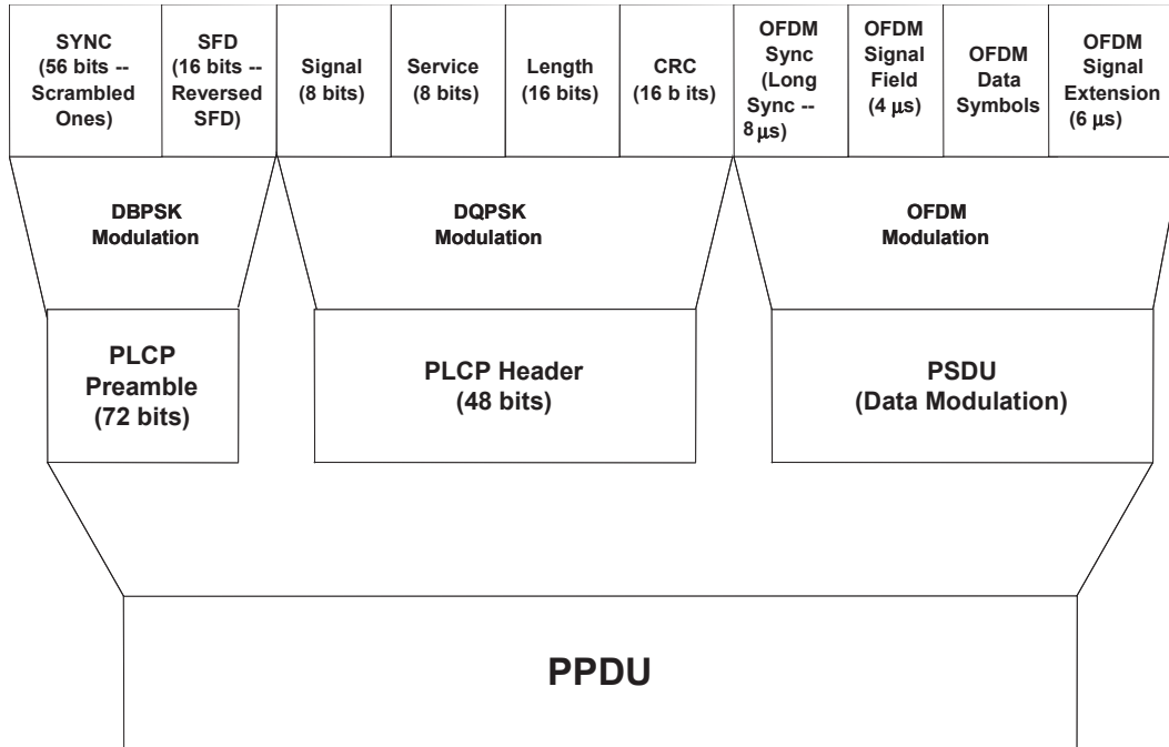
Figure 19-2—Short preamble PDU format for DSSS-OFDM
