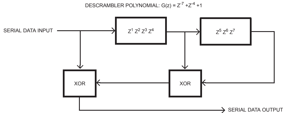
Figure 18-6—Data descrambler
