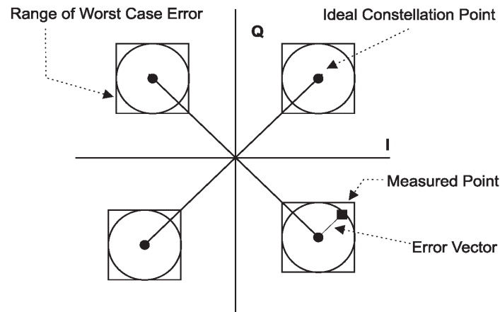
Figure 18-22—Modulation accuracy measurement example
