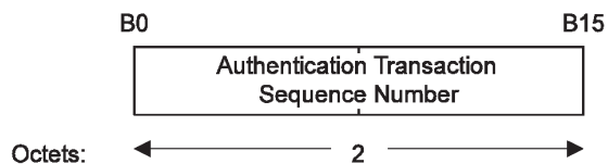
Figure 7-20—Authentication Transaction Sequence Number field
