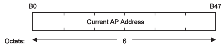
Figure 7-23—Current AP Address field
