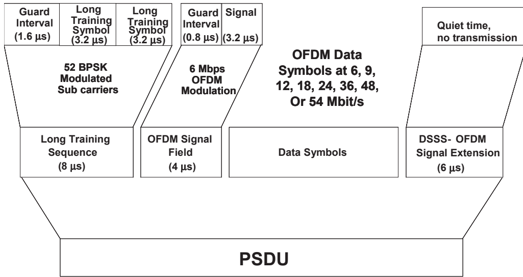
Figure 19-6—DSSS-OFDM PSDU
