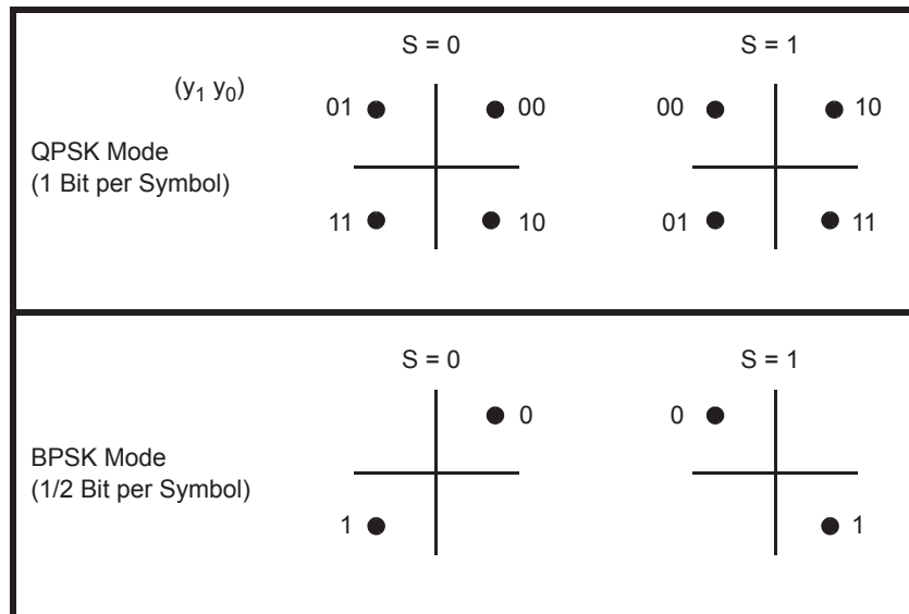
Figure 18-14—Cover code mapping
