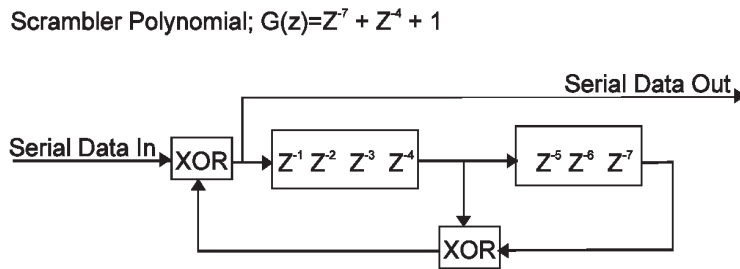
Figure 15-4—Data scrambler
