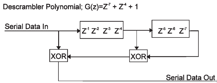
Figure 15-5—Data descrambler
