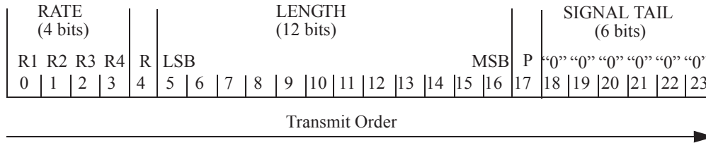
Figure 17-5—SIGNAL field bit assignment
