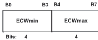
Figure 7-81—ECWmin and ECWmax fields
