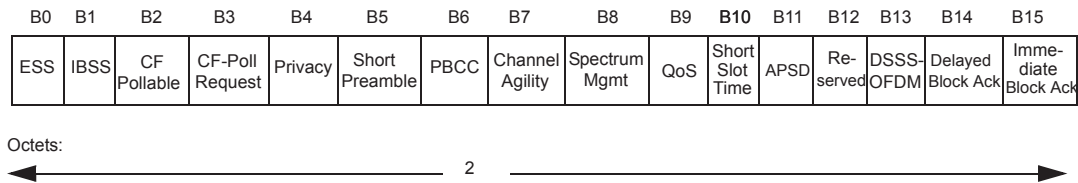
Figure 7-22—Capability Information field
