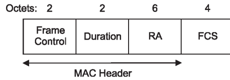
Figure 7-8—ACK frame
