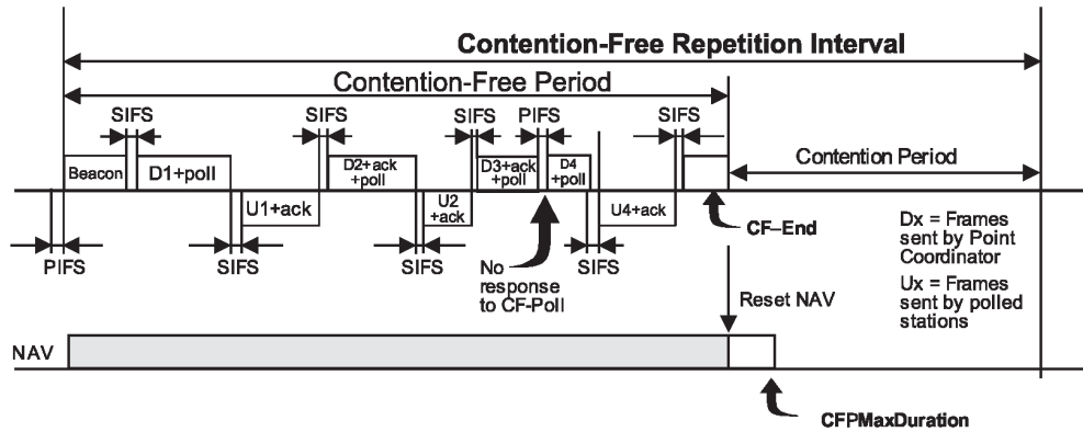
Figure 9-16—Example of PCF frame transfer
