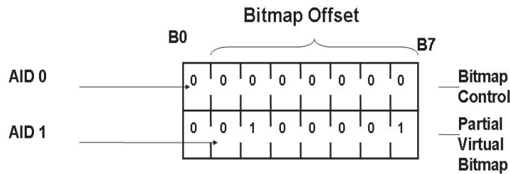
Figure L.1—Virtual bitmap example #1
