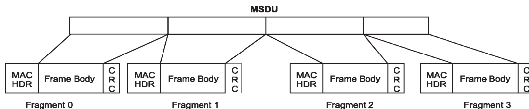
Figure 9-2—Fragmentation
