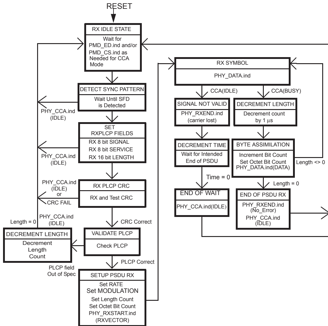
Figure 18-10—PLCP receive state machine
