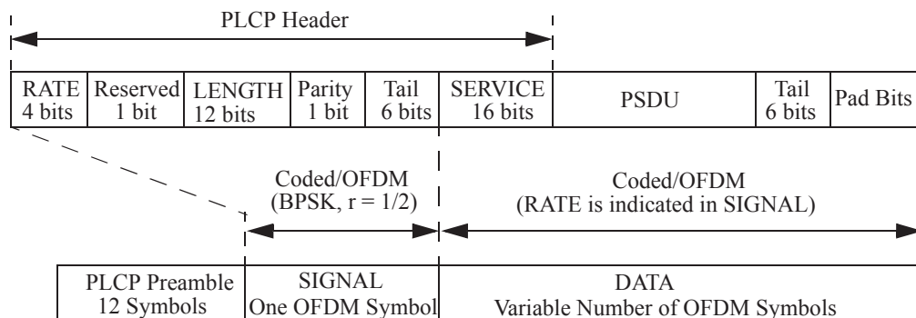
Figure 17-1—PPDU frame format
