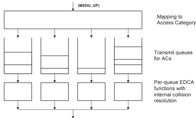
Figure 9-17—Reference implementation model
