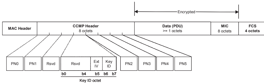
Figure 8-15—Expanded CCMP MPDU
