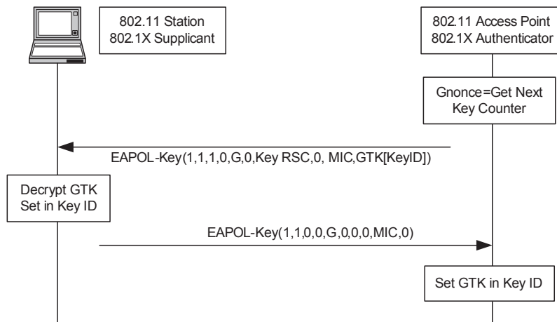
Figure 8-34—Sample Group Key Handshake
