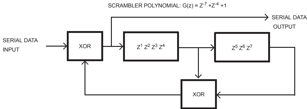
Figure 18-5—Data scrambler
