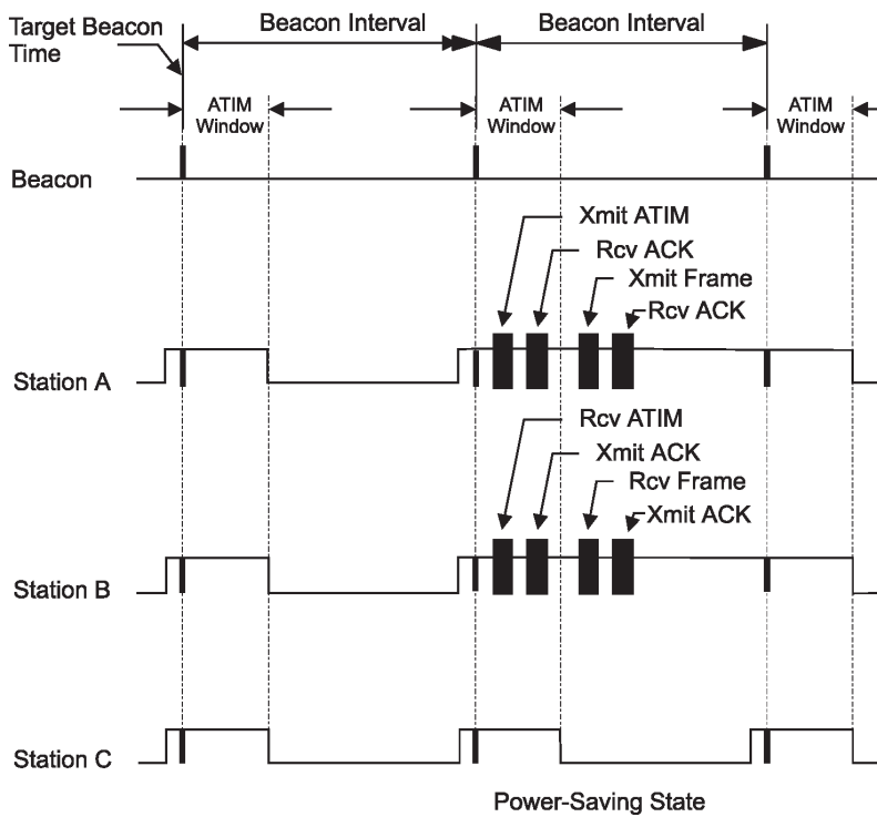
Figure 11-5—Power management in an IBSS—basic operation
