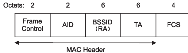
Figure 7-9—PS-Poll frame
