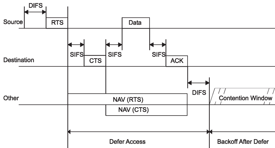
Figure 9-7—RTS/CTS/data/ACK and NAV setting
