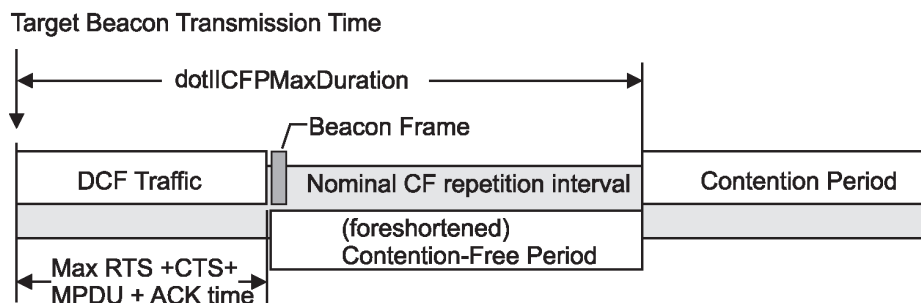
Figure 9-15—Example of delayed beacon and foreshortened CFP
