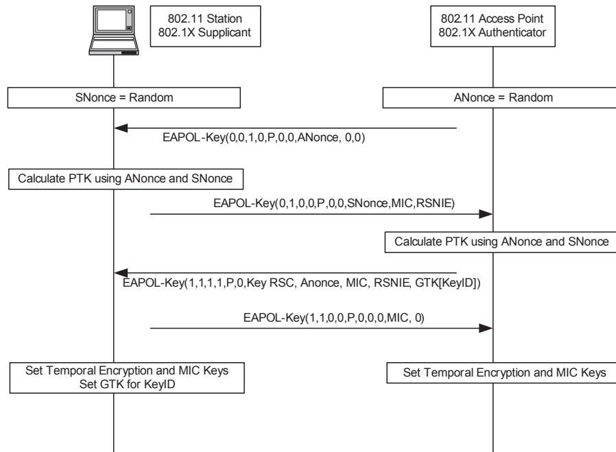
Figure 8-33—Sample 4-Way Handshake
