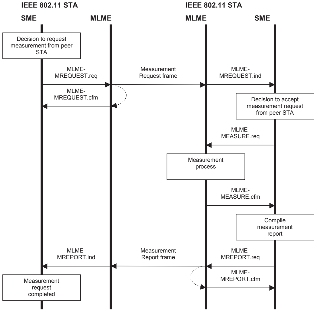
Figure 10-3—Measurement request—accepted
