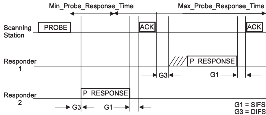
Figure 11-3—Probe response
