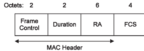
Figure 7-7—CTS frame
