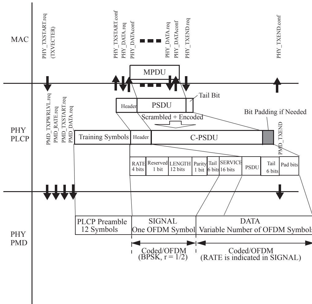
Figure 17-14—Transmit PLCP
