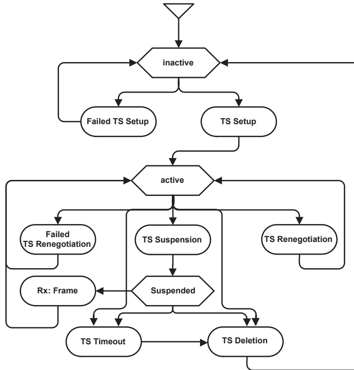
Figure 11-7—TS lifecycle
