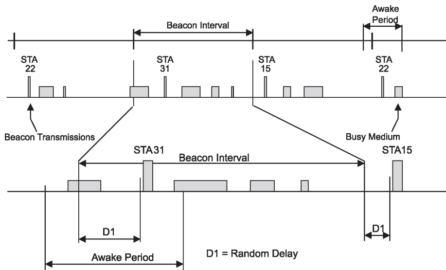
Figure 11-2—Beacon transmission in an IBSS
