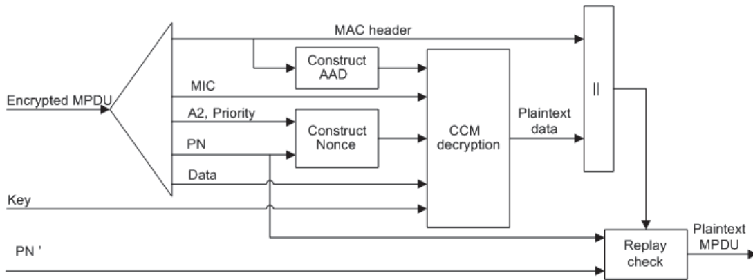
Figure 8-19—CCMP decapsulation block diagram
