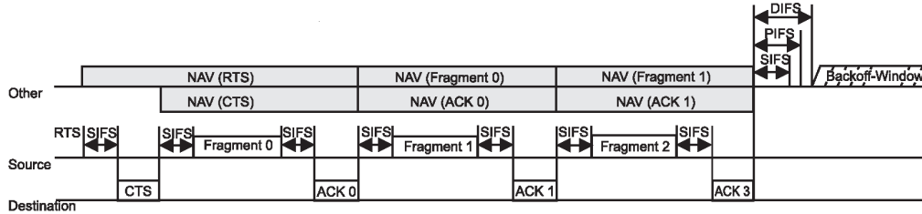
Figure 9-9—RTS/CTS with fragmented MSDU
