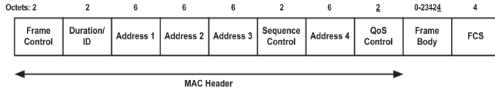
Figure 7-17—Data frame
