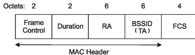
Figure 7-10—CF-End frame
