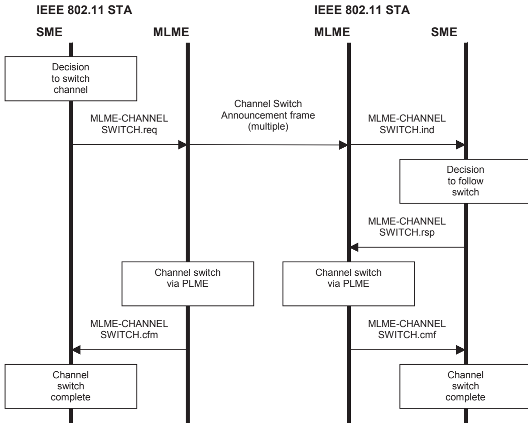
Figure 10-6—Channel switch
