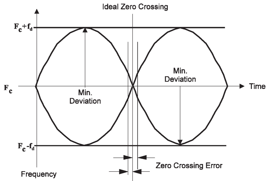
Figure 14-16—Transmit modulation mask
