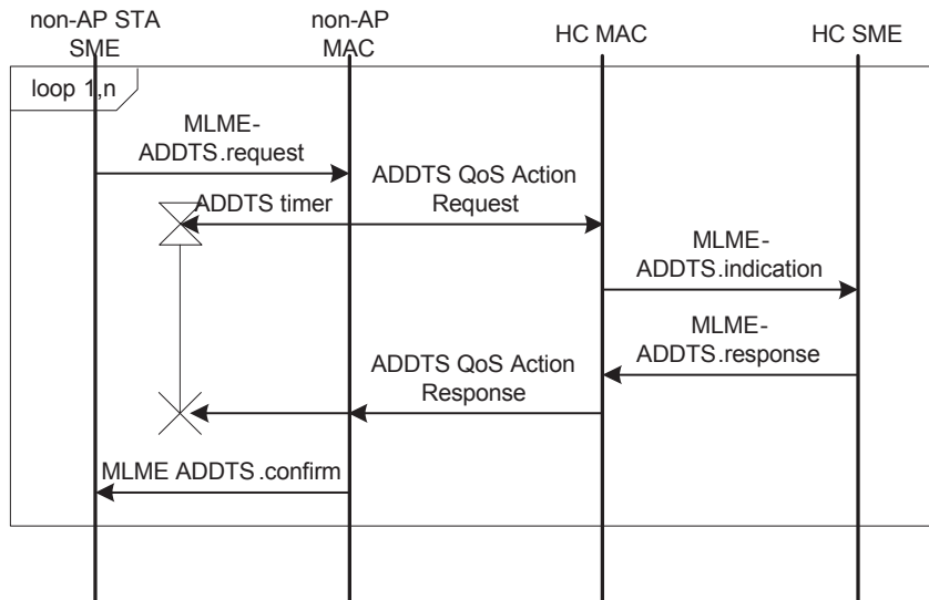
Figure 11-8—TS setup
