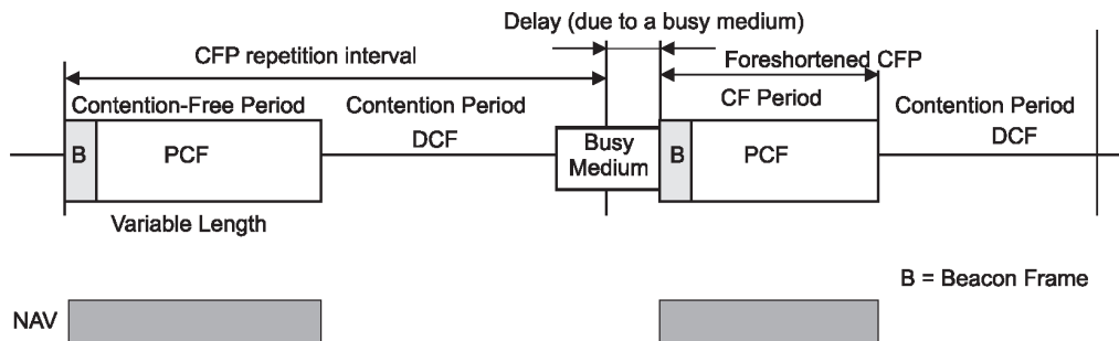
Figure 9-13—CFP/CP alternation
