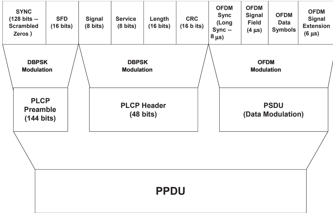
Figure 19-1—Long preamble PDU format for DSSS-OFDM
