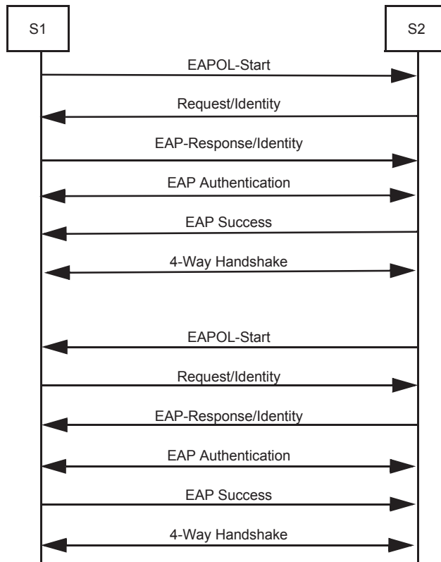
Figure 5-16—Example using IEEE 802.1X authentication
