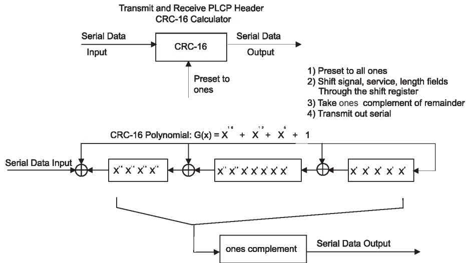
Figure 15-2—CRC-16 implementation
