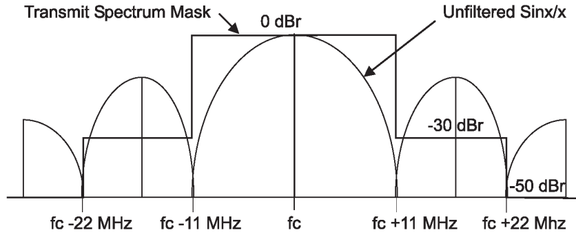
Figure 15-11—Transmit spectrum mask
