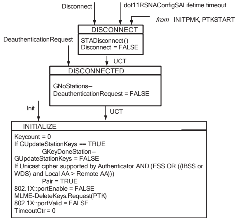
Figure 8-38—Authenticator state machines, part 2
