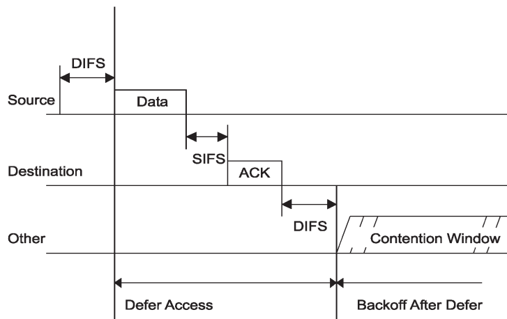
Figure 9-11—Individually addressed data/ACK MPDU
