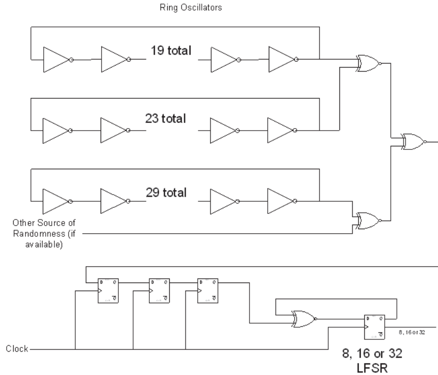
Figure H.1—Randomness generating circuit
