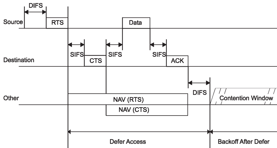
Figure 9-7—RTS/CTS/data/ACK and NAV setting
