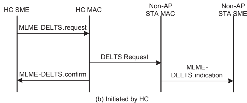
Figure 11-10—TS deletion
