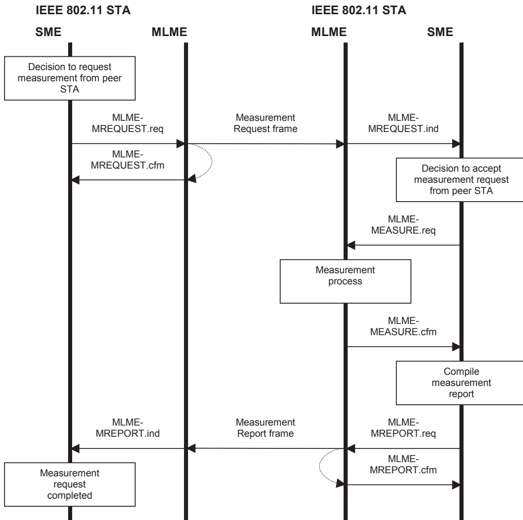
Figure 10-3—Measurement request—accepted
