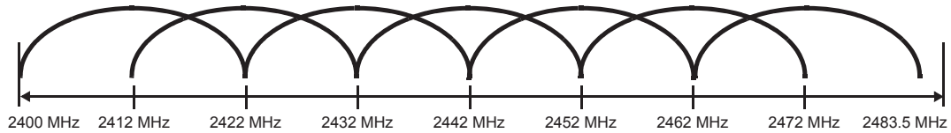
Figure 18-18—European channel selection—overlapping
