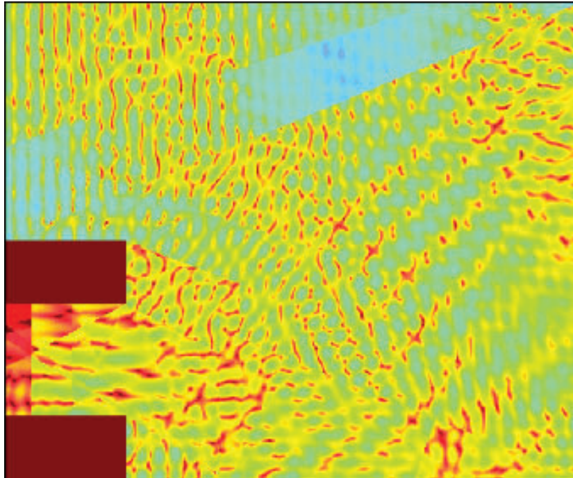
Figure 5-4—A representative signal intensity map
