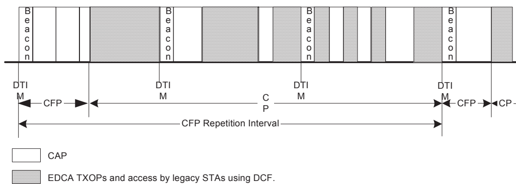
Figure 9-19—CAP/CFP/CP periods
