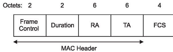
Figure 7-6—RTS frame
