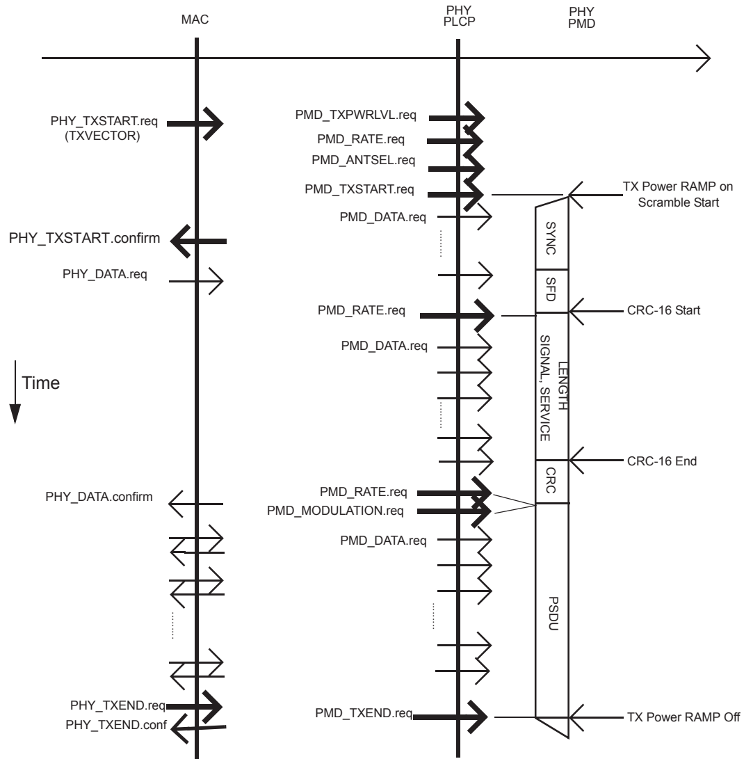
Figure 18-7—Transmit PLCP
