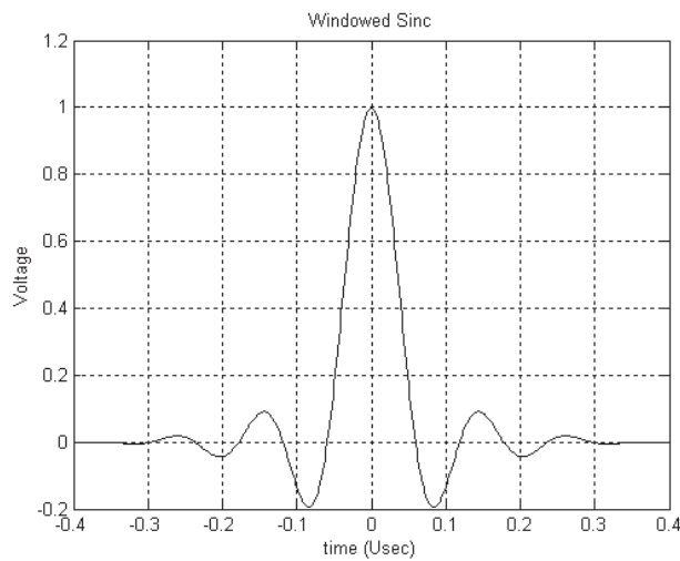
Figure 19-13—Specified pulse
