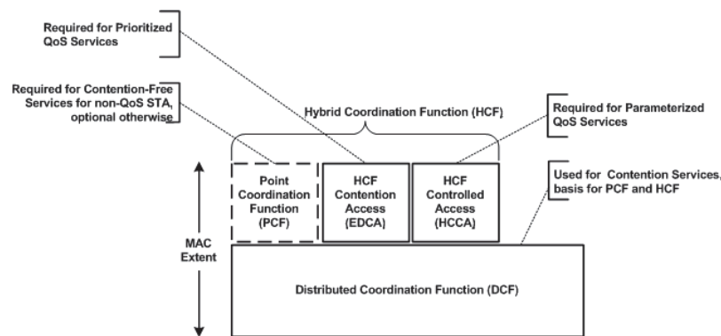
Figure 9-1—MAC architecture
