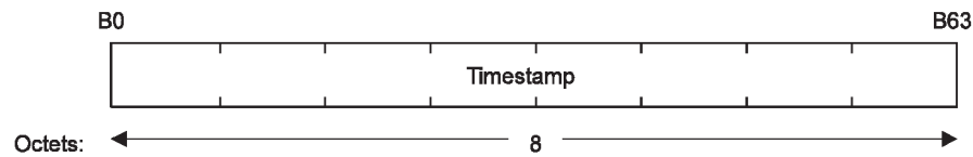
Figure 7-28—Timestamp field
