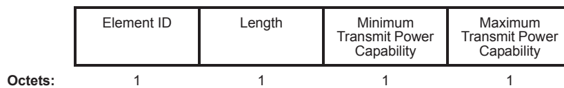
Figure 7-53—Power Capability element format
