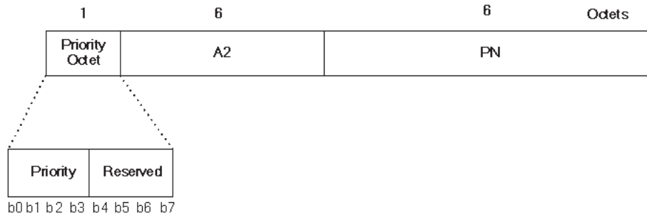
Figure 8-18—Nonce construction
