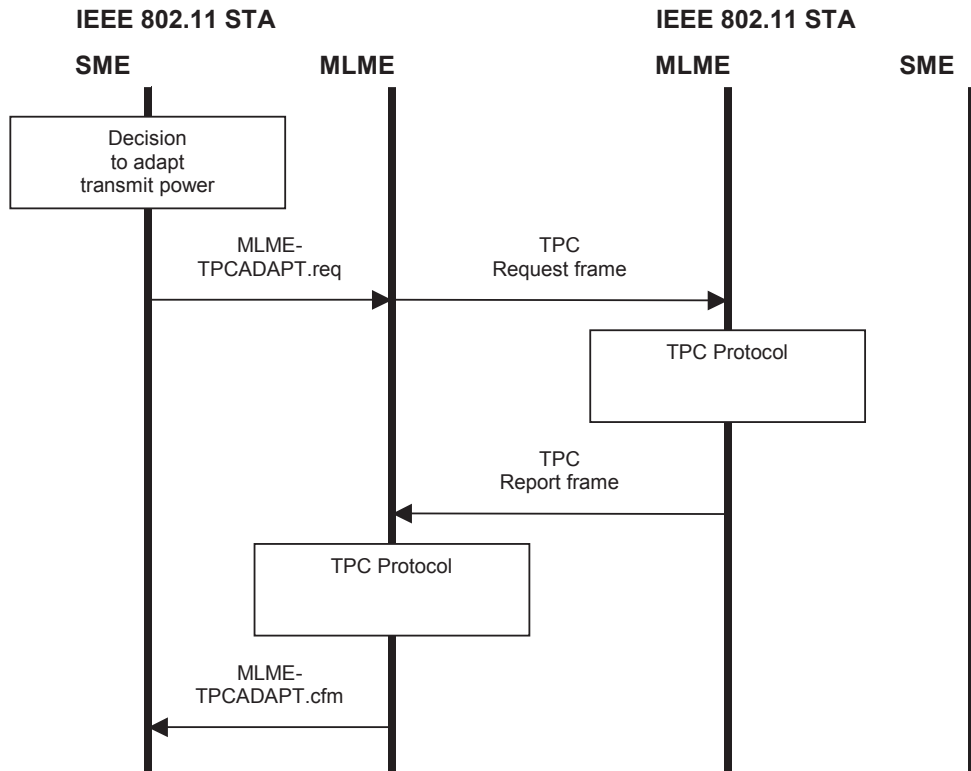
Figure 10-5—TPC adaptation
