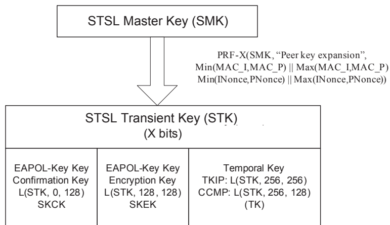
Figure 8-22—PeerKey hierarchy
