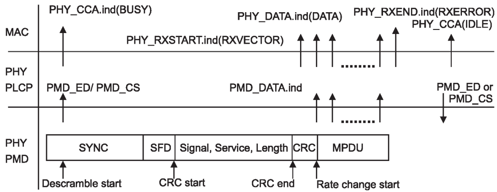
Figure 15-8—Receive PLCP
