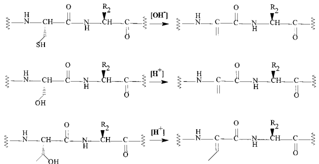
Scheme 5—β Elimination.
