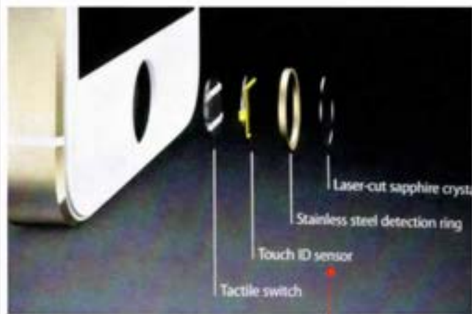
Biometric sensor 121
