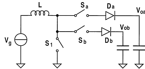
Fig. 5. Converter presented in [13].
