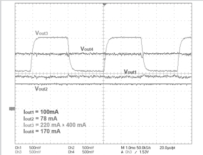
Figure 24.6.5: Measured regulated output voltages ( V_{out1} = 0.9V ch. 1, V_{out2} = 0.7V ch. 2, V_{out3} = 1.1 to 2V ch. 3, V_{out4} = 1.6V ch. 4)
