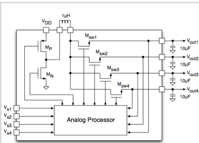
Figure 24.6.1: Architecture of the single-inductor four-output DC-DC buck converter.
