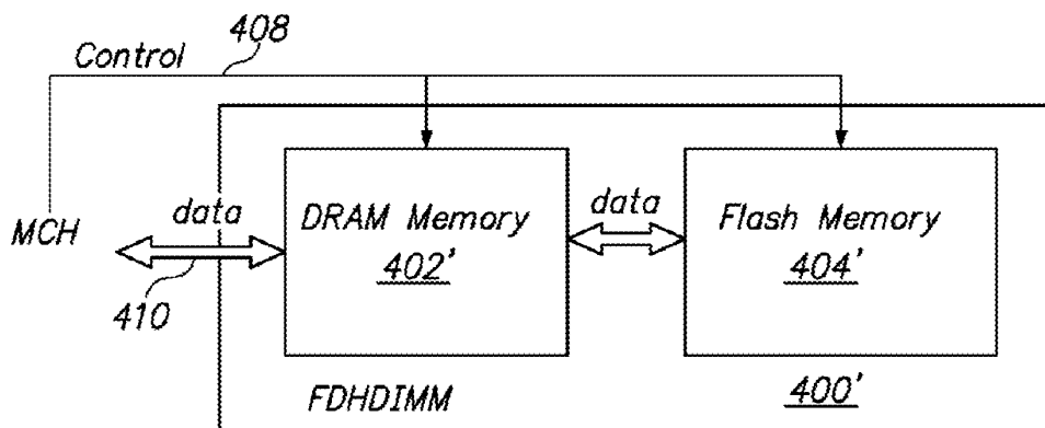
FIG. 2 (PRIOR ART)
