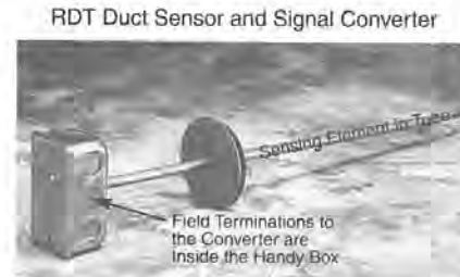
Figure 13.8 RTD Sensor and Signal Converter
