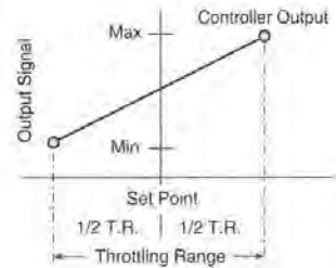
Figure 6.2 Process Throttling Range
