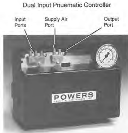
Figure 3.4 Pneumatic Controller
