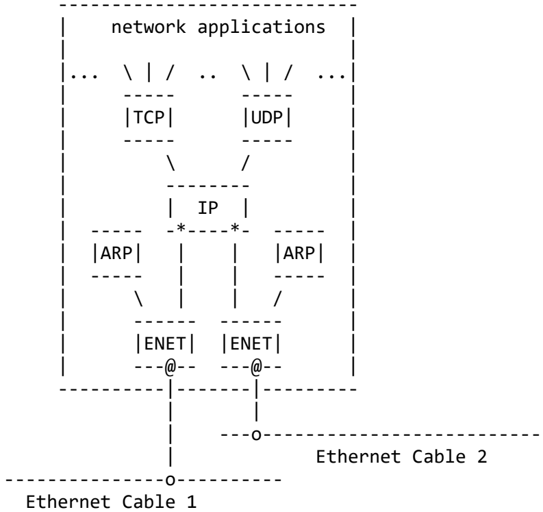
Figure 3. TCP/IP Network Node on 2 Ethernets
