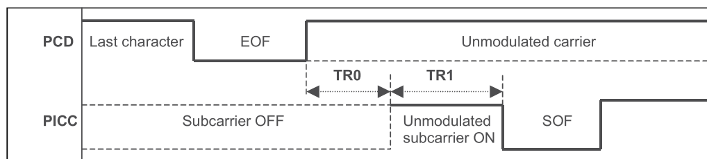
Figure 16 — PICC subcarrier SOF
