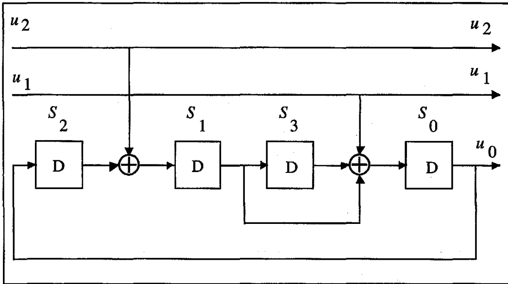
Figure 11 – Finite state machine for Wei's encoder
