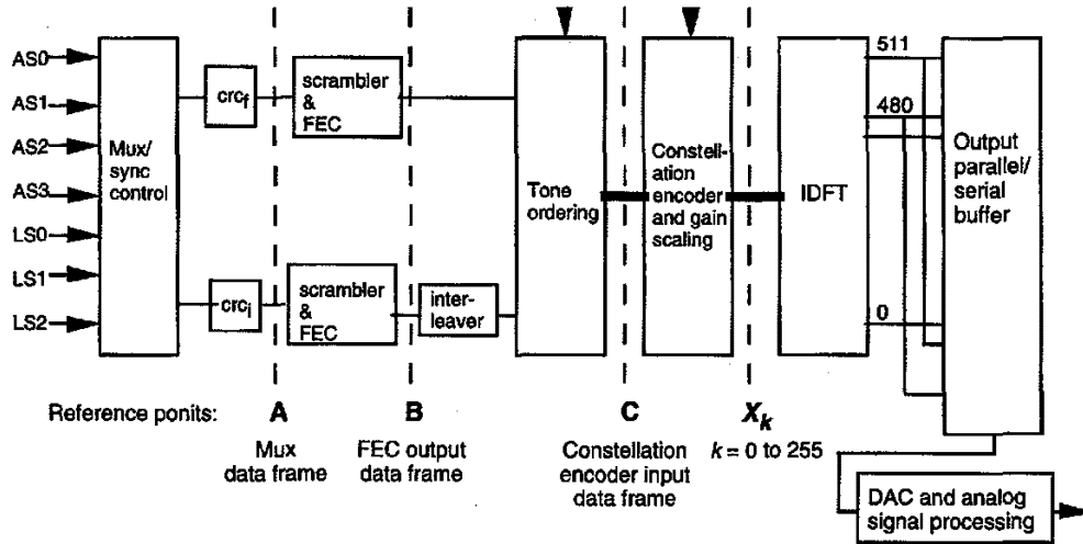
Figure 2 – ATU-C transmitter reference diagram
