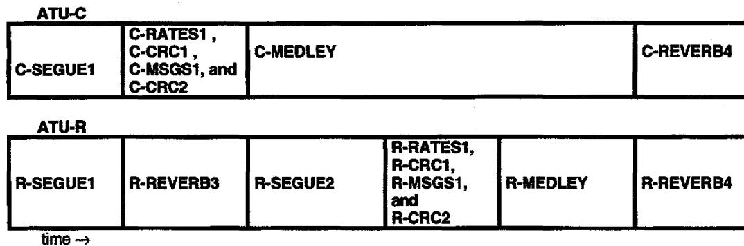
Figure 32 – Timing diagram of channel analysis (12.6-12.7)
