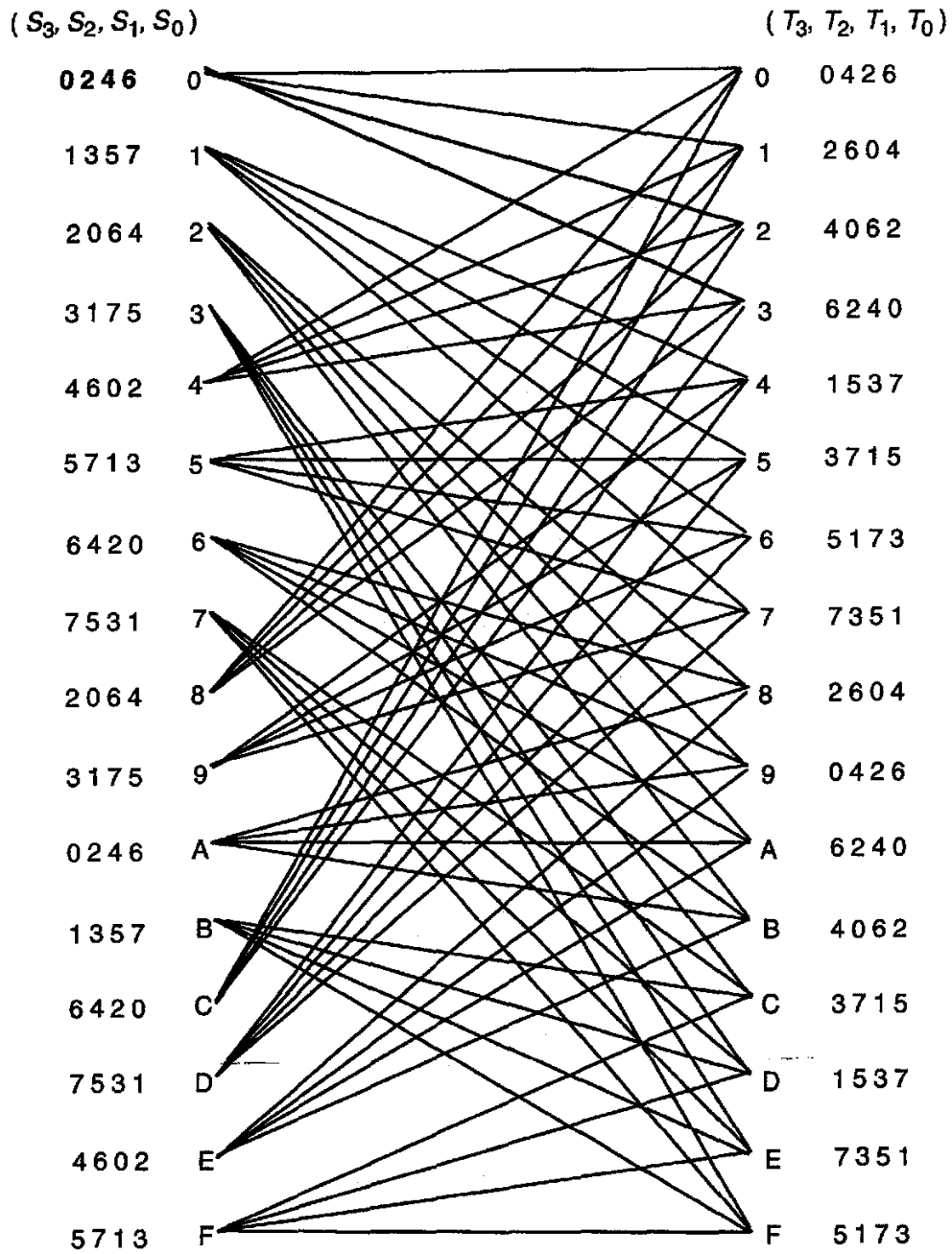
Figure 12 - Trellis diagram
