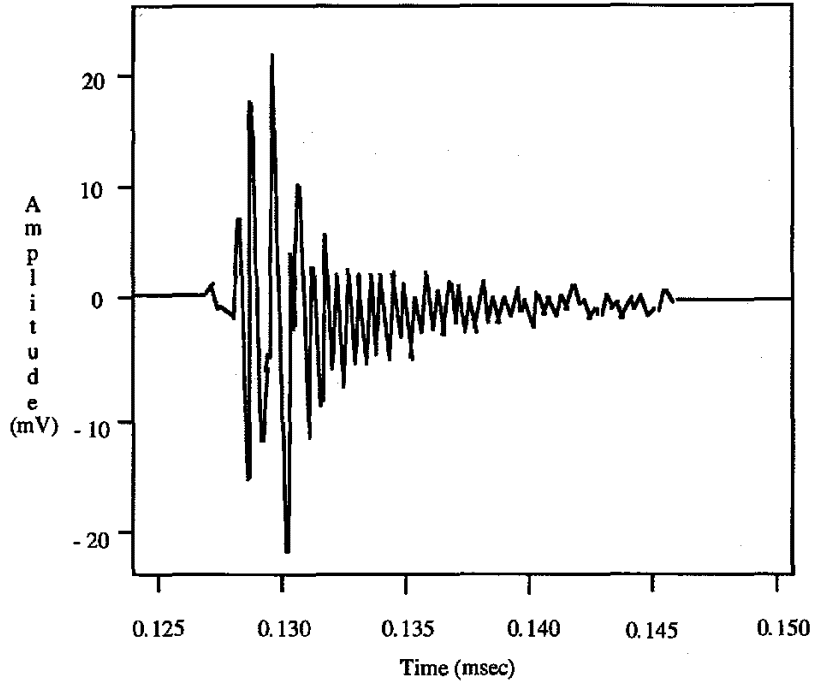
Figure 39 – Test impulse #1
