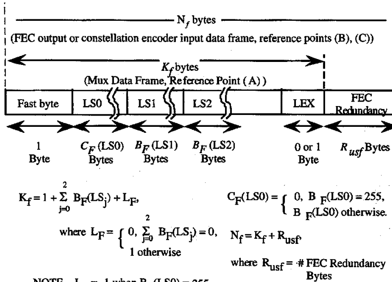
Figure 20 - Fast data buffer - ATU-R transmitter
