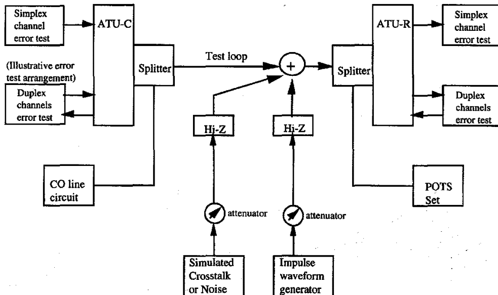
Figure 41 – Laboratory test setup for measuring performance margins
