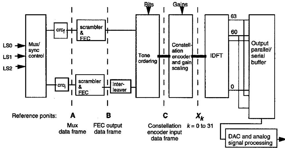
Figure 3 – ATU-R transmitter reference diagram
