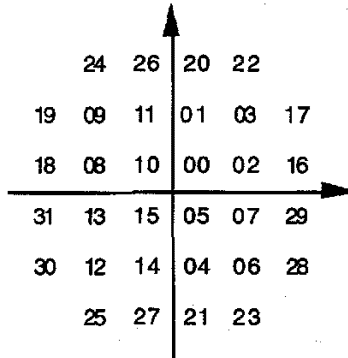
Figure 16 – Constellation labels for b = 5
