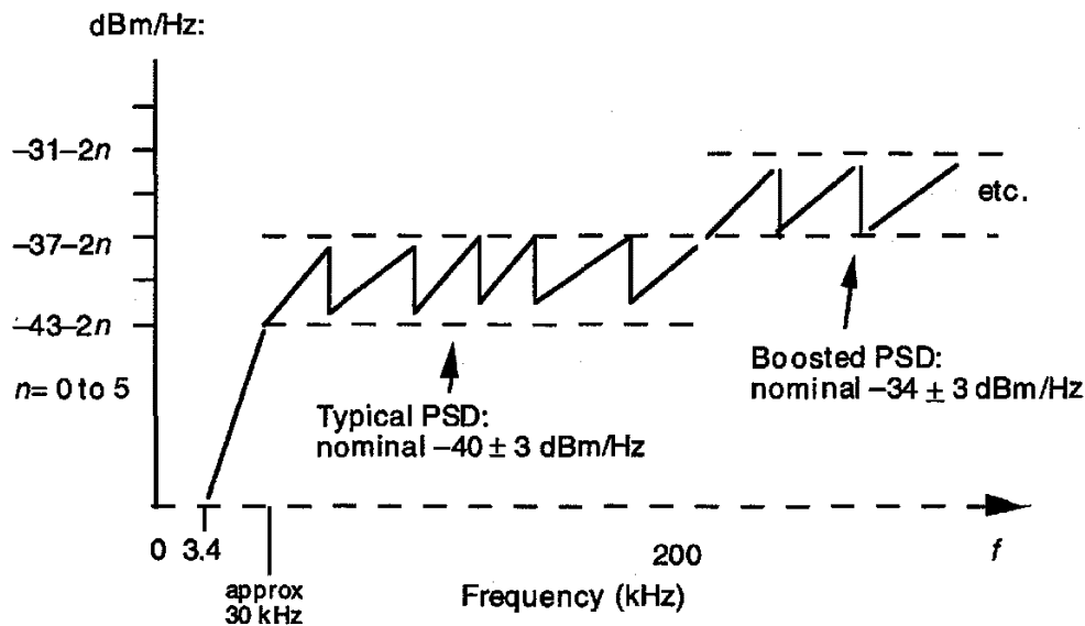
Figure 18 – ATU-C transmitter PSD mask: pass-band detail
