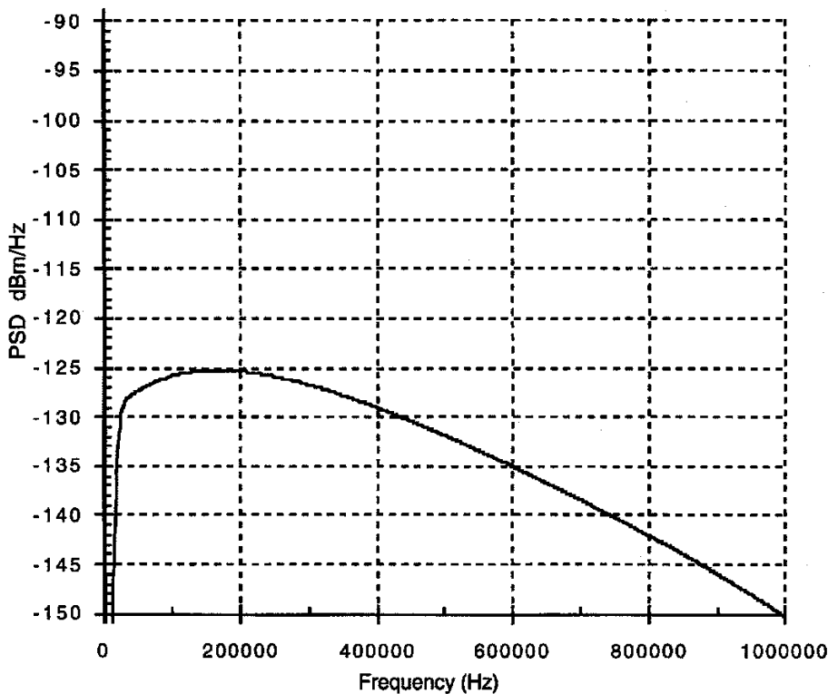
Figure B.4 – Theoretical 10-disturber ADSL FEXT
