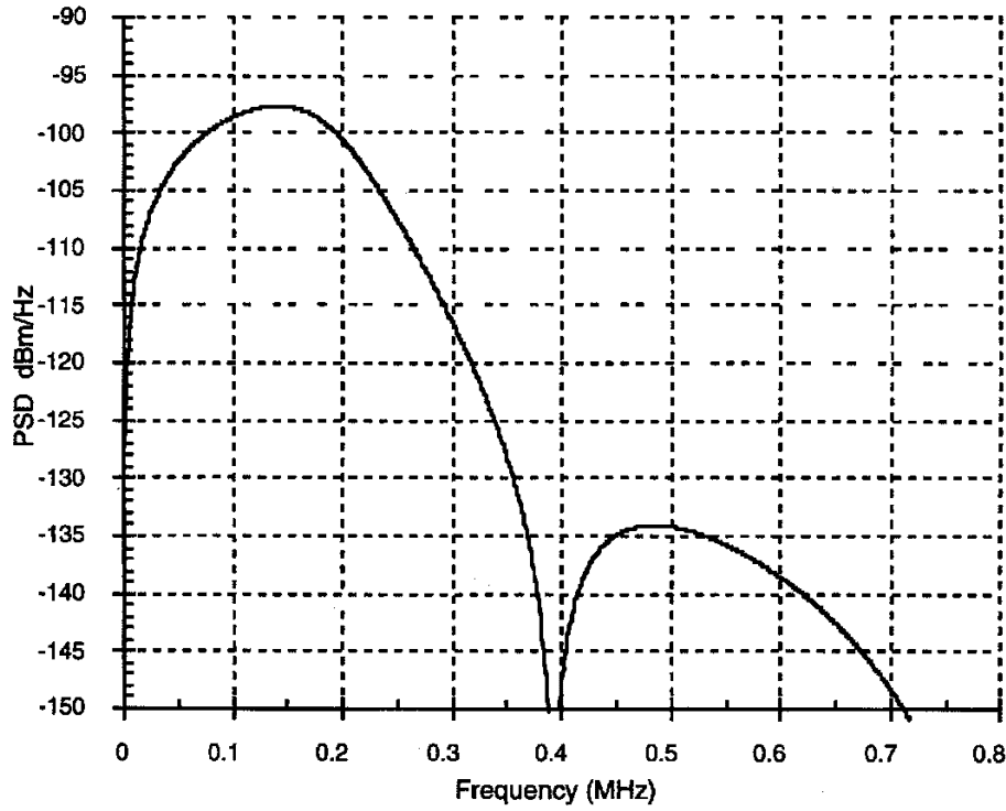
Figure B.2 – 10-disturber HDSL NEXT
