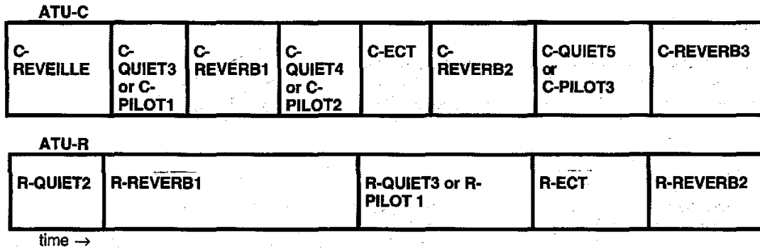
Figure 31 – Timing diagram of transceiver training (12.4-12.5)
