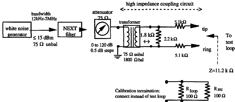
Figure 42 – High impedance crosstalk injection circuit
