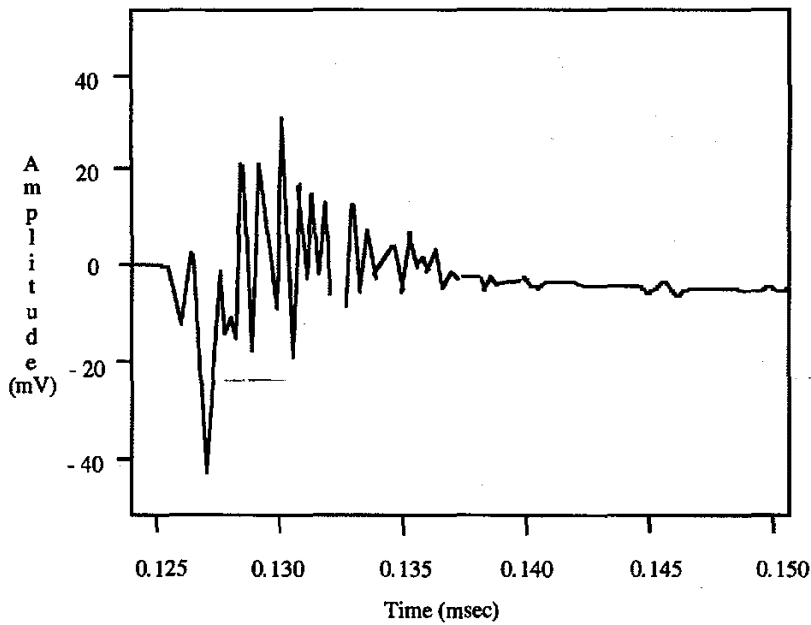
Figure 40 – Test impulse #2
