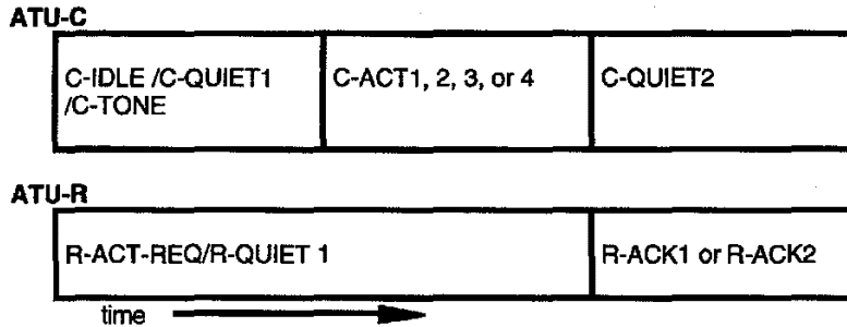
Figure 30 – Timing diagram of activation and acknowledgment (12.2-12.3)
