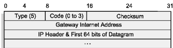
Figure 6.37 ICMP destination unreachable message
