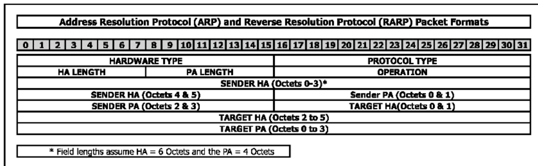
Figure 6.27 ARP header
