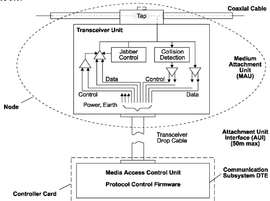
Figure 3.1 10Base5 hardware components
