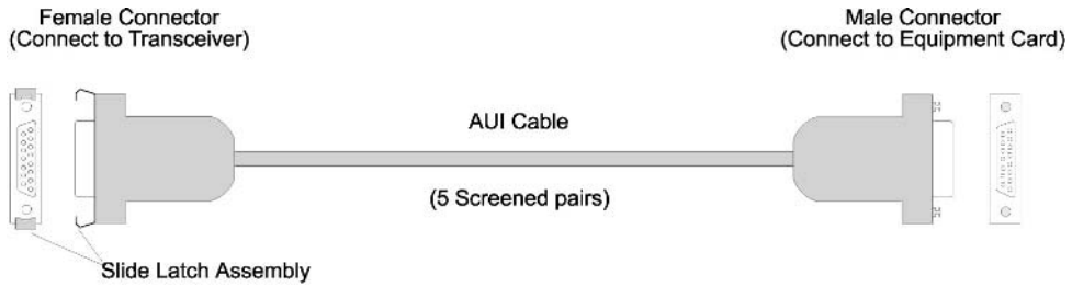
Figure 3.2 AUI cable connectors
