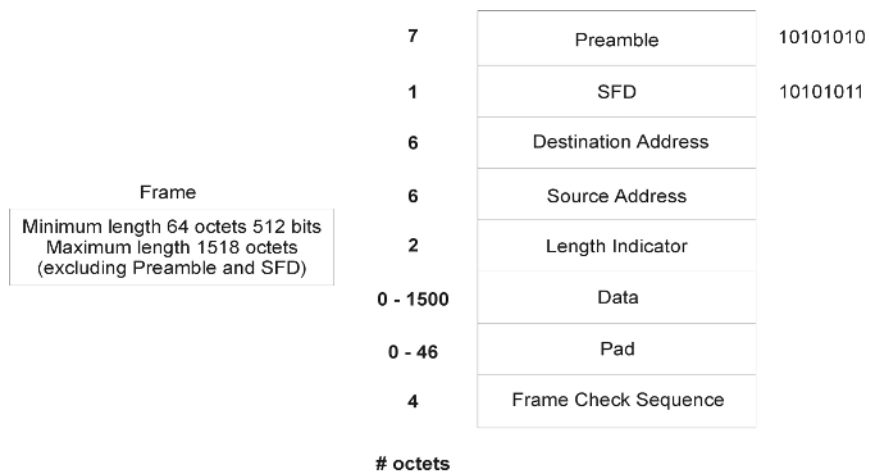
Figure 3.8 MAC frame format
