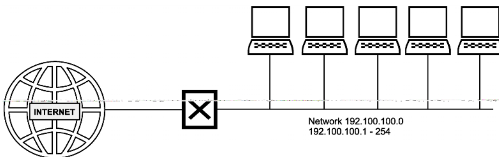
Figure 6.6 Before subnetting
