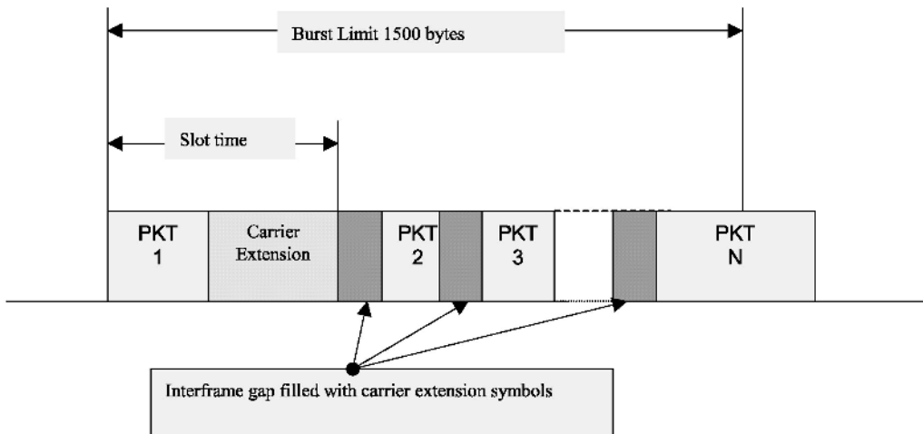
Figure 4.7 Packet bursting
