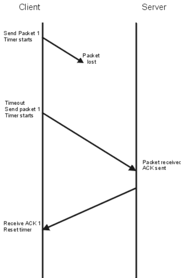
Figure 7.2 Positive acknowledgment philosophy
