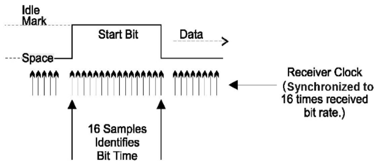
Figure 1.13 Clock estimation at receiver
