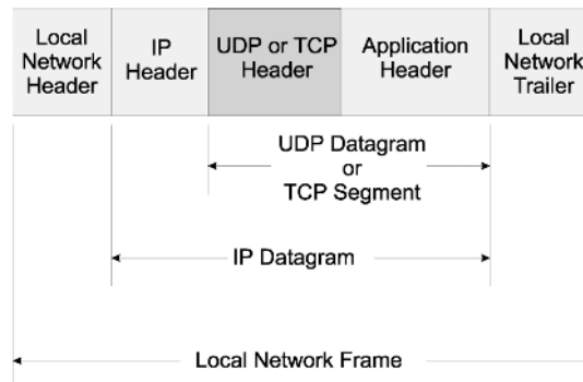
Figure 18.3 Typical structure of Ethernet, TCP/IP and application header
