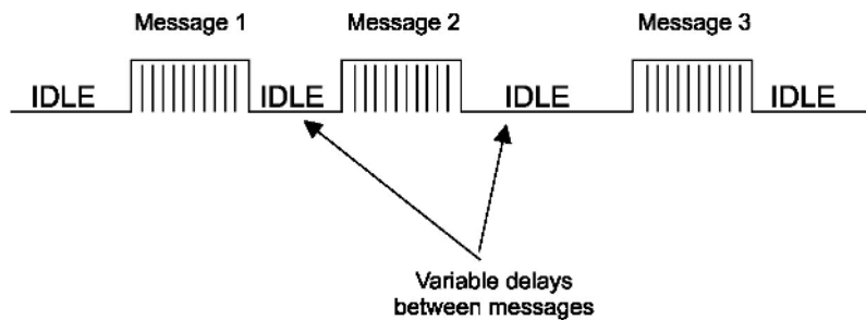
Figure 1.12 Asynchronous data transmission
