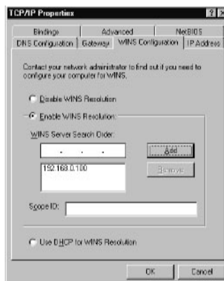
Figure 8.8 WINS Configuration (courtesy of Microsoft Corporation)
