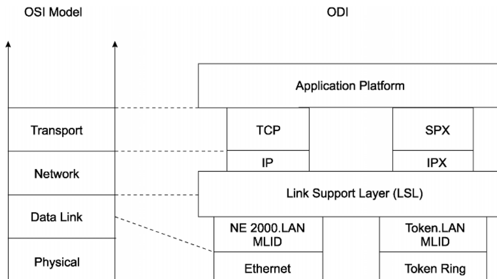
Figure 16.2 ODI architecture
