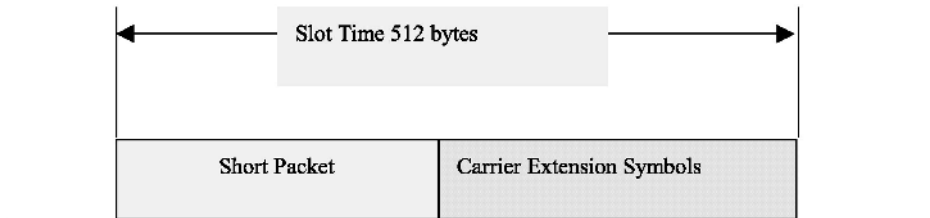
Figure 4.6 Carrier extension
