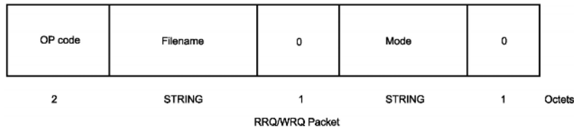
Figure 8.1 RRQ/WRQ frame format
