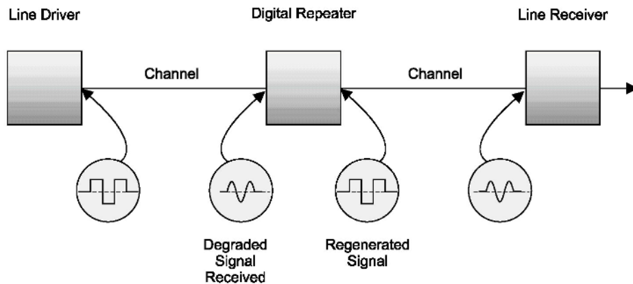
Figure 1.8 Digital link
