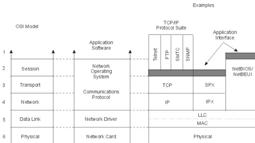
Figure 16.1 Network operating system drivers/protocols
