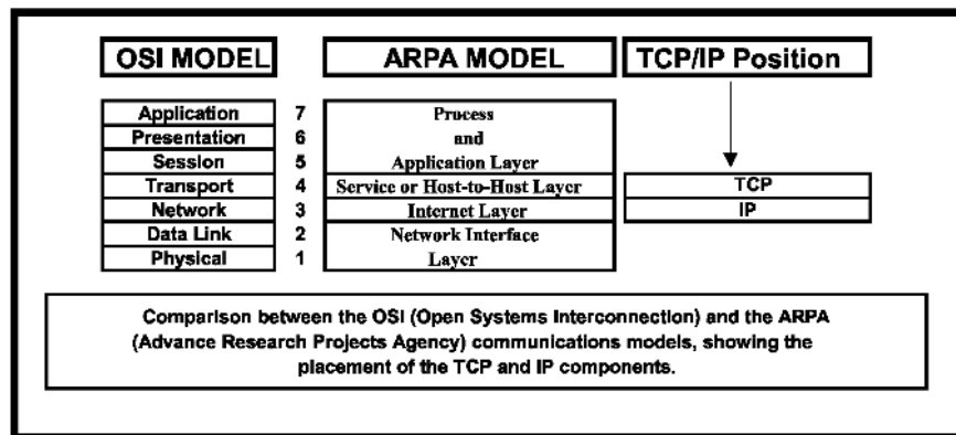
Figure 5.1 OSI vs ARPA models
