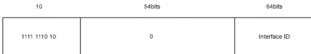
Figure 6.24 Link-local unicast addresses
