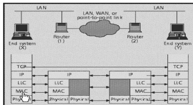
Figure 18.4 Typical protocol stack for TCP/IP (courtesy of Stallings 1997)
