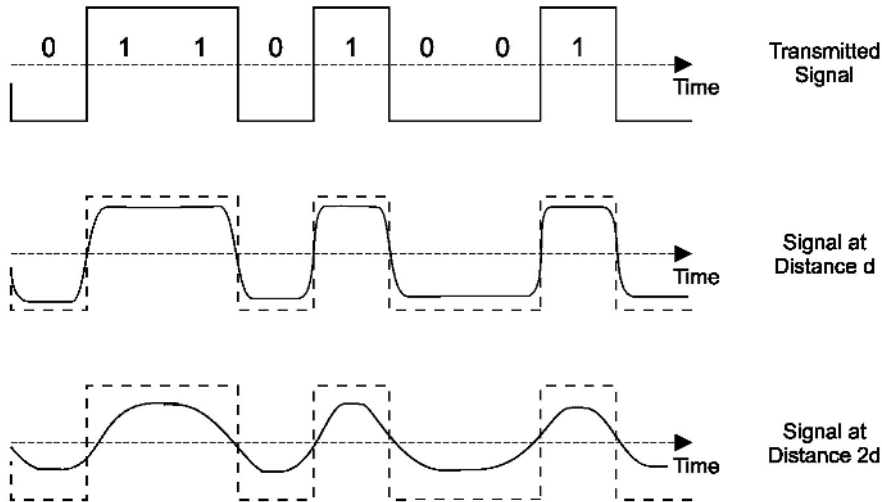
Figure 1.4 Signal attenuation
