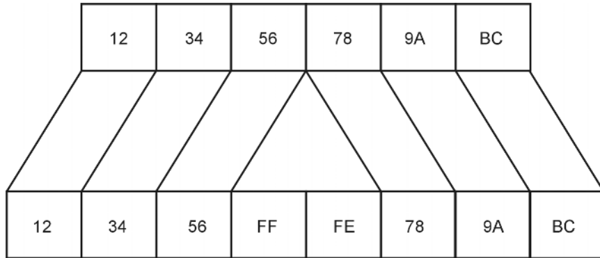
Figure 6.22 Converting a 48-bit MAC address to EUI-64 format
