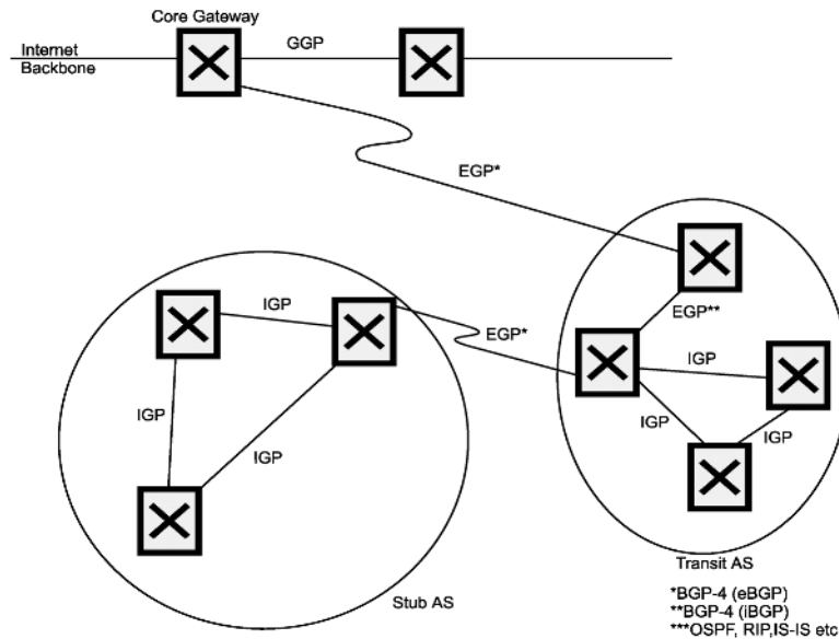
Figure 6.42 Application of routing protocols
