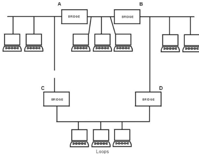
Figure 10.3 Avoidance of loops in bridge networks
