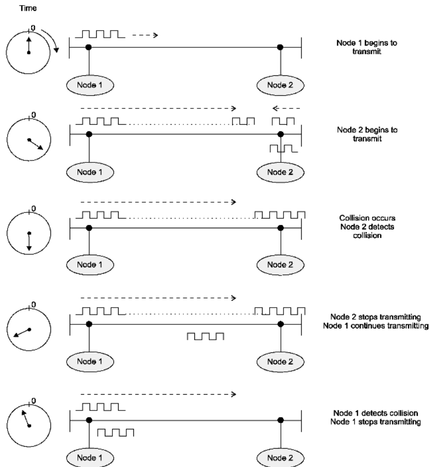
Figure 3.7 CSMA/CD collisions
