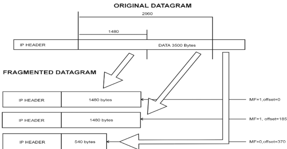
Figure 6.16 IPv4 fragmentation
