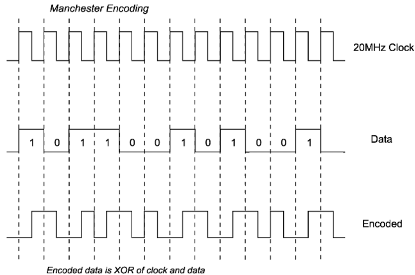
Figure 3.6 Manchester encoding
