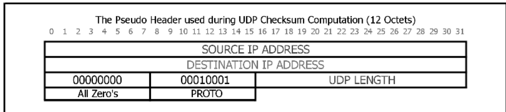
Figure 7.8 UDP pseudo header format
