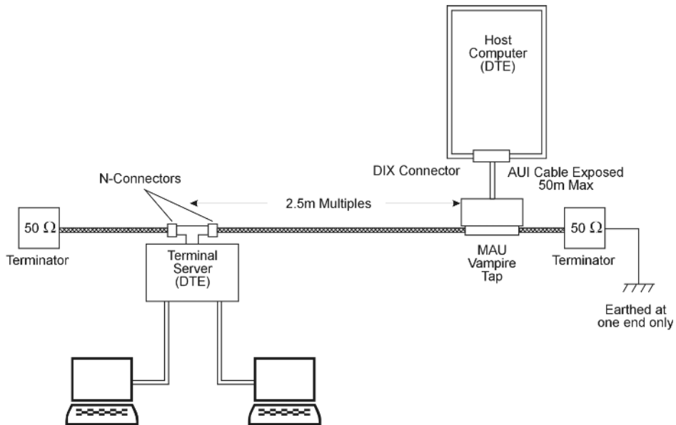
Figure 3.3 10Base5 Ethernet segment
