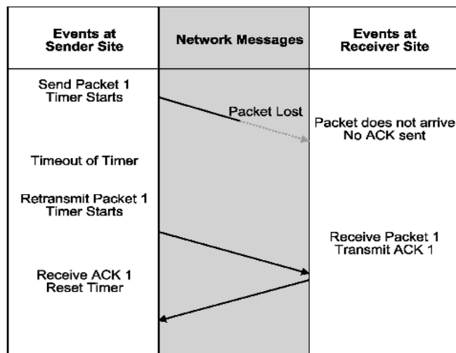
Figure 18.5 Positive acknowledgment philosophy
