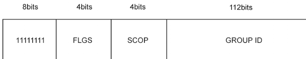
Figure 6.25 Address format: IPv6 multicast
