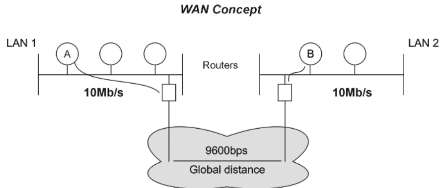
Figure 2.3 WAN concept
