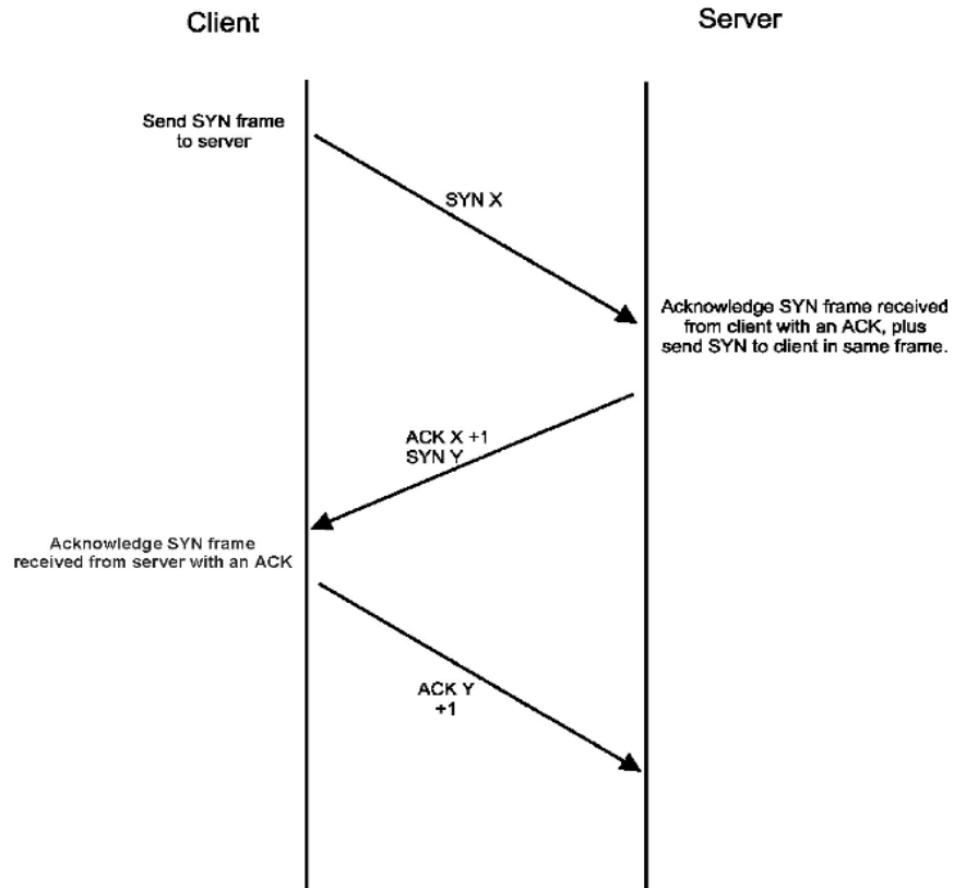
Figure 7.3 TCP connection establishment
