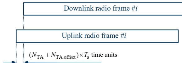
Figure 8.1-1: Uplink-downlink timing relation
