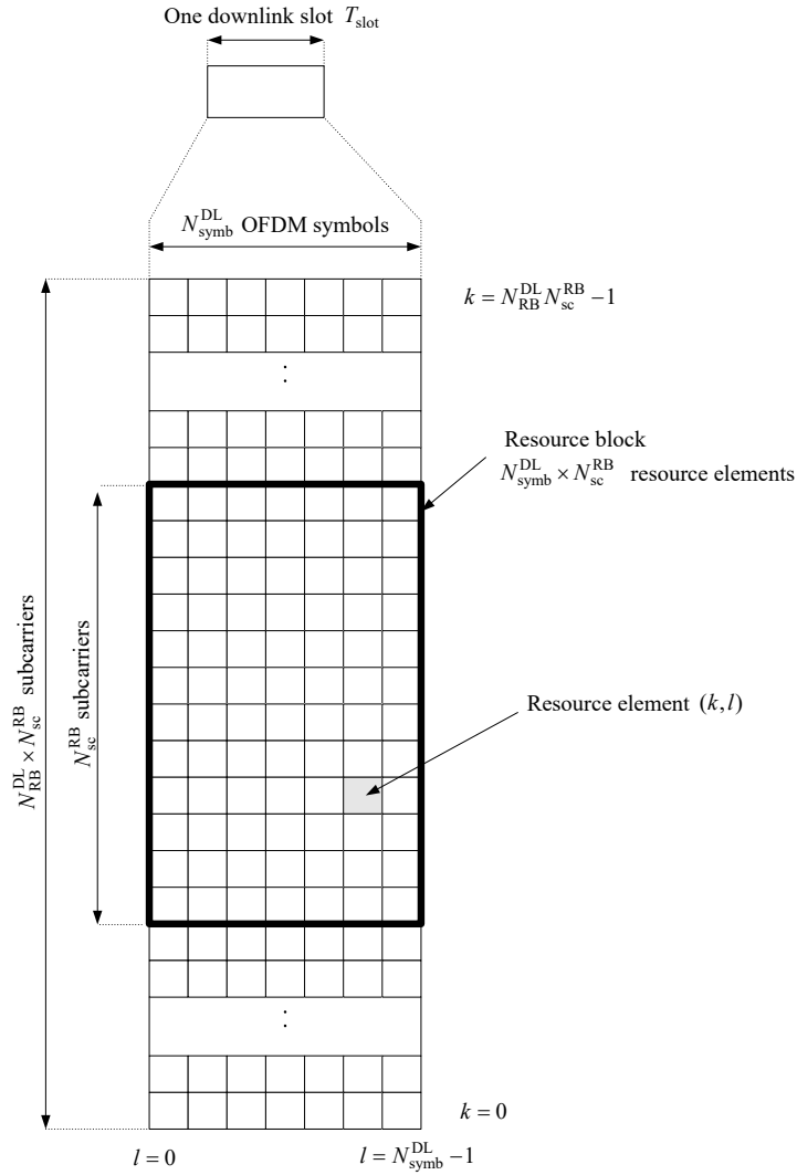
Figure 6.2.2-1: Downlink resource grid.
