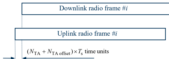
Figure 8.1-1: Uplink-downlink timing relation
