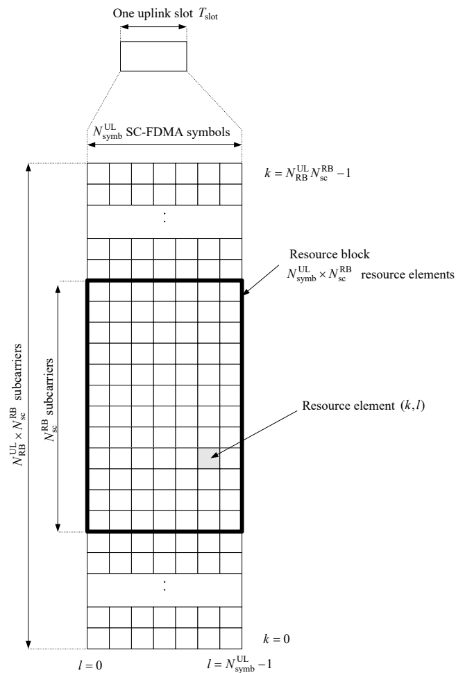
Figure 5.2.1-1: Uplink resource grid.
