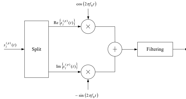
Figure 6.13-1: Downlink modulation.
