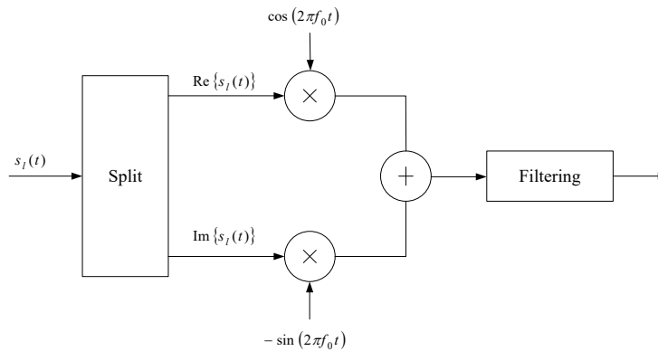
Figure 5.8-1: Uplink modulation.
