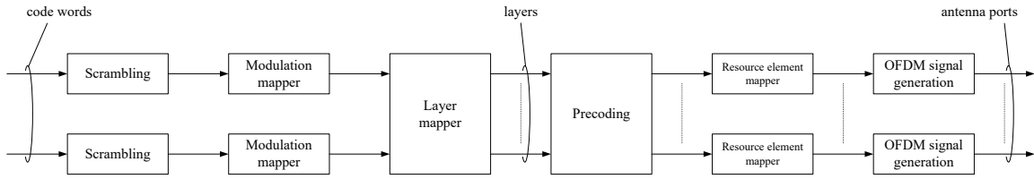
Figure 6.3-1: Overview of physical channel processing.
