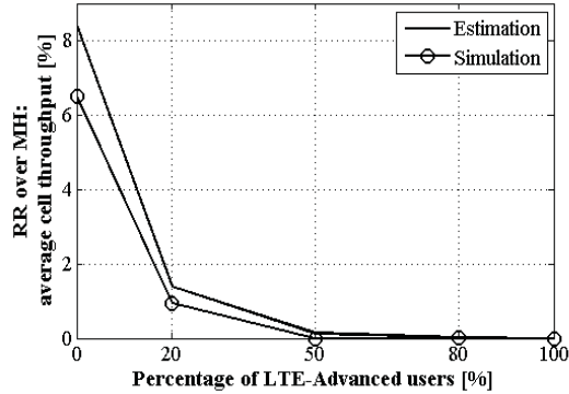
Fig. 3. Gain in average cell throughput by using RR balancing as compared to MH. Performance is evaluated with 10 users per cell and different ratios of LTE-Advanced users. Both estimated and simulated results are shown.
