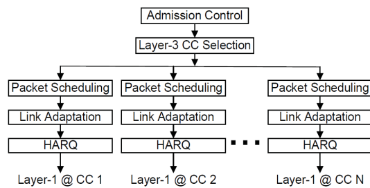
Fig. 1. Structure of a multi-component carrier LTE-Advanced system.
