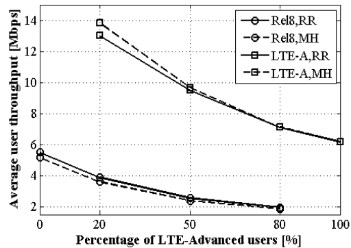
Fig. 4. Average user throughput for the two carrier load balancing methods. Results are obtained via simulation with 10 users per cell and different ratios of LTE-Advanced users.
