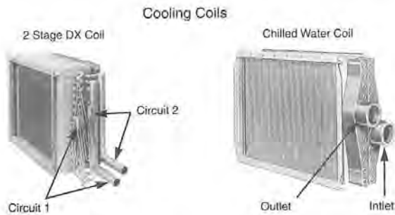
Figure 17.1 Cooling Coils
