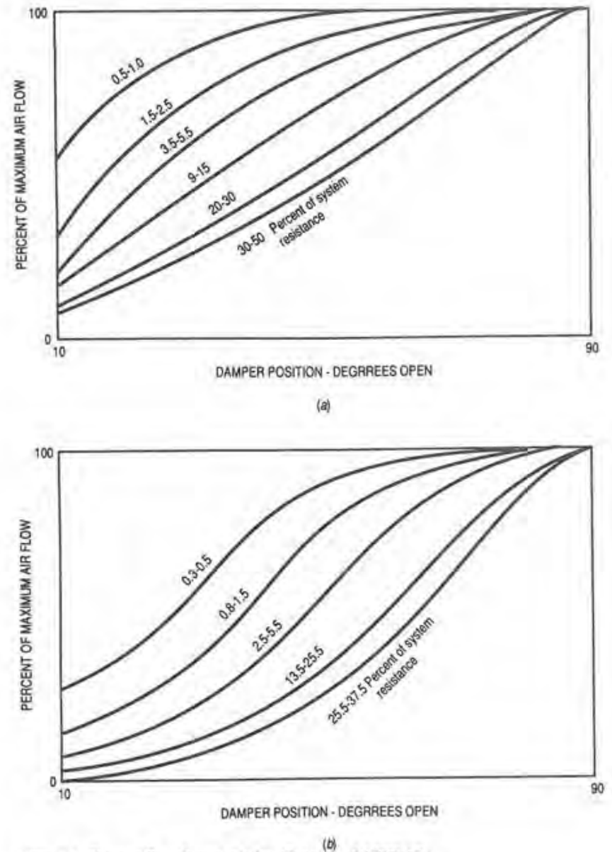
Figure 3.4 Damper flow characteristics. (Courtesy of ASHRAE.)
