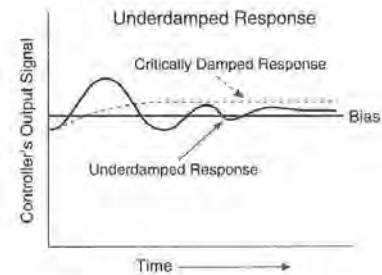
Figure 12.8 Underdamped Response
