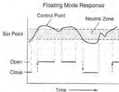
Figure 8.9 Floating Controller Response
