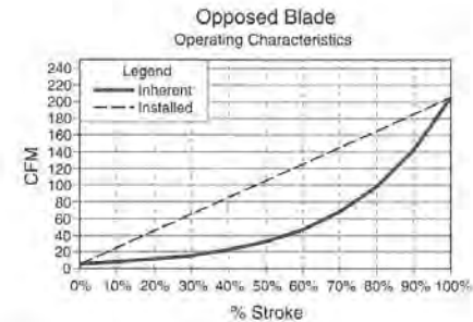
Figure 9.16 Opposed Blade Damper Response
