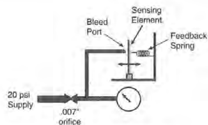
Figure 7.4 Pneumatic Restrictor/Sensor
