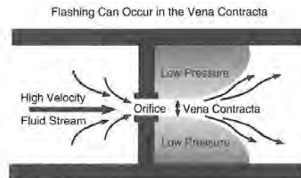
Figure 9.8 The Vena Contracta - Location of the Highest Fluid Velocity and Lowest Static Pressure
