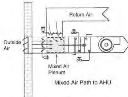
Figure 2.4 Mixed Airstream
