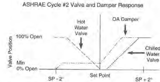
Figure 20.22 Cycle 2 Valve and Damper Response
