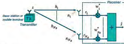
FIGURE 5.2 Channel gains together with linear receive-antenna combination.
