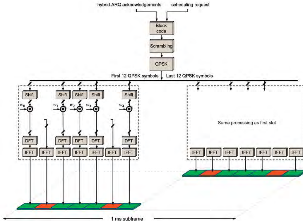
FIGURE 11.28 PUCCH format 3 (normal cyclic prefix).
