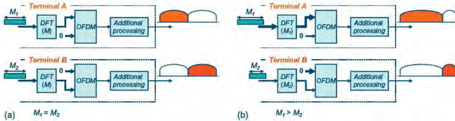
FIGURE 4.12 Uplink user multiplexing in case of DFTS-OFDM. (a) Equal-bandwidth assignment. (b) Unequal-bandwidth assignment.
