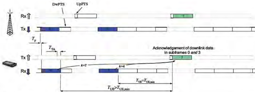
FIGURE 12.7 Example of timing relation between downlink data and uplink hybrid-ARQ acknowledgement for TDD (configuration 2).
