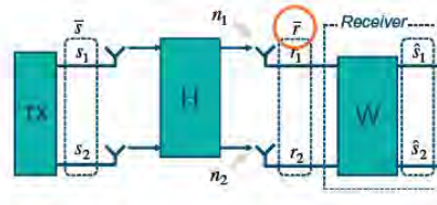
FIGURE 5.15 Linear reception/demodulation of spatially multiplexed signals.
