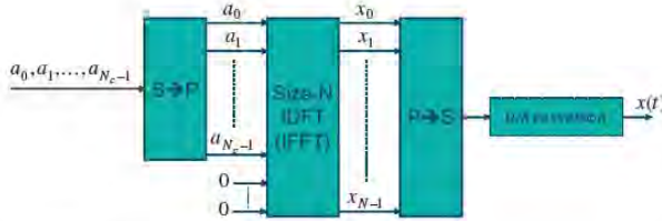
FIGURE 3.6 OFDM modulation by means of IFFT processing.
