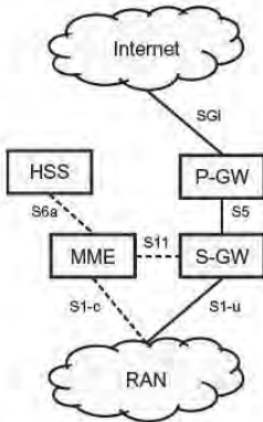
FIGURE 8.1 Core-network (EPC) architecture.
