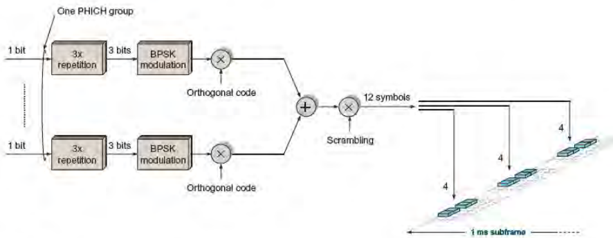
FIGURE 10.24 PHICH structure.
