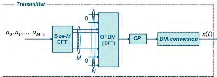
FIGURE 4.8 DFTS-OFDM signal generation.
