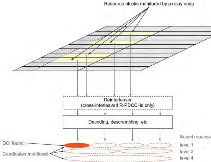
FIGURE 16.9 Illustration of the principle of R-PDCCH monitoring.
