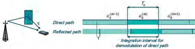
FIGURE 3.8 Time dispersion and corresponding received-signal timing.
