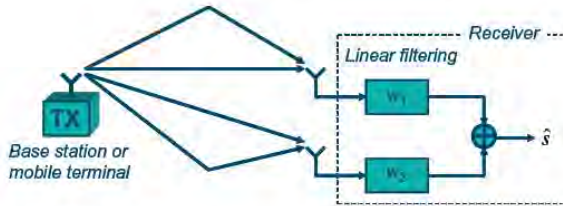
FIGURE 5.5 Two-dimensional space-time linear processing (two receive antennas).
