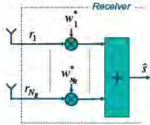
FIGURE 5.1 Linear receive-antenna combination.
