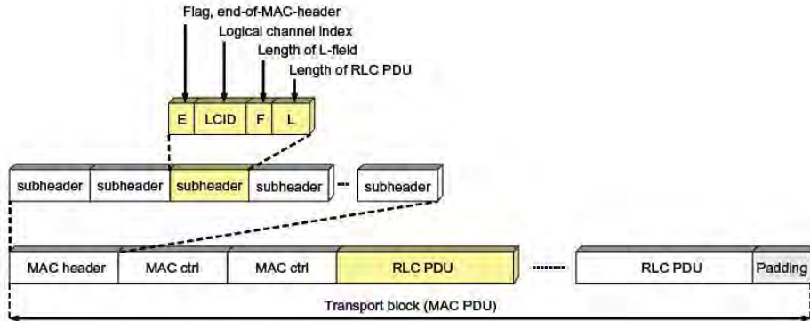
FIGURE 8.9 MAC header and SDU multiplexing.
