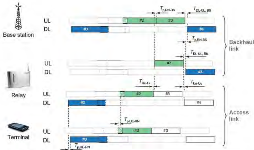
FIGURE 16.12 Example of uplink timing relation for TDD.
