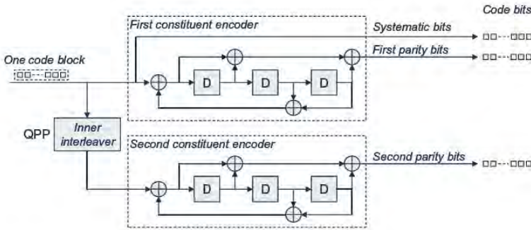
FIGURE 10.3 LTE Turbo encoder.
