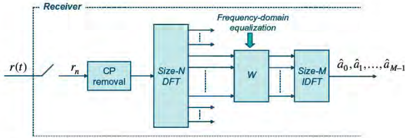
FIGURE 4.11 DFTS-OFDM demodulator with frequency-domain equalization.
