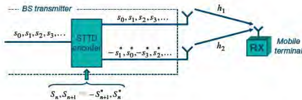
FIGURE 5.9 Space-Time Transmit Diversity (STTD).
