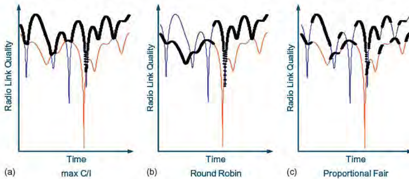
FIGURE 6.3 Examples of three different scheduling behaviors for two users with different average channel quality: (a) max-C/I; (b) round robin; (c) proportional fair. The selected user is shown with bold lines.
