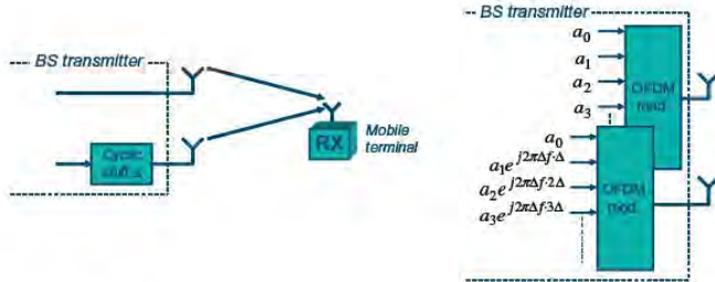
FIGURE 5.8 Two-antenna Cyclic-Delay Diversity (CDD).
