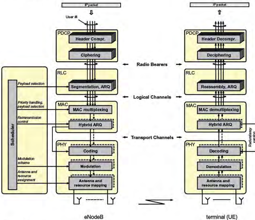
FIGURE 8.4 LTE protocol architecture (downlink).
