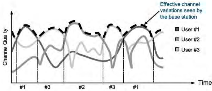
FIGURE 6.2 Channel-dependent scheduling.
