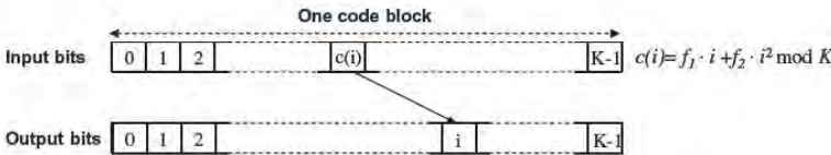
FIGURE 10.4 Principles of QPP-based interleaving.
