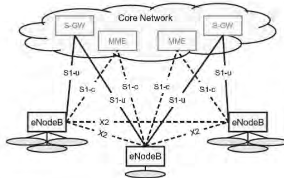
FIGURE 8.2 Radio-access-network interfaces.
