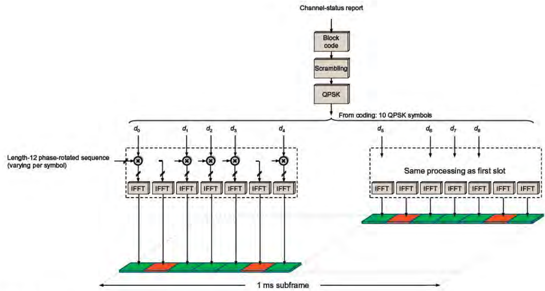
FIGURE 11.27 PUCCH format 2 (normal cyclic prefix).
