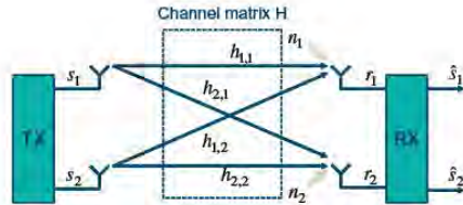
FIGURE 5.14 2 × 2 antenna configuration.
