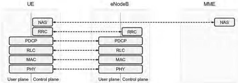
FIGURE 8.3 Overall RAN protocol architecture.
