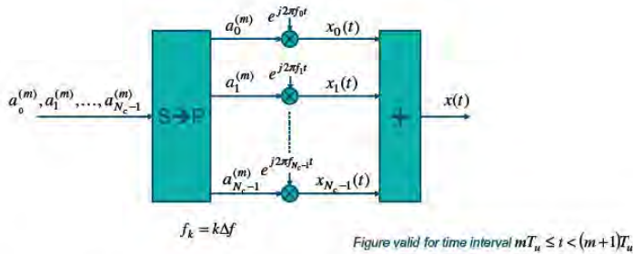
FIGURE 3.3 Principles for OFDM modulation.
