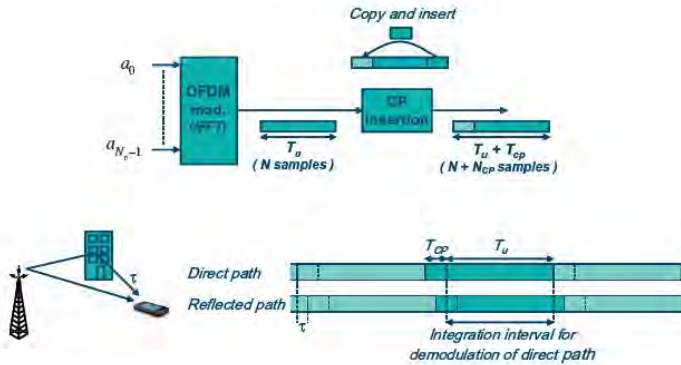
FIGURE 3.9 Cyclic-prefix insertion.
