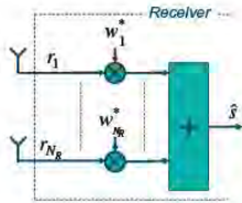
FIGURE 5.1 Linear receive-antenna combination.
