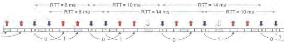
FIGURE 16.6 Example of hybrid-ARQ process numbering for FDD.
